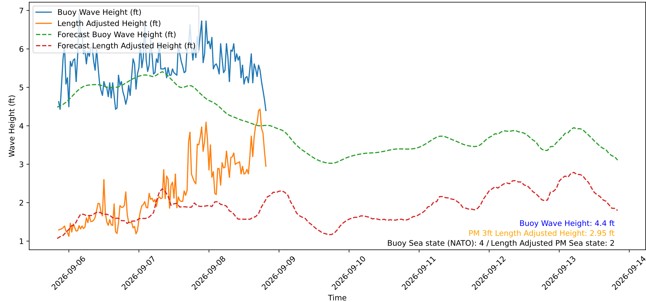
Wave Heights over Time for Red Beach at 2026-09-08 20:20:50
