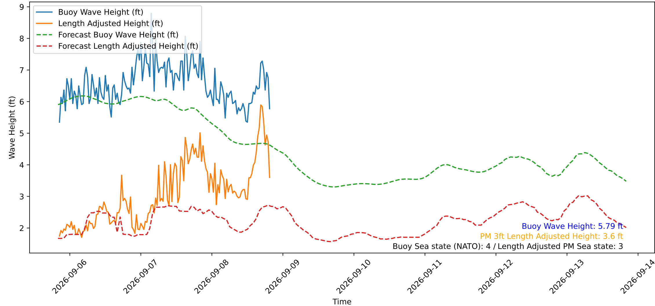
Wave Heights over Time for Green Beach at 2026-09-08 20:21:15
