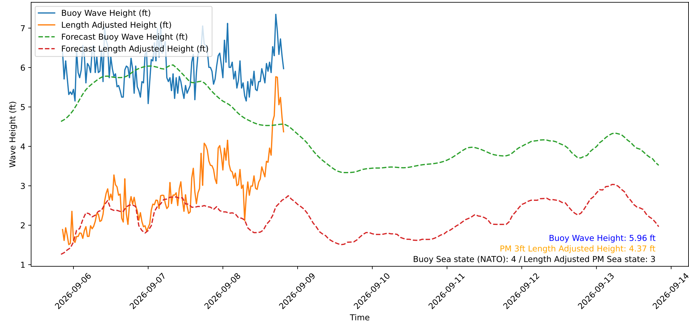
Wave Heights over Time for Oceanside Harbor at 2026-09-08 20:20:29
