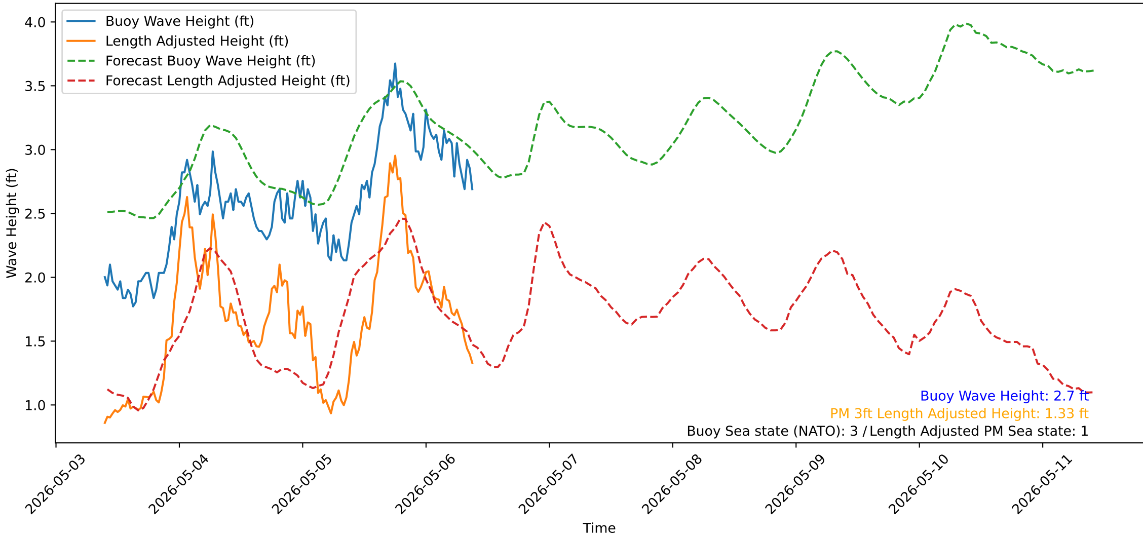
Wave Heights over Time for Green Beach at 2026-05-06 09:41:13
