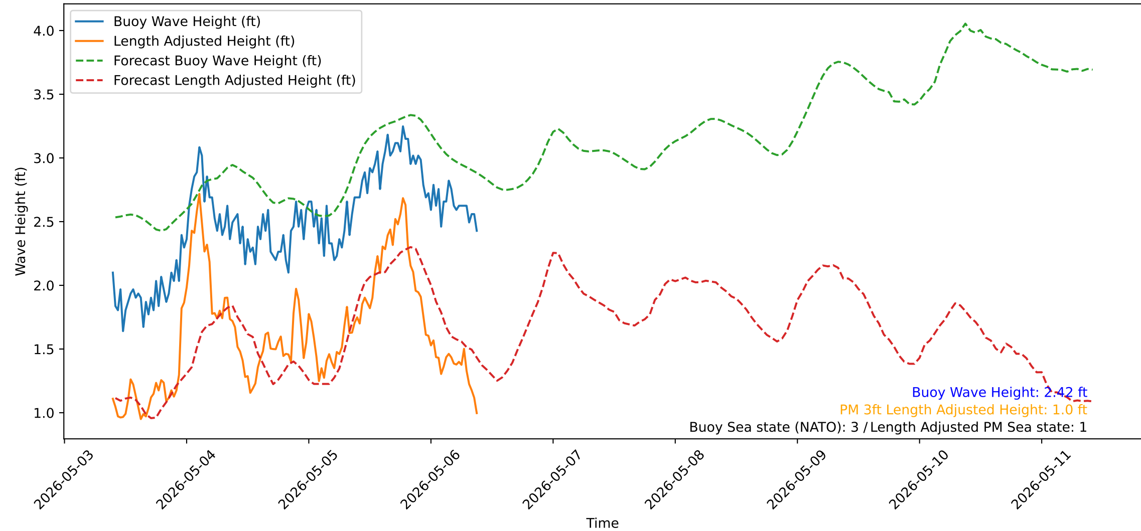
Wave Heights over Time for Oceanside Harbor at 2026-05-06 09:40:31
