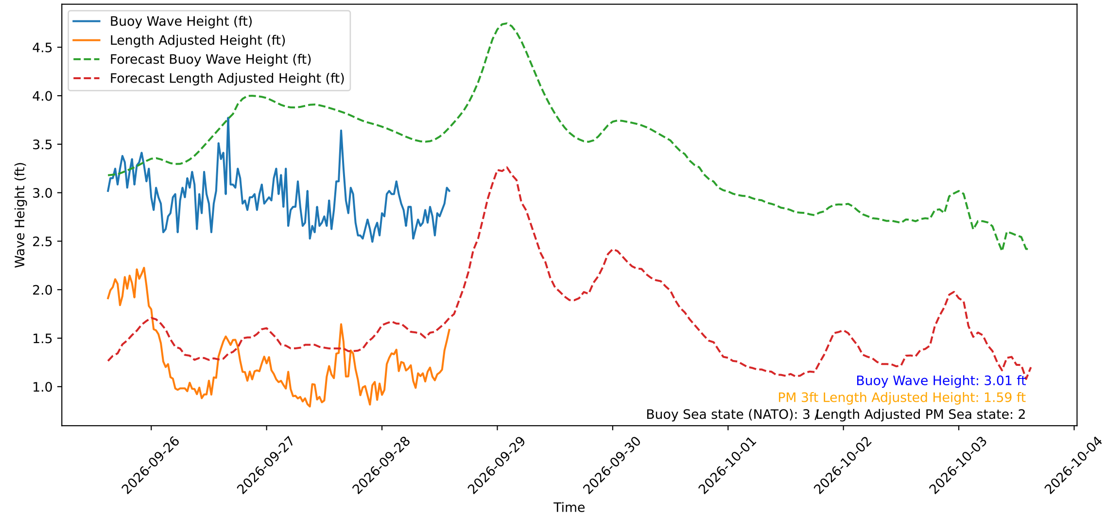
Wave Heights over Time for Oceanside Harbor at 2026-09-28 14:50:29
