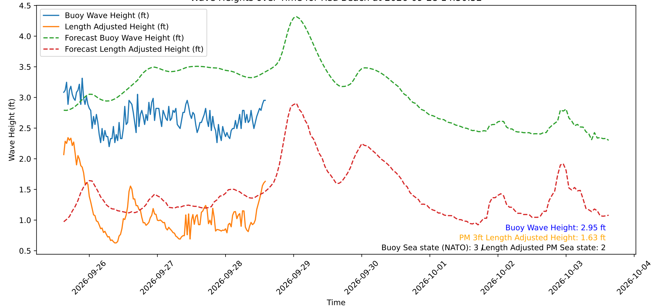
Wave Heights over Time for Red Beach at 2026-09-28 14:50:52
