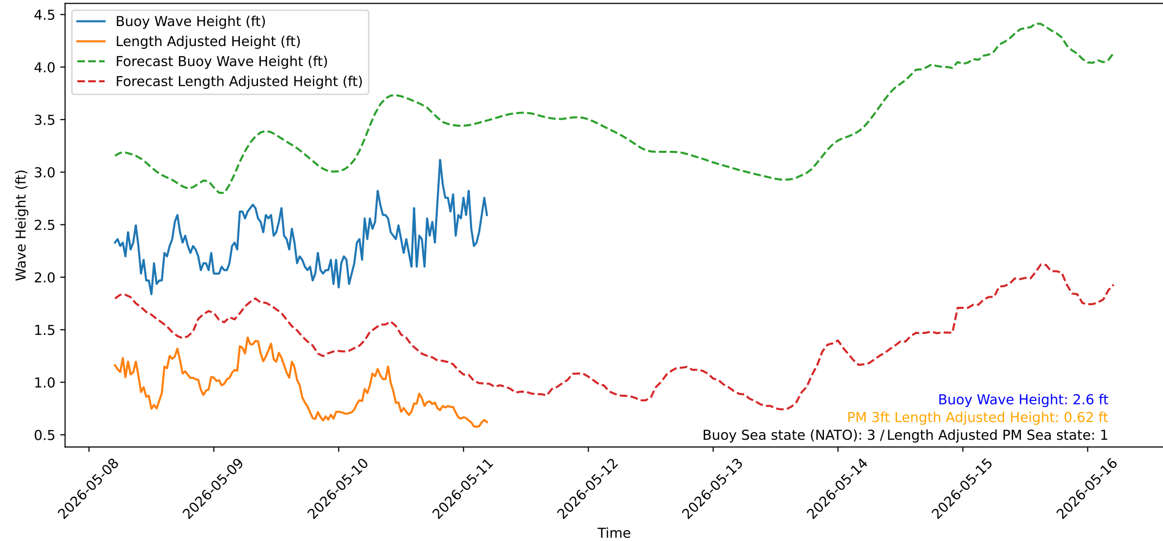
Wave Heights over Time for Green Beach at 2026-05-11 05:11:12
