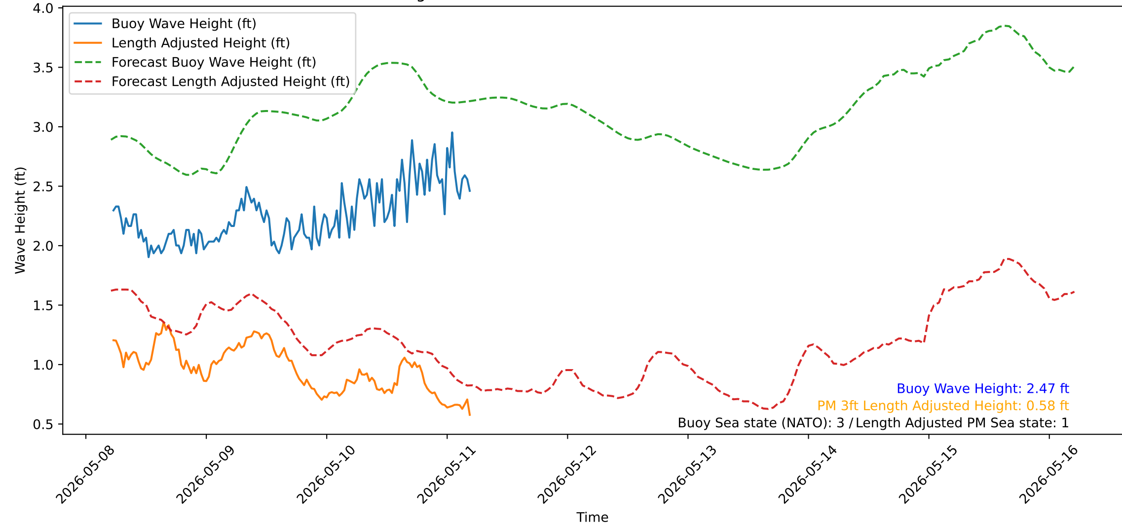
Wave Heights over Time for Red Beach at 2026-05-11 05:10:50
