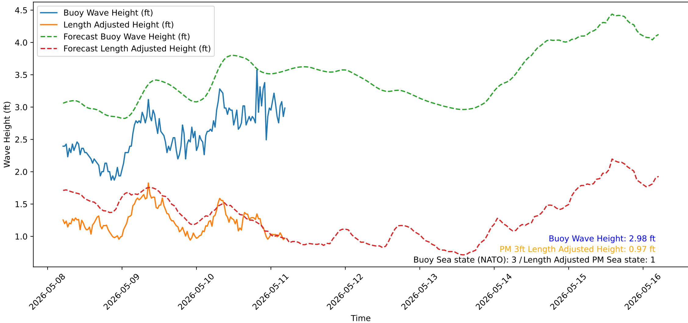
Wave Heights over Time for Oceanside Harbor at 2026-05-11 05:10:30
