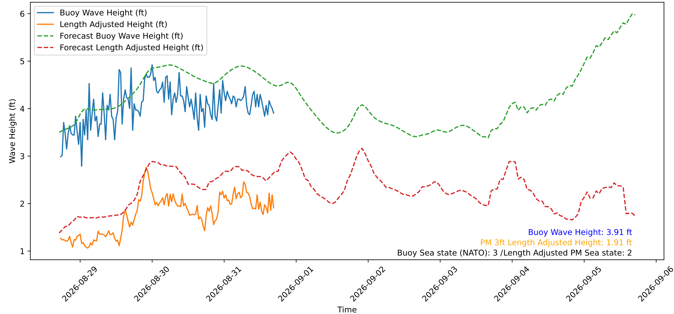
Wave Heights over Time for Green Beach at 2026-08-31 17:21:15
