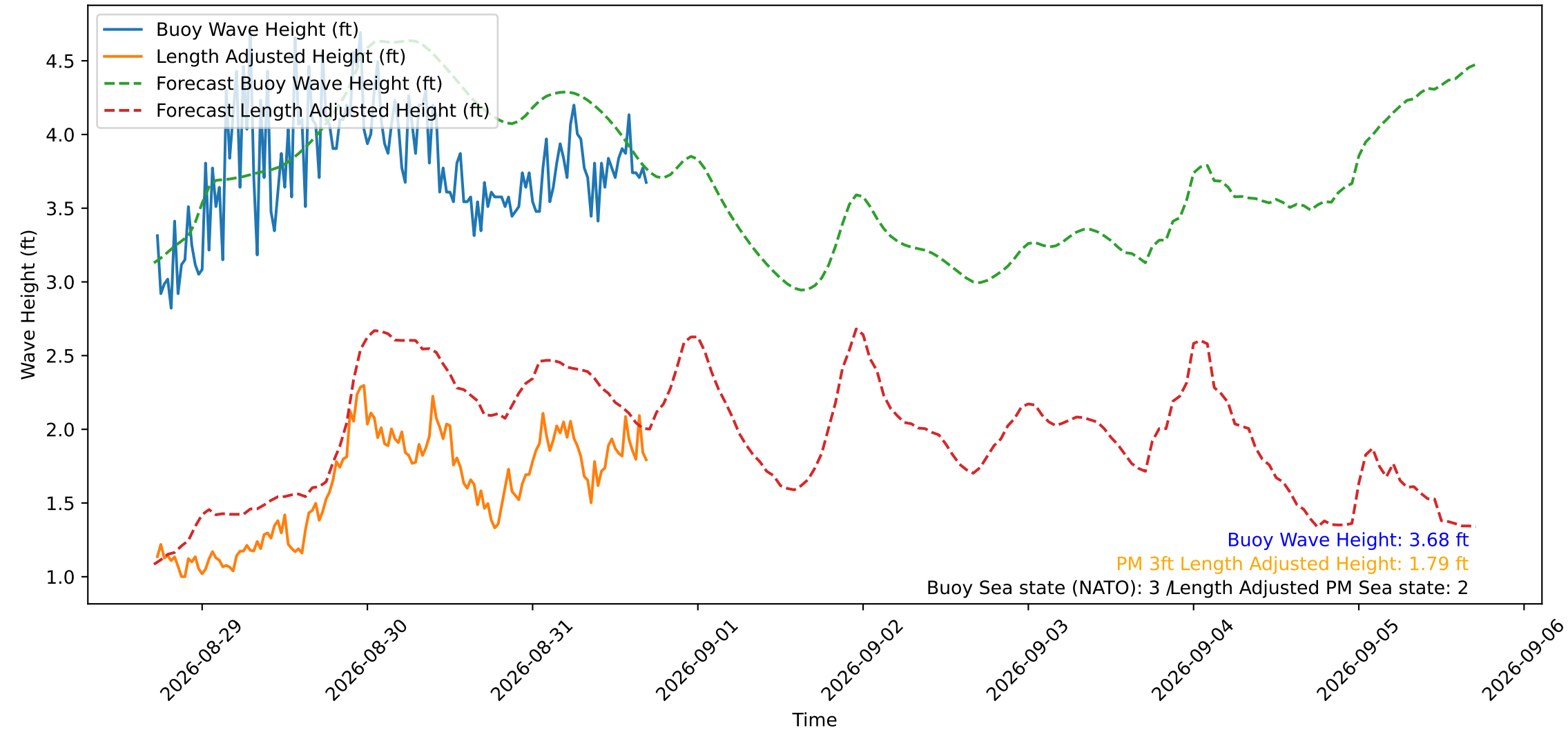
Wave Heights over Time for Red Beach at 2026-08-31 17:20:51
