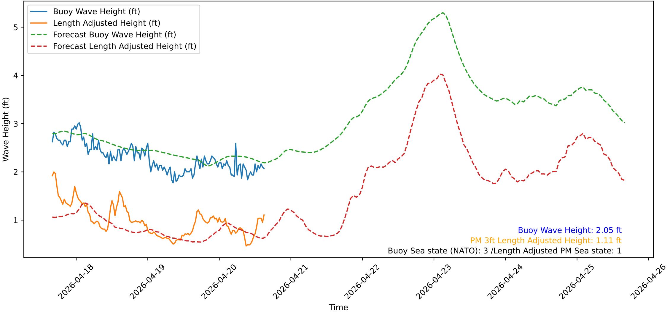
Wave Heights over Time for Red Beach at 2026-04-20 15:40:50
