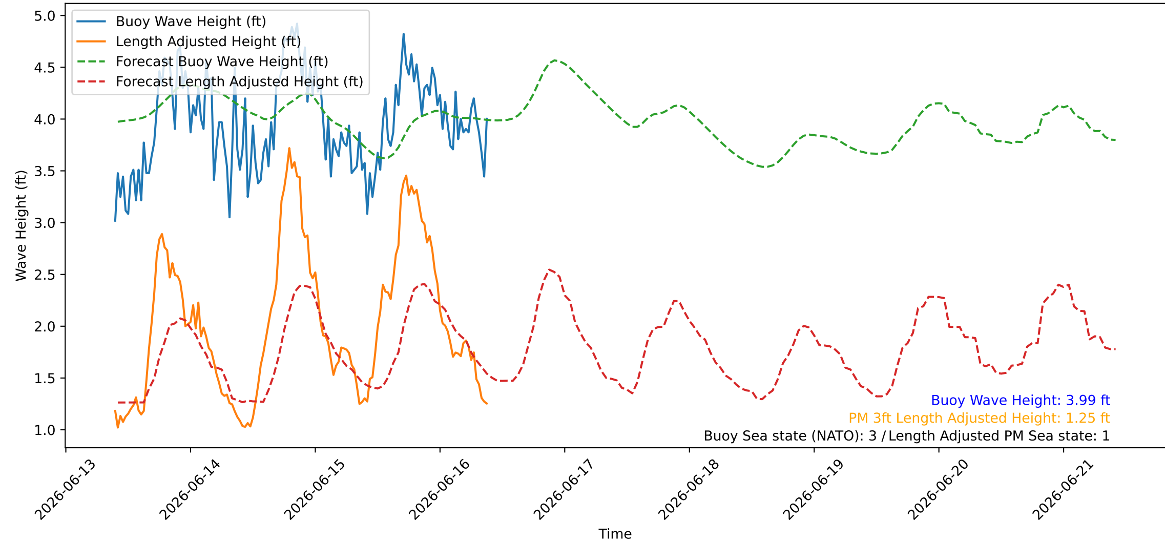
Wave Heights over Time for Green Beach at 2026-06-16 09:41:08
