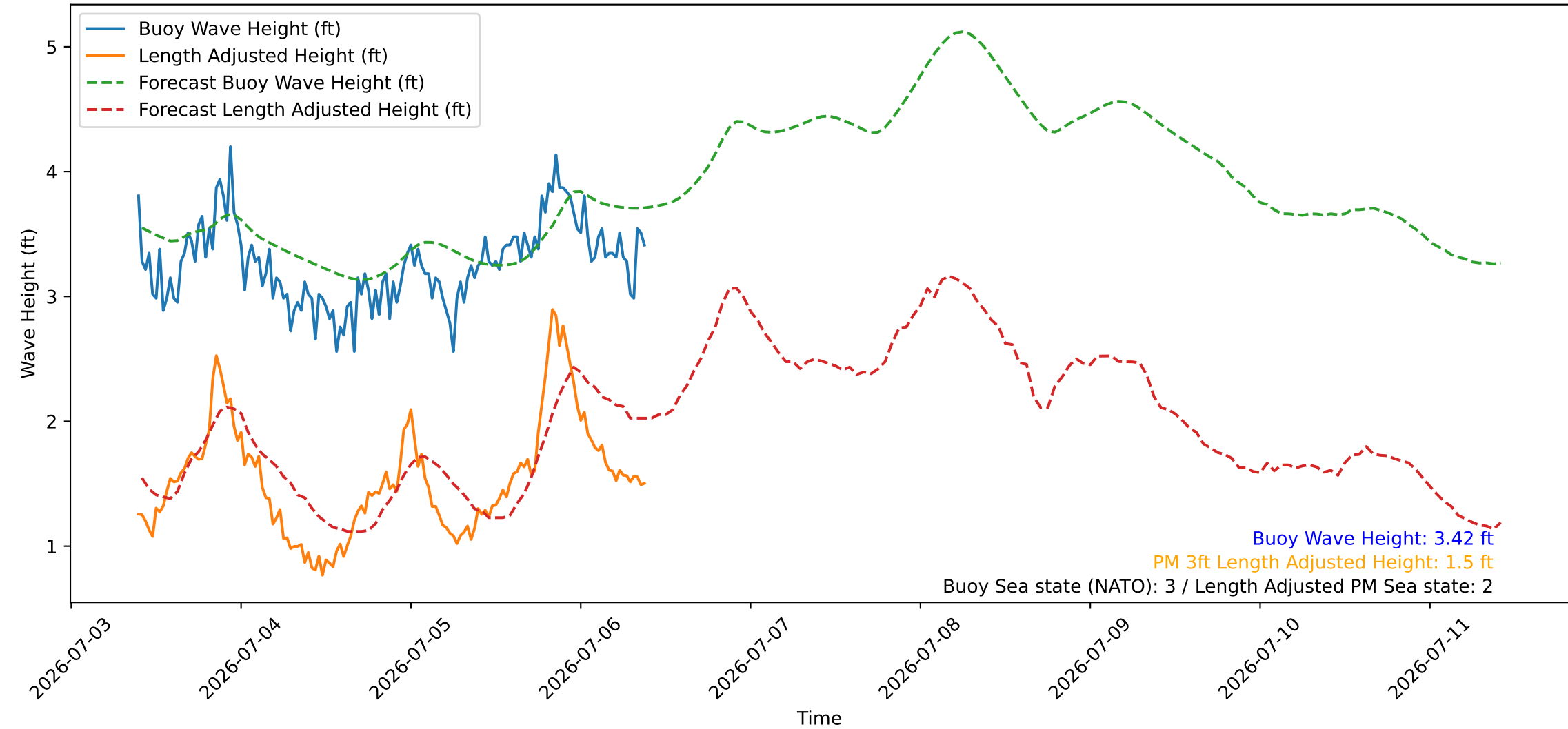
Wave Heights over Time for Green Beach at 2026-07-06 09:41:10
