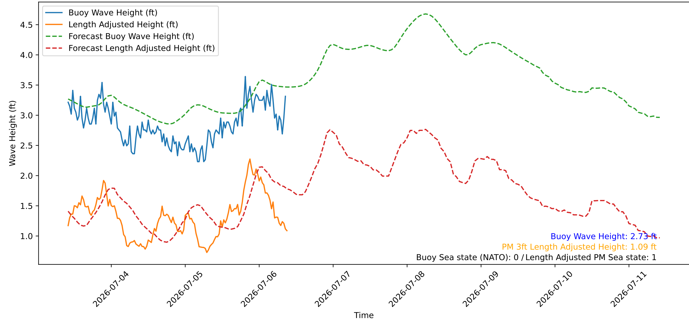
Wave Heights over Time for Red Beach at 2026-07-06 09:40:47
