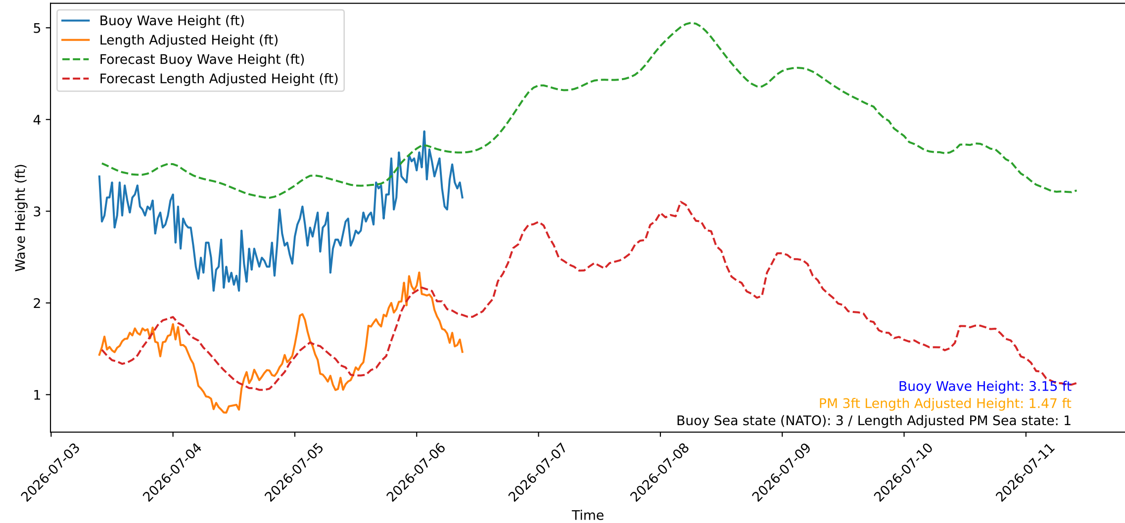
Wave Heights over Time for Oceanside Harbor at 2026-07-06 09:40:27
