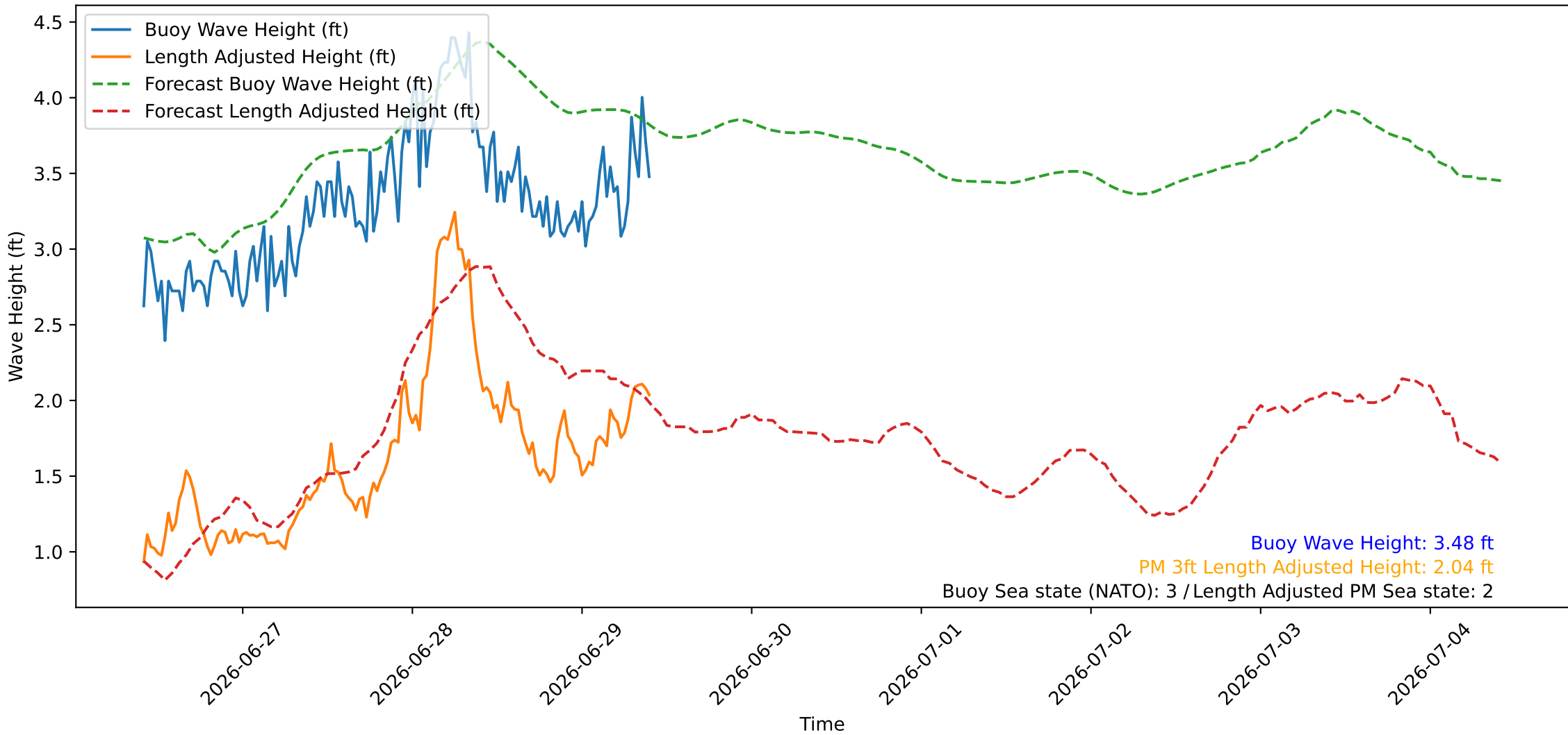
Wave Heights over Time for Oceanside Harbor at 2026-06-29 10:10:25
