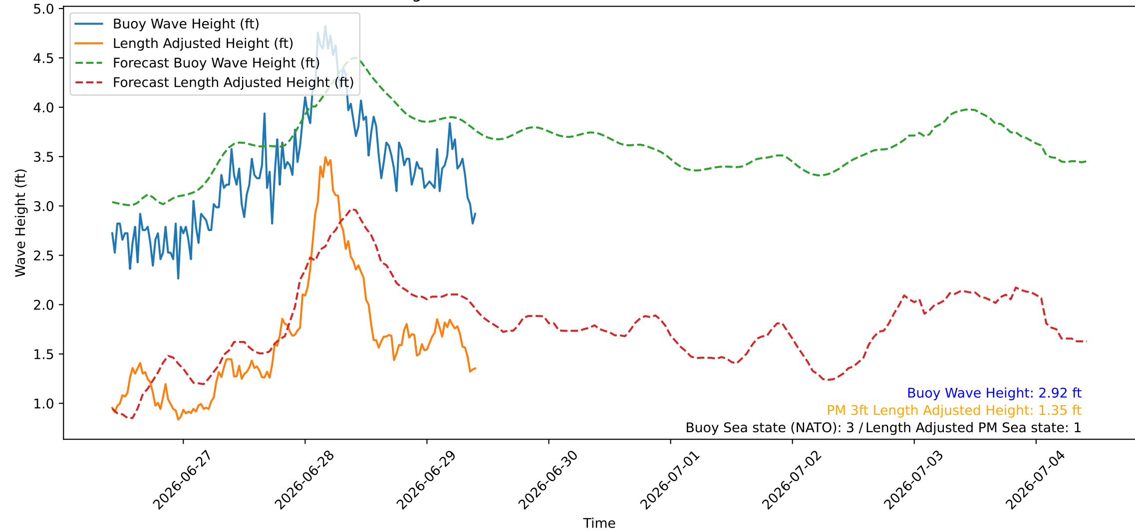
Wave Heights over Time for Green Beach at 2026-06-29 10:11:07
