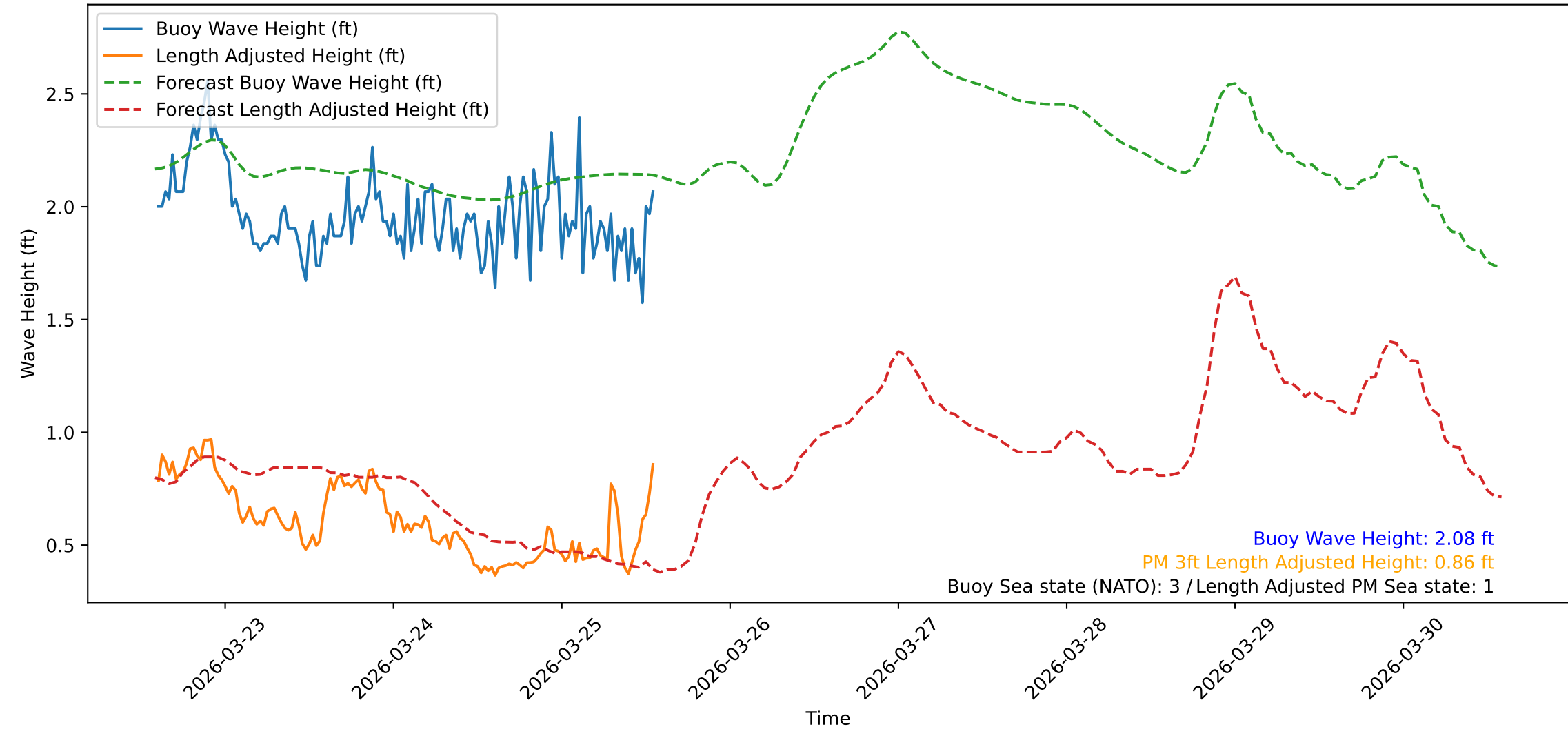
Wave Heights over Time for Red Beach at 2026-03-25 14:00:47
