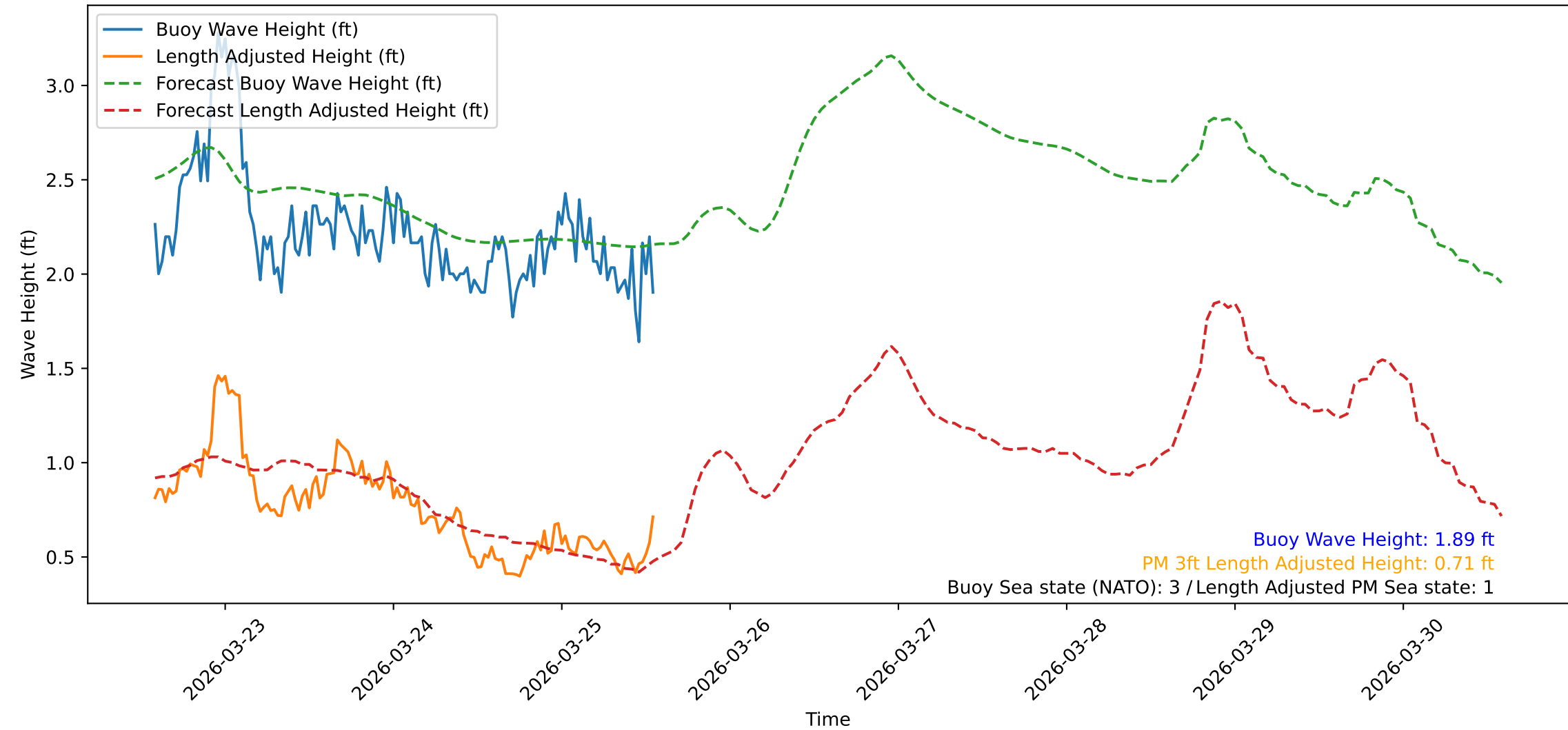
Wave Heights over Time for Green Beach at 2026-03-25 14:01:09
