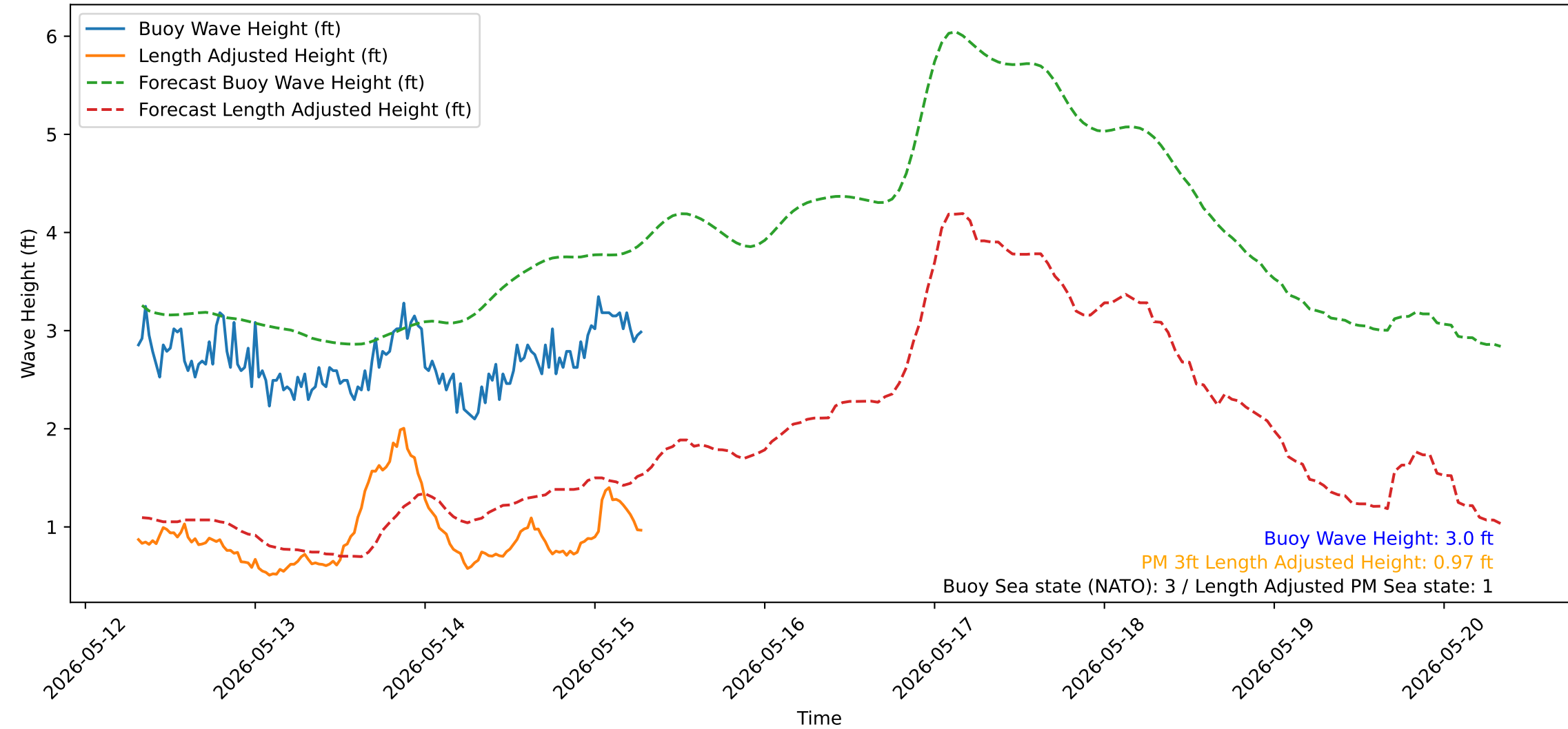
Wave Heights over Time for Green Beach at 2026-05-15 07:31:14
