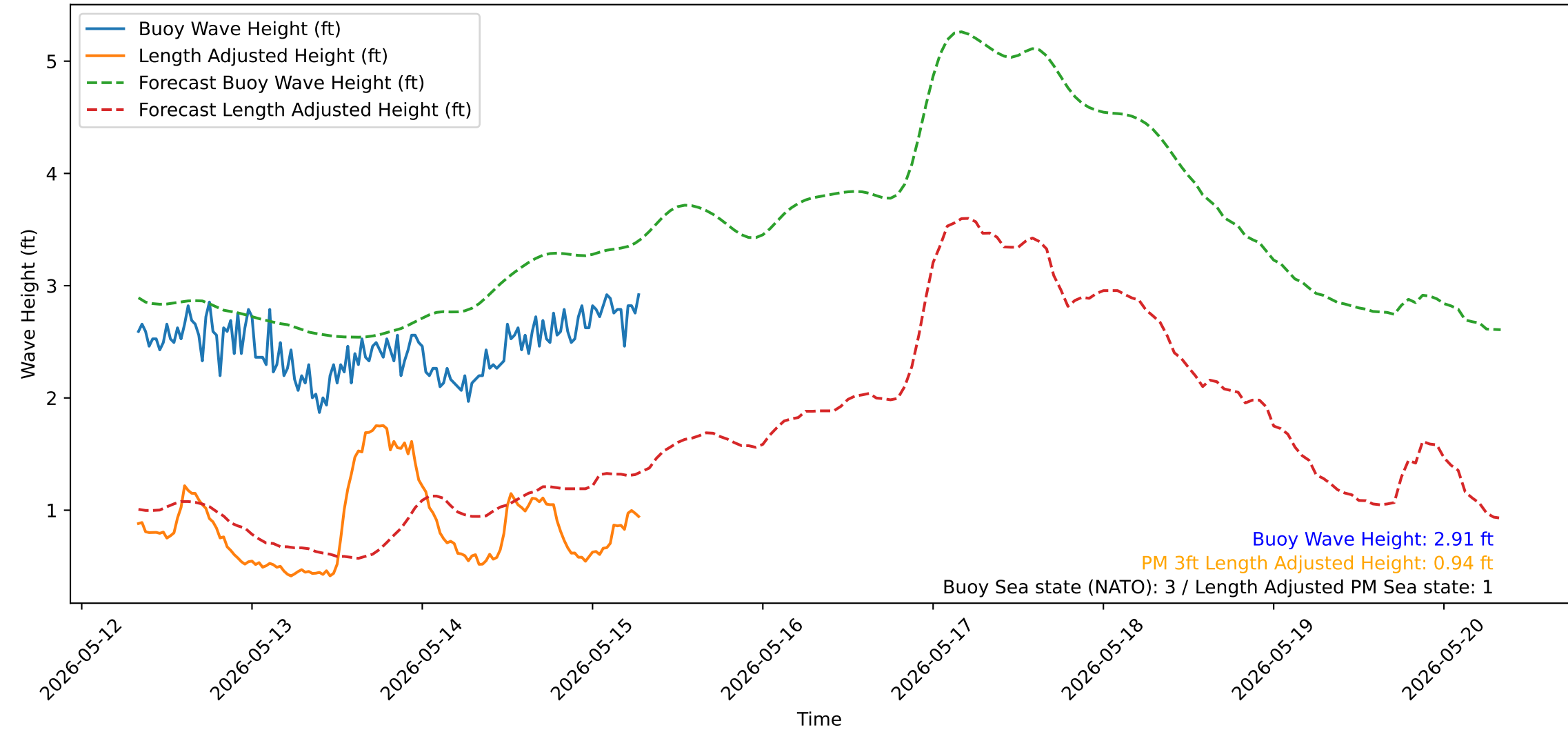
Wave Heights over Time for Red Beach at 2026-05-15 07:30:51
