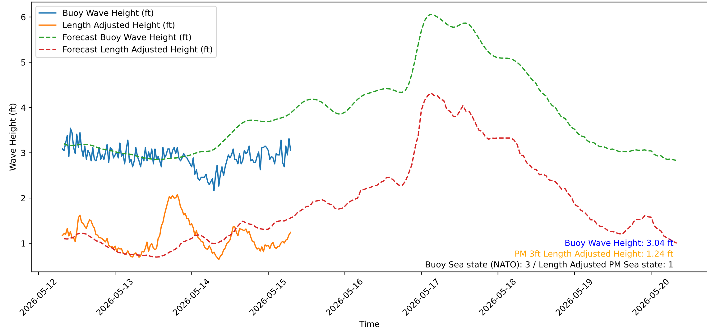
Wave Heights over Time for Oceanside Harbor at 2026-05-15 07:30:32
