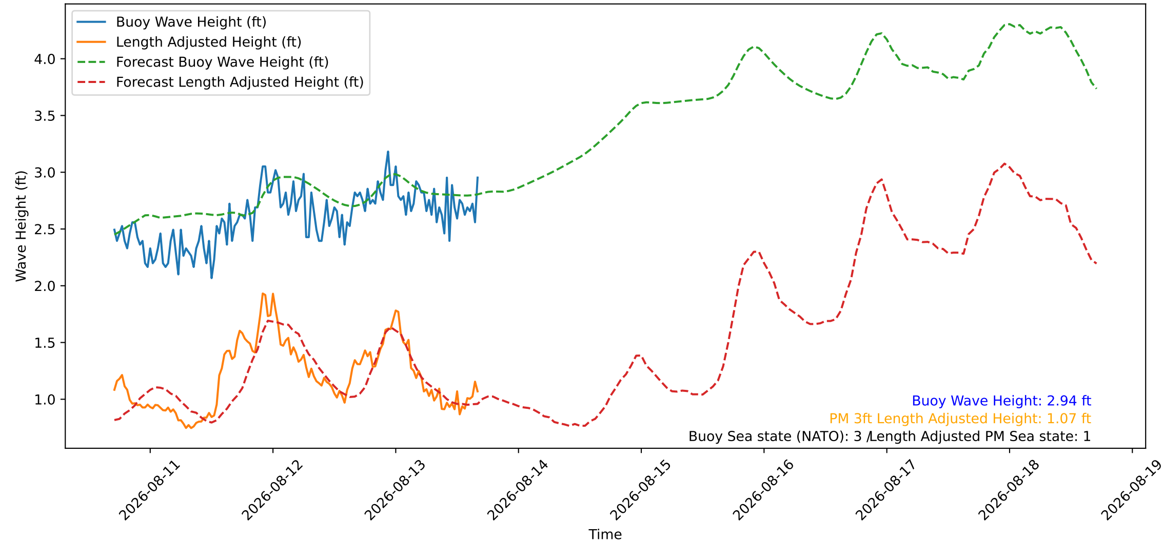
Wave Heights over Time for Oceanside Harbor at 2026-08-13 16:50:27
