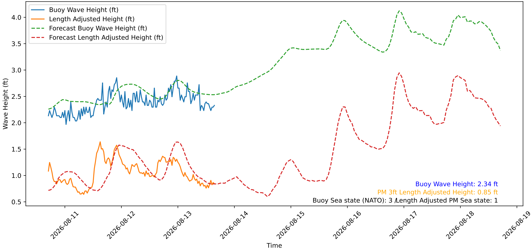
Wave Heights over Time for Red Beach at 2026-08-13 16:50:47
