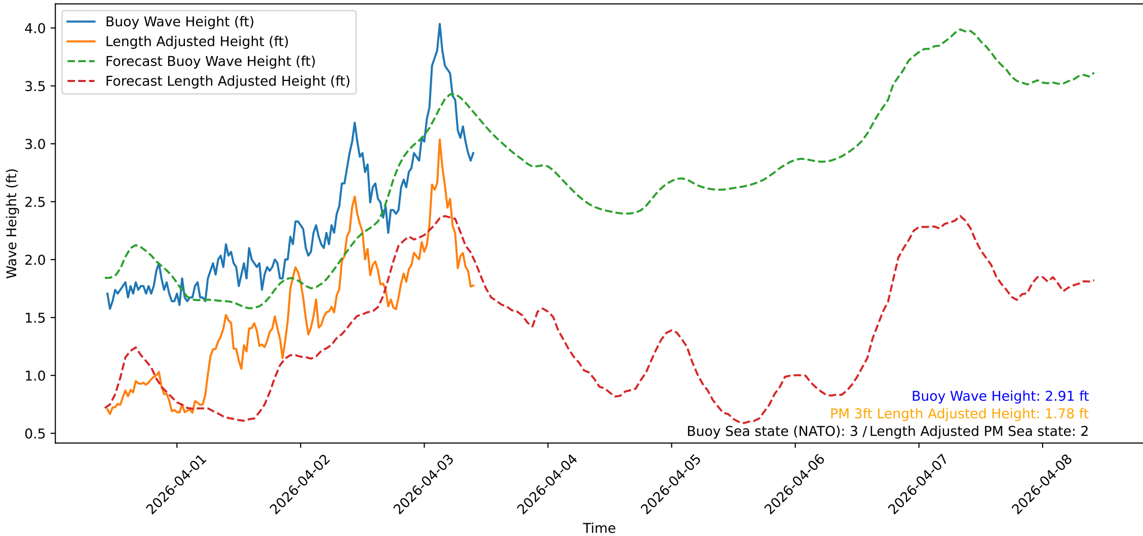
Wave Heights over Time for Oceanside Harbor at 2026-04-03 10:20:31
