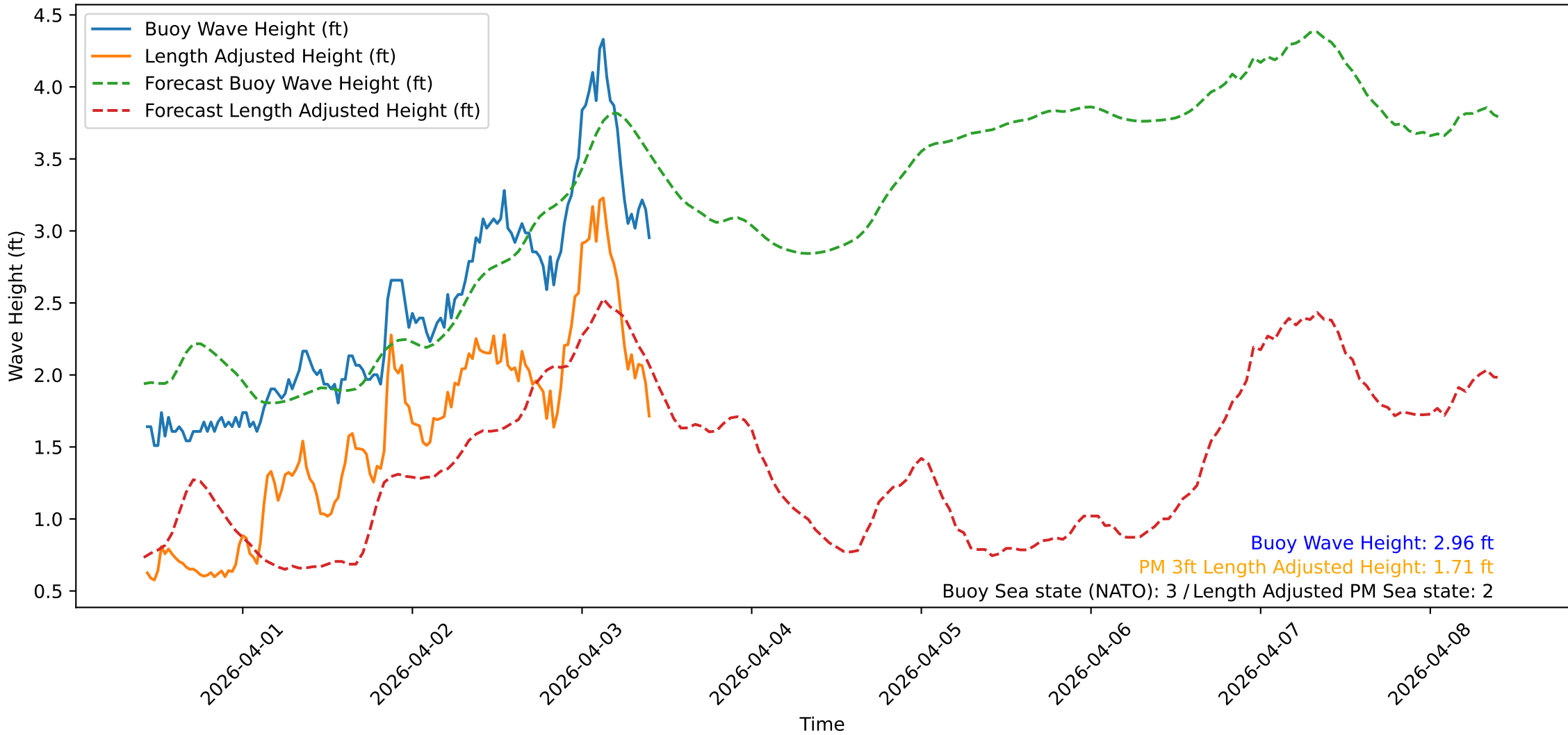
Wave Heights over Time for Green Beach at 2026-04-03 10:21:09
