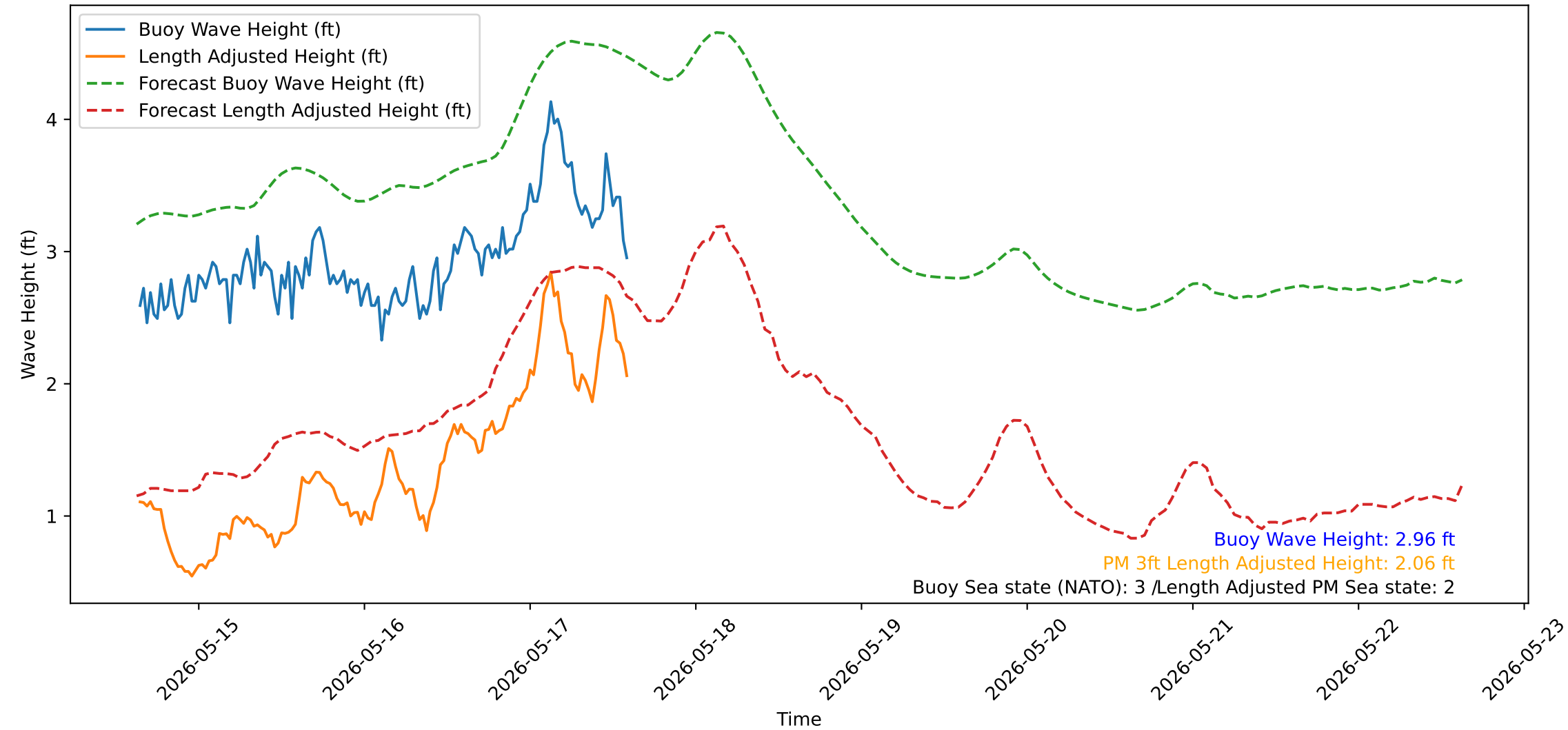
Wave Heights over Time for Red Beach at 2026-05-17 15:00:51
