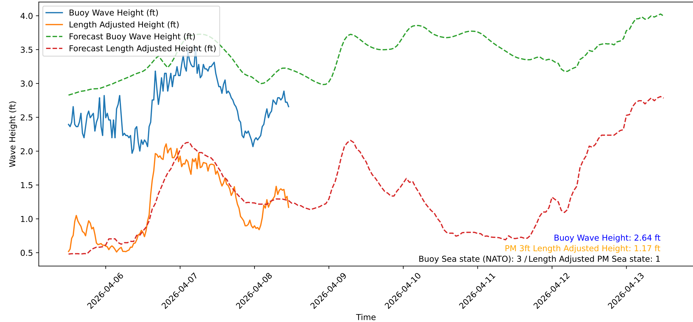
Wave Heights over Time for Red Beach at 2026-04-08 11:40:48
