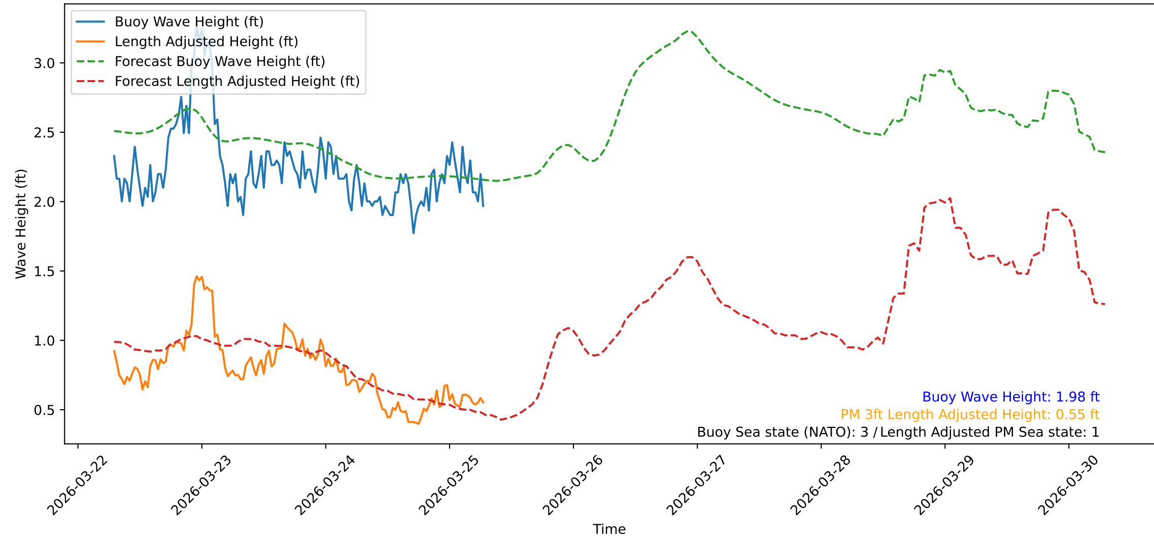
Wave Heights over Time for Green Beach at 2026-03-25 07:11:10
