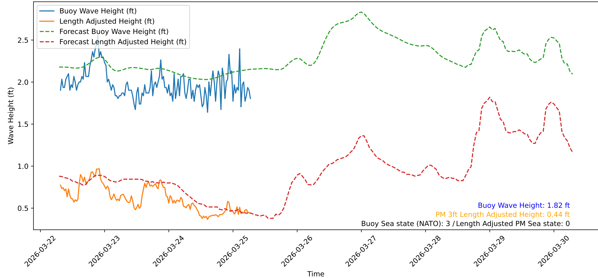
Wave Heights over Time for Red Beach at 2026-03-25 07:10:47
