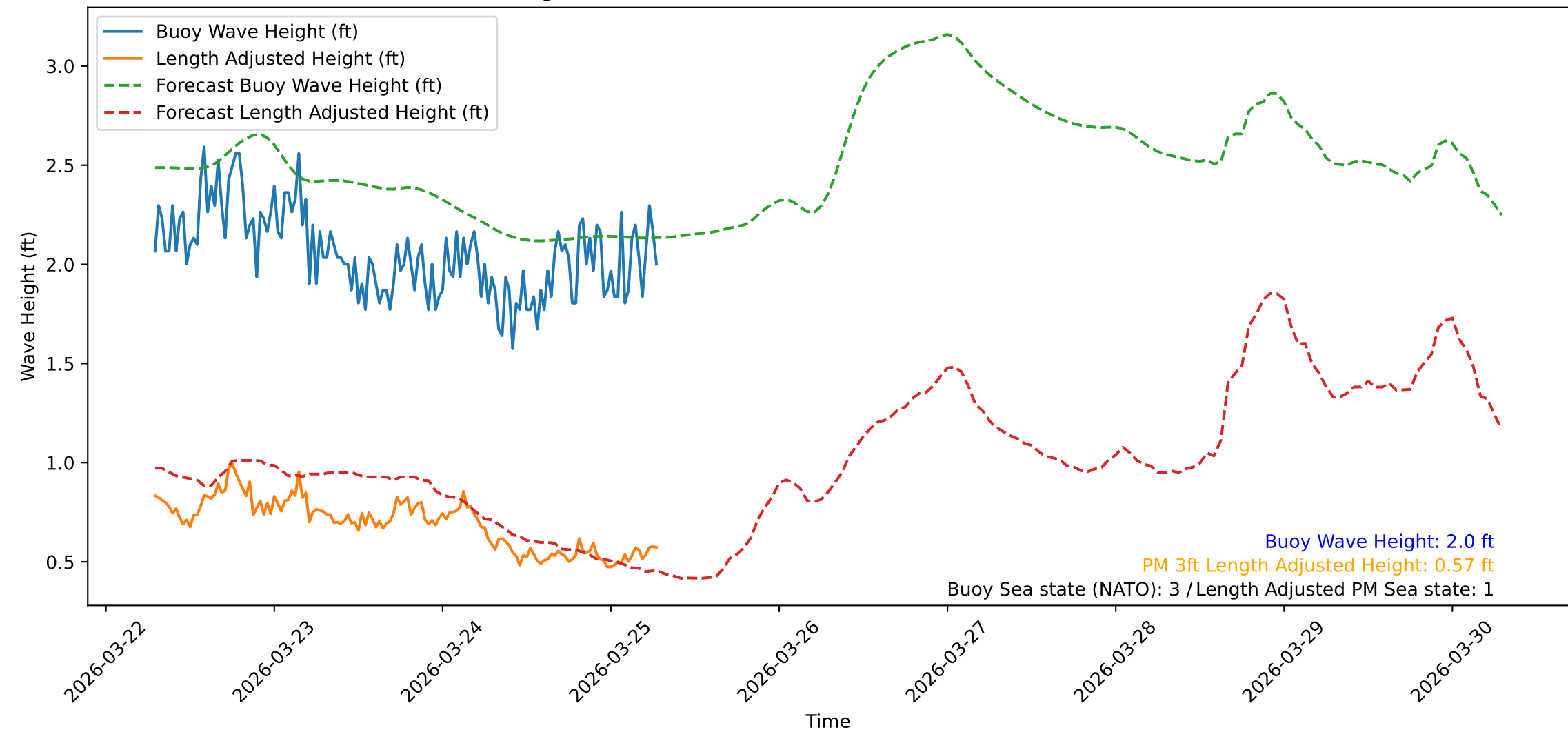
Wave Heights over Time for Oceanside Harbor at 2026-03-25 07:10:32
