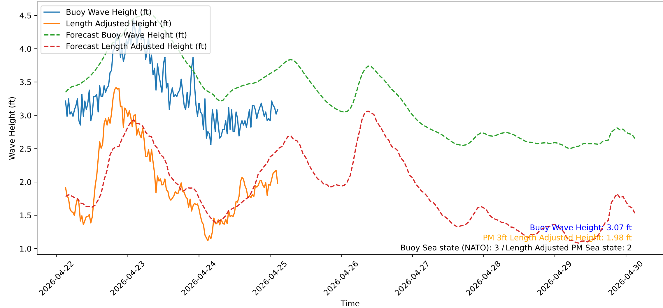
Wave Heights over Time for Oceanside Harbor at 2026-04-25 03:00:32
