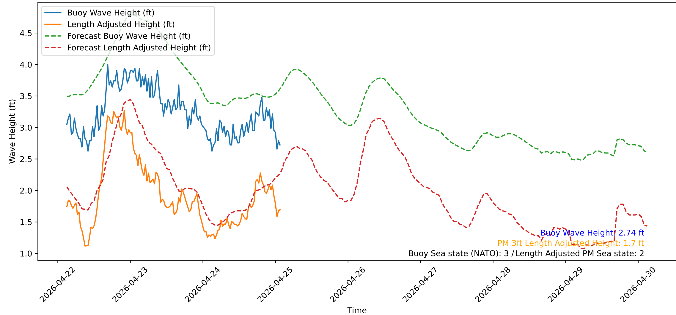
Wave Heights over Time for Green Beach at 2026-04-25 03:01:13
