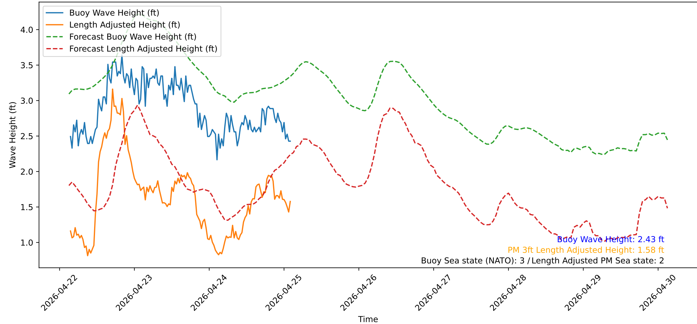
Wave Heights over Time for Red Beach at 2026-04-25 03:00:51
