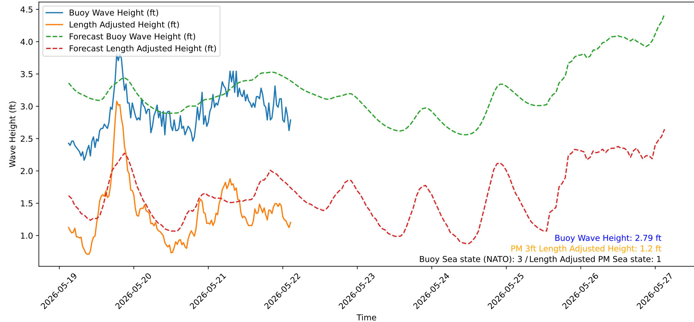
Wave Heights over Time for Green Beach at 2026-05-22 03:11:13
