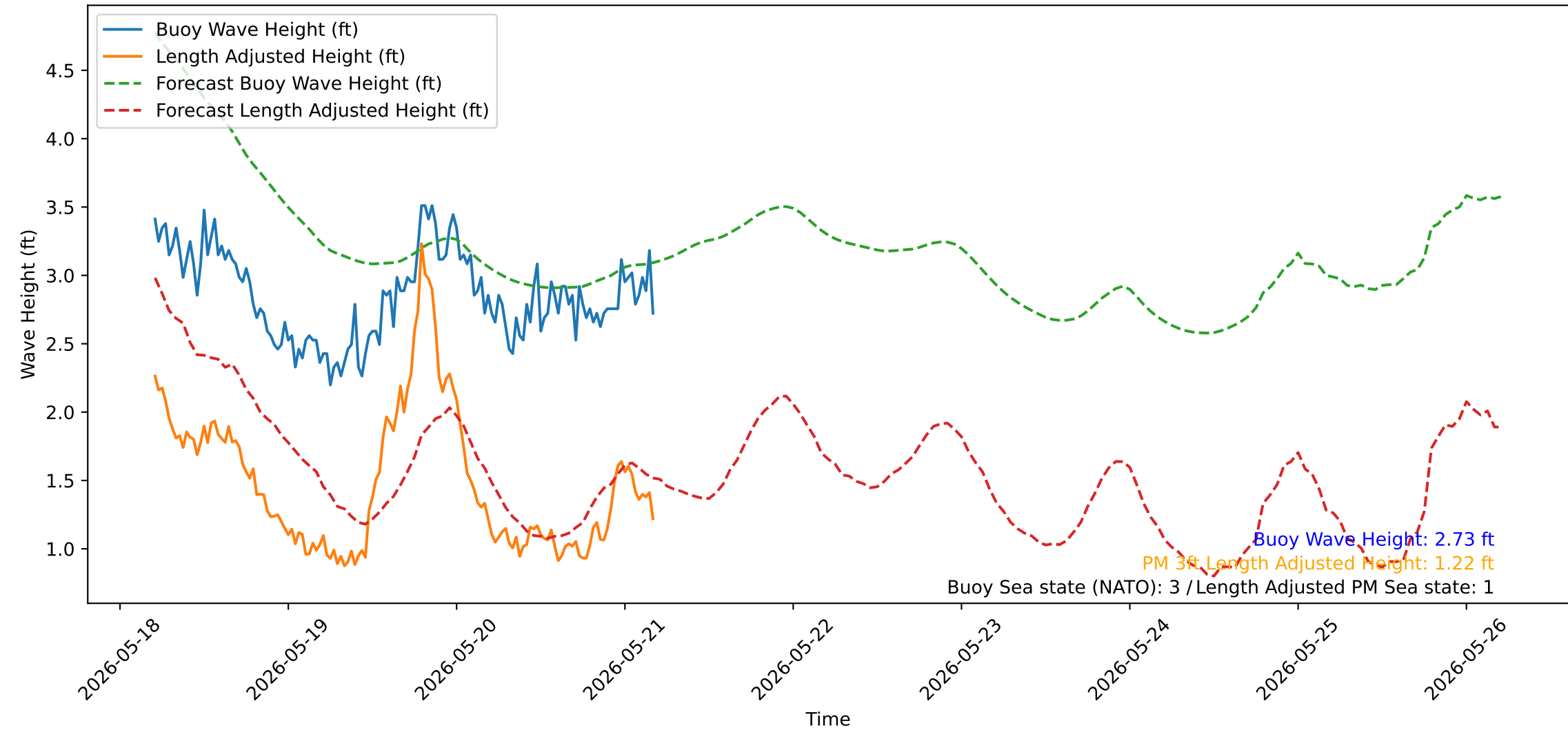
Wave Heights over Time for Oceanside Harbor at 2026-05-21 04:50:31
