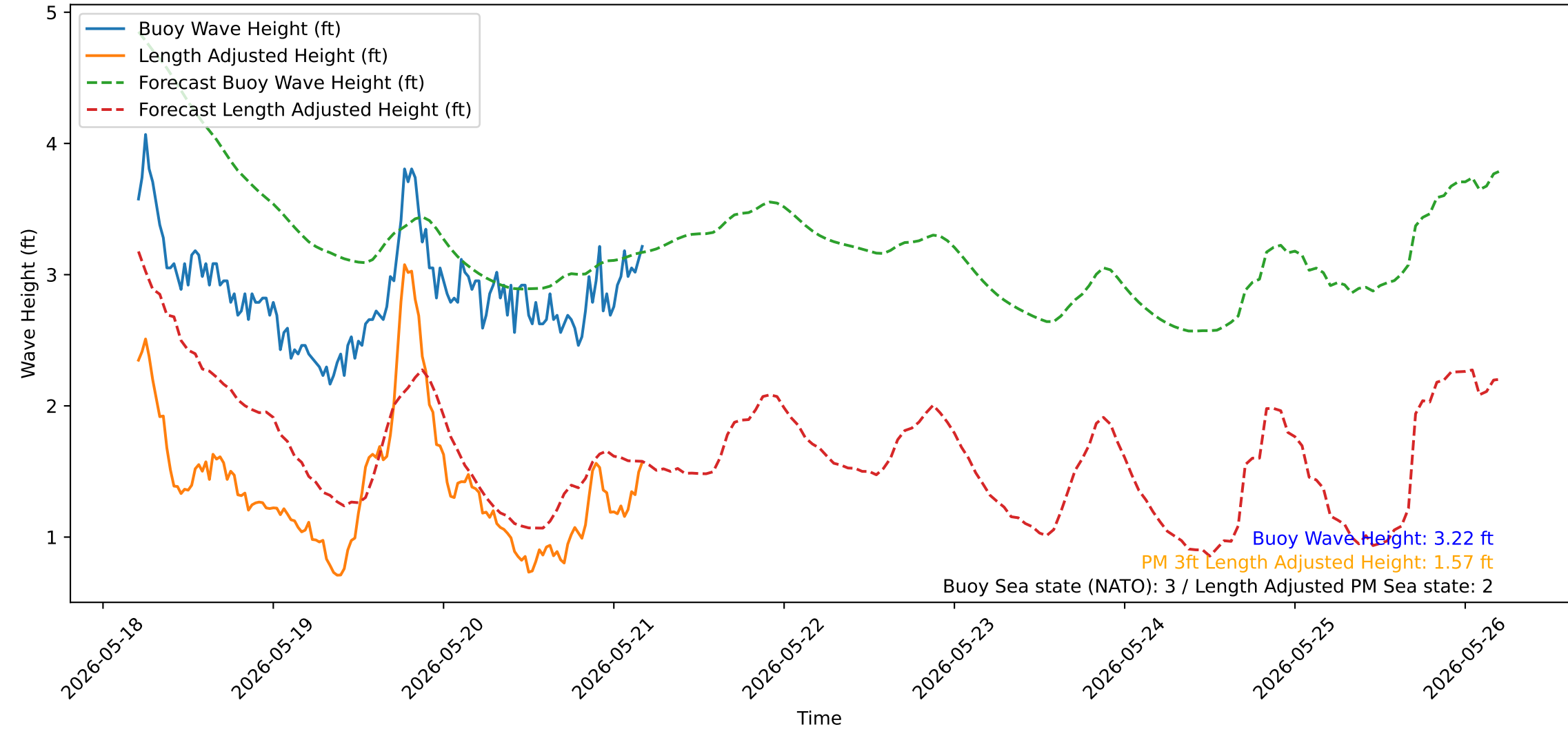
Wave Heights over Time for Green Beach at 2026-05-21 04:51:14
