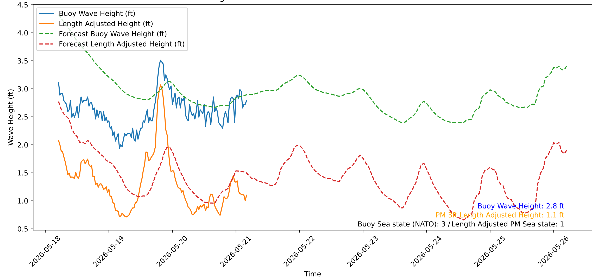
Wave Heights over Time for Red Beach at 2026-05-21 04:50:51
