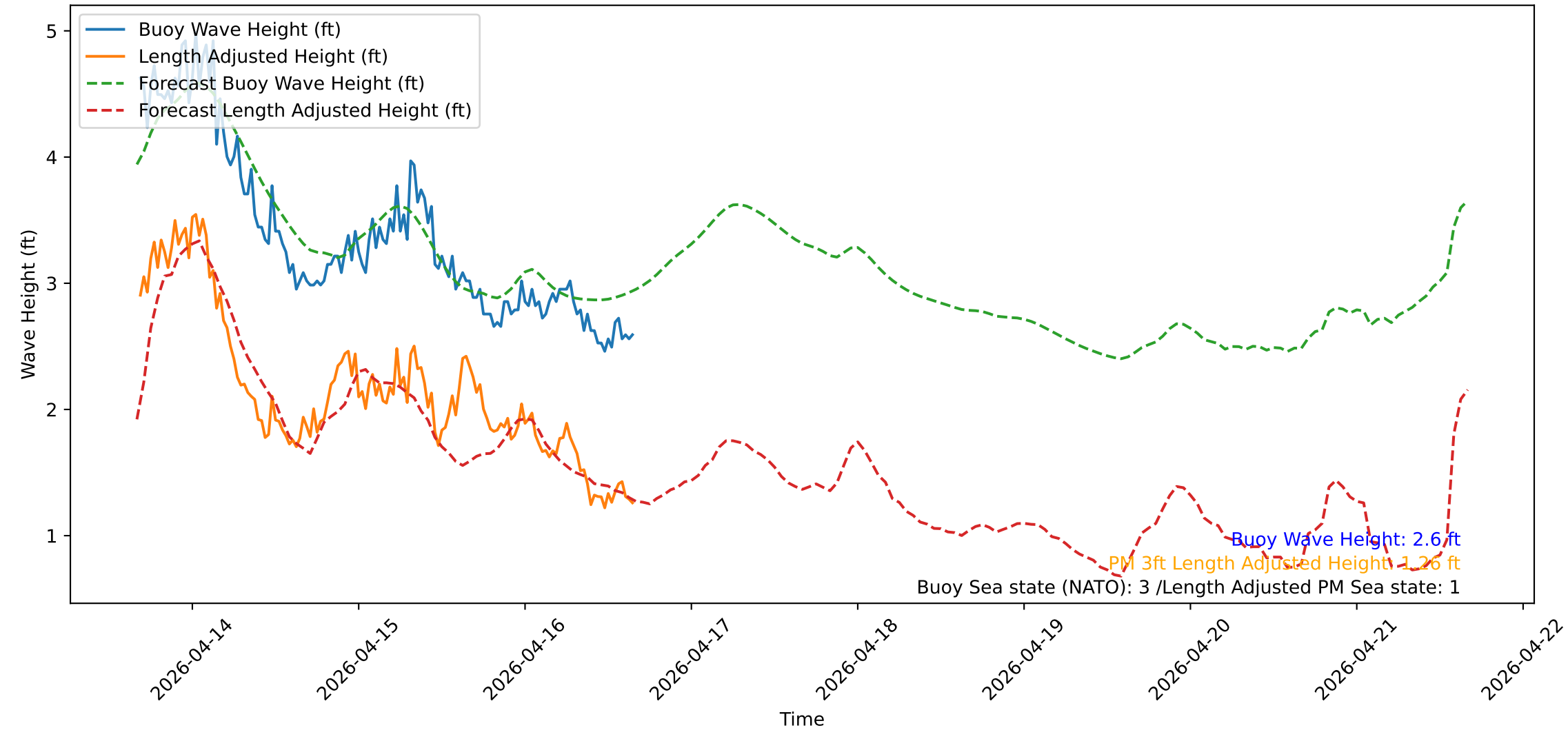
Wave Heights over Time for Green Beach at 2026-04-16 16:21:18
