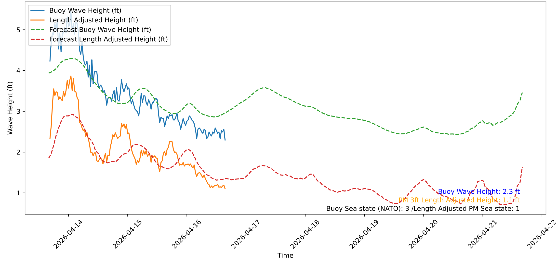
Wave Heights over Time for Oceanside Harbor at 2026-04-16 16:20:33
