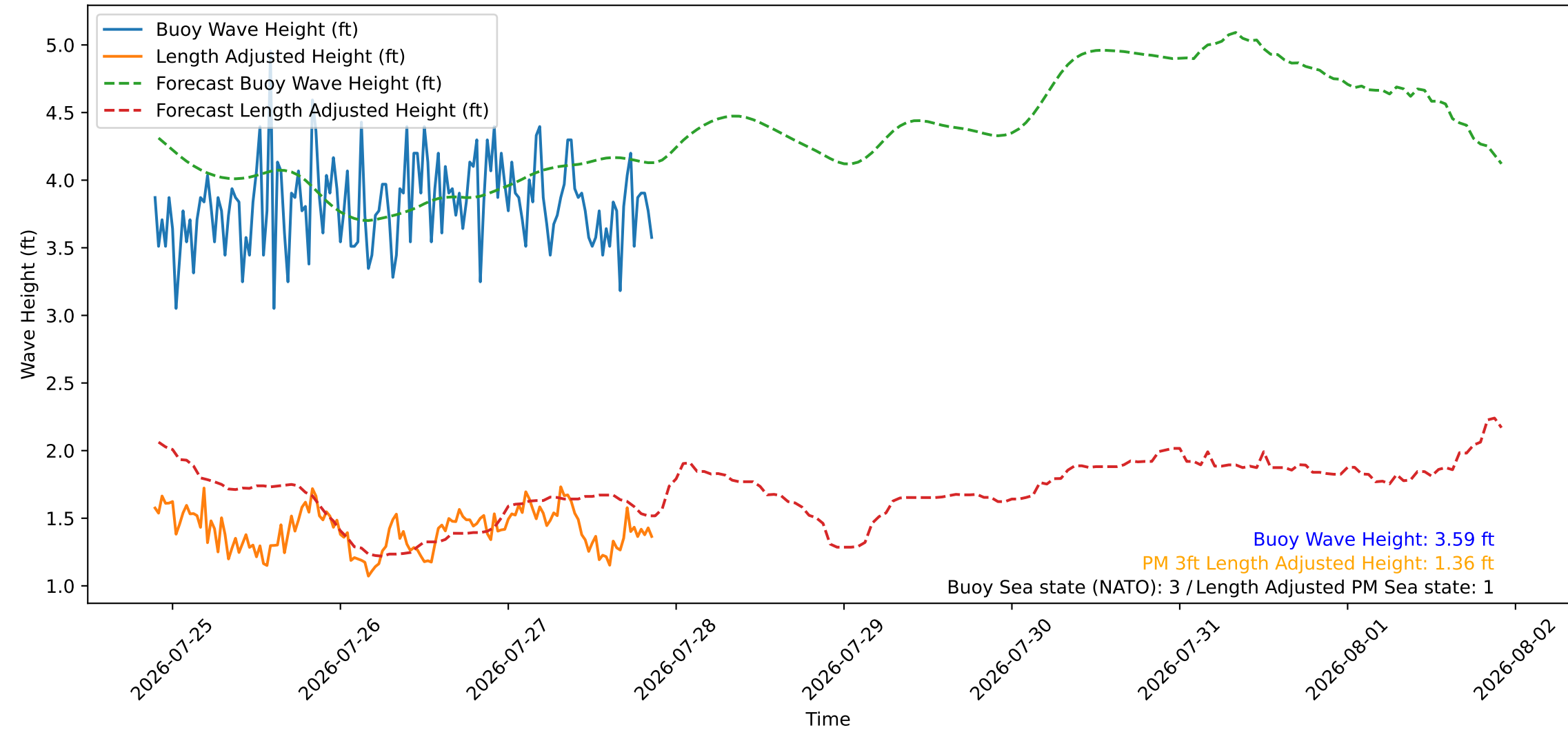
Wave Heights over Time for Oceanside Harbor at 2026-07-27 21:30:26
