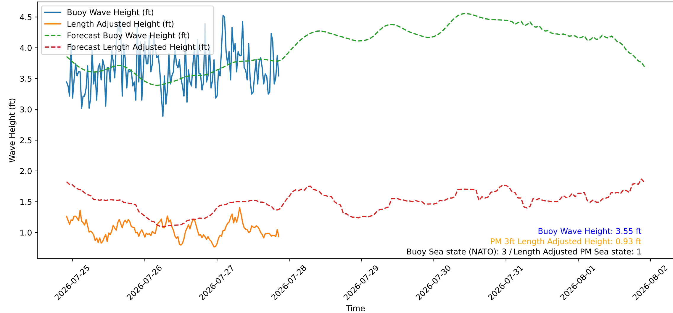
Wave Heights over Time for Red Beach at 2026-07-27 21:30:46
