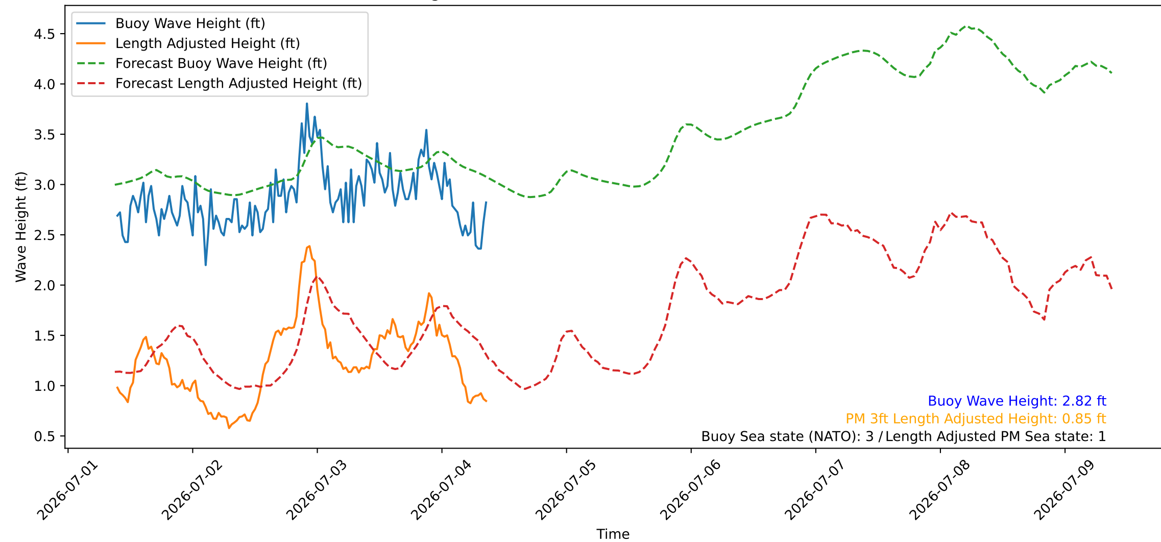
Wave Heights over Time for Red Beach at 2026-07-04 09:20:48
