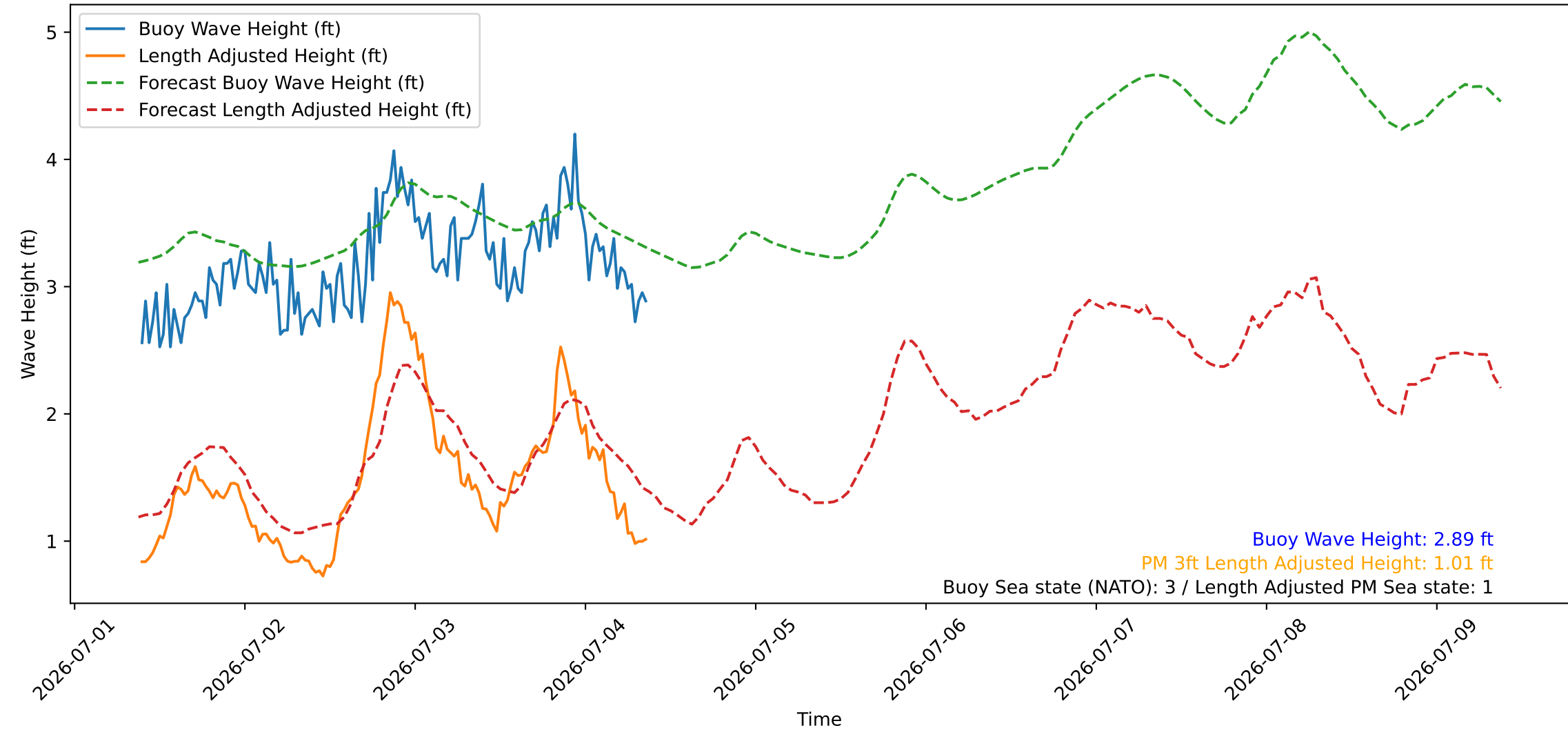
Wave Heights over Time for Green Beach at 2026-07-04 09:21:10
