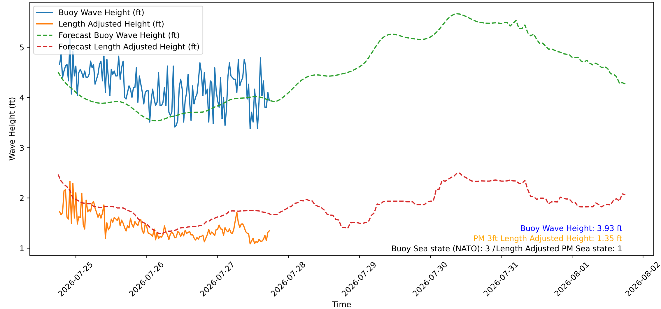
Wave Heights over Time for Green Beach at 2026-07-27 18:21:10
