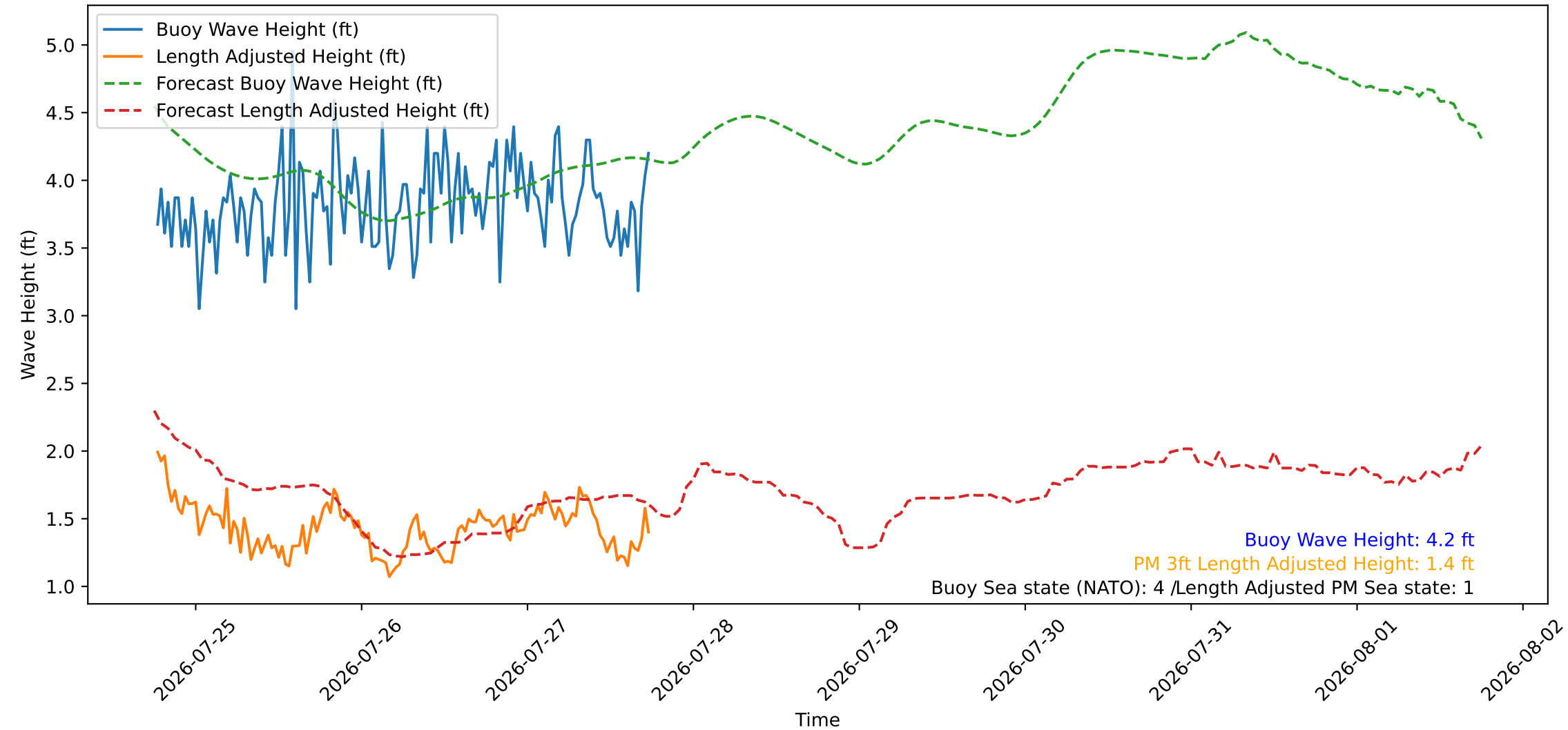
Wave Heights over Time for Oceanside Harbor at 2026-07-27 18:20:26
