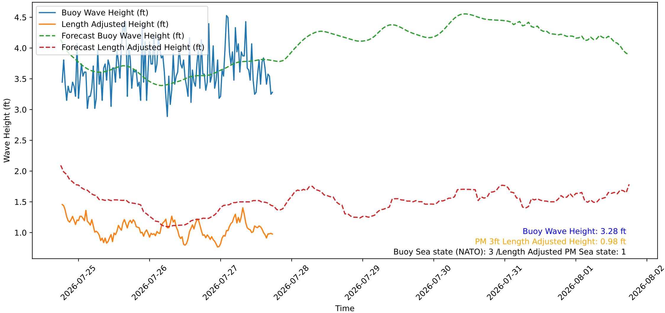
Wave Heights over Time for Red Beach at 2026-07-27 18:20:47
