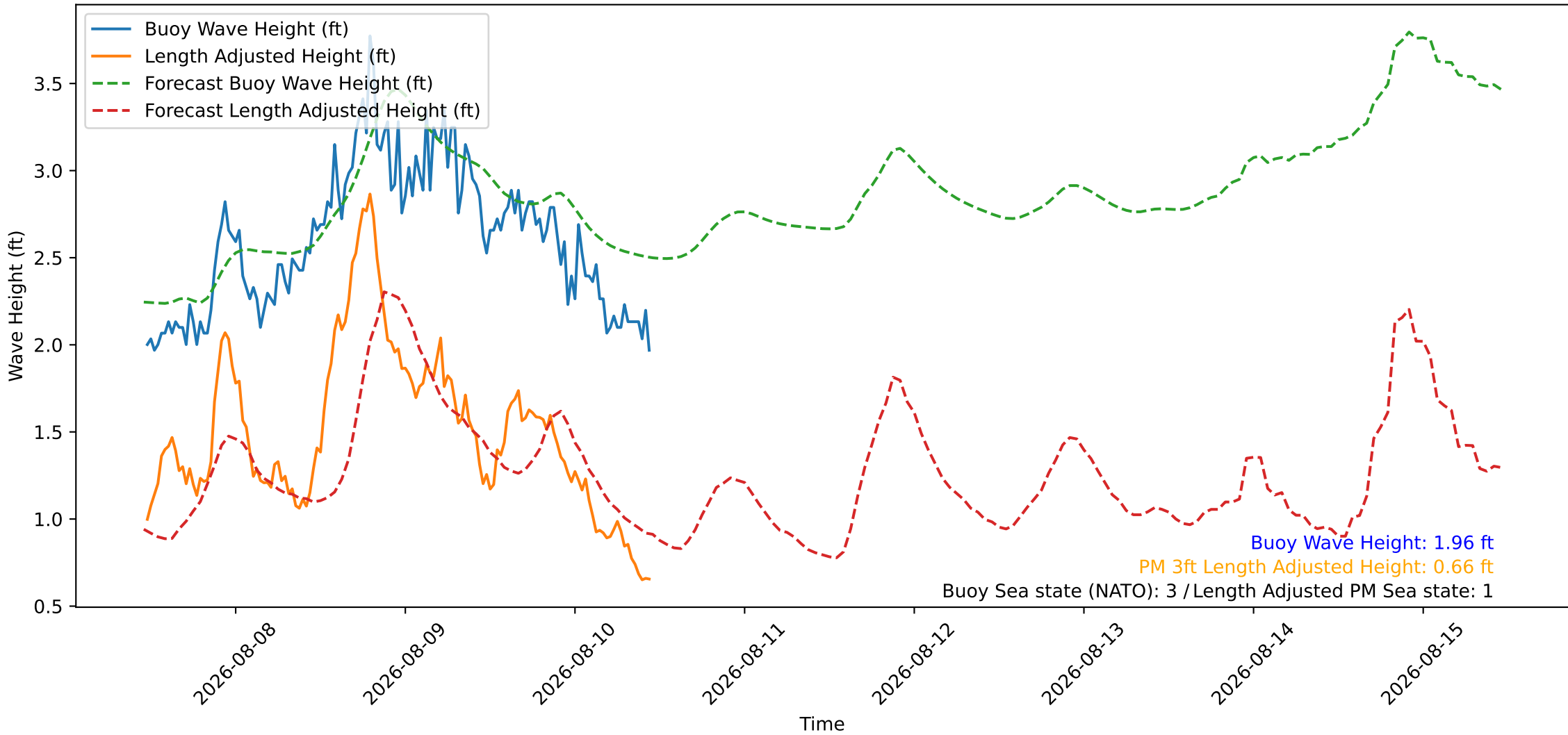
Wave Heights over Time for Green Beach at 2026-08-10 11:21:10
