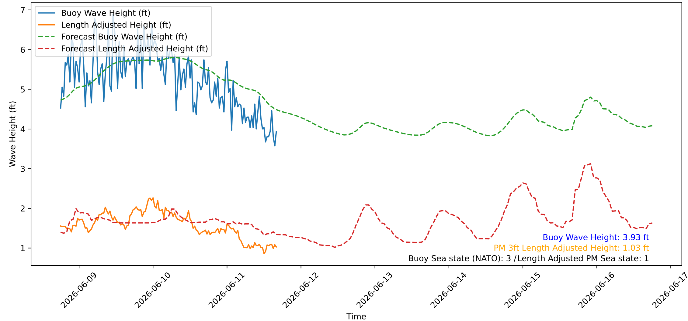
Wave Heights over Time for Green Beach at 2026-06-11 18:01:08
