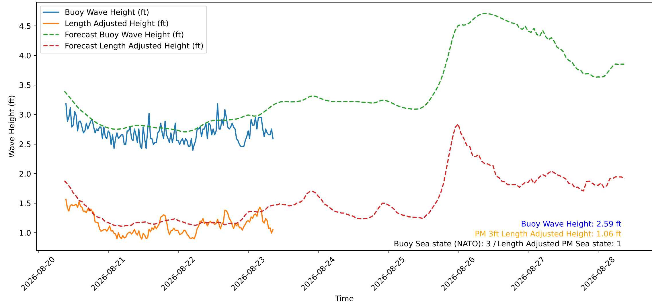
Wave Heights over Time for Green Beach at 2026-08-23 09:21:14
