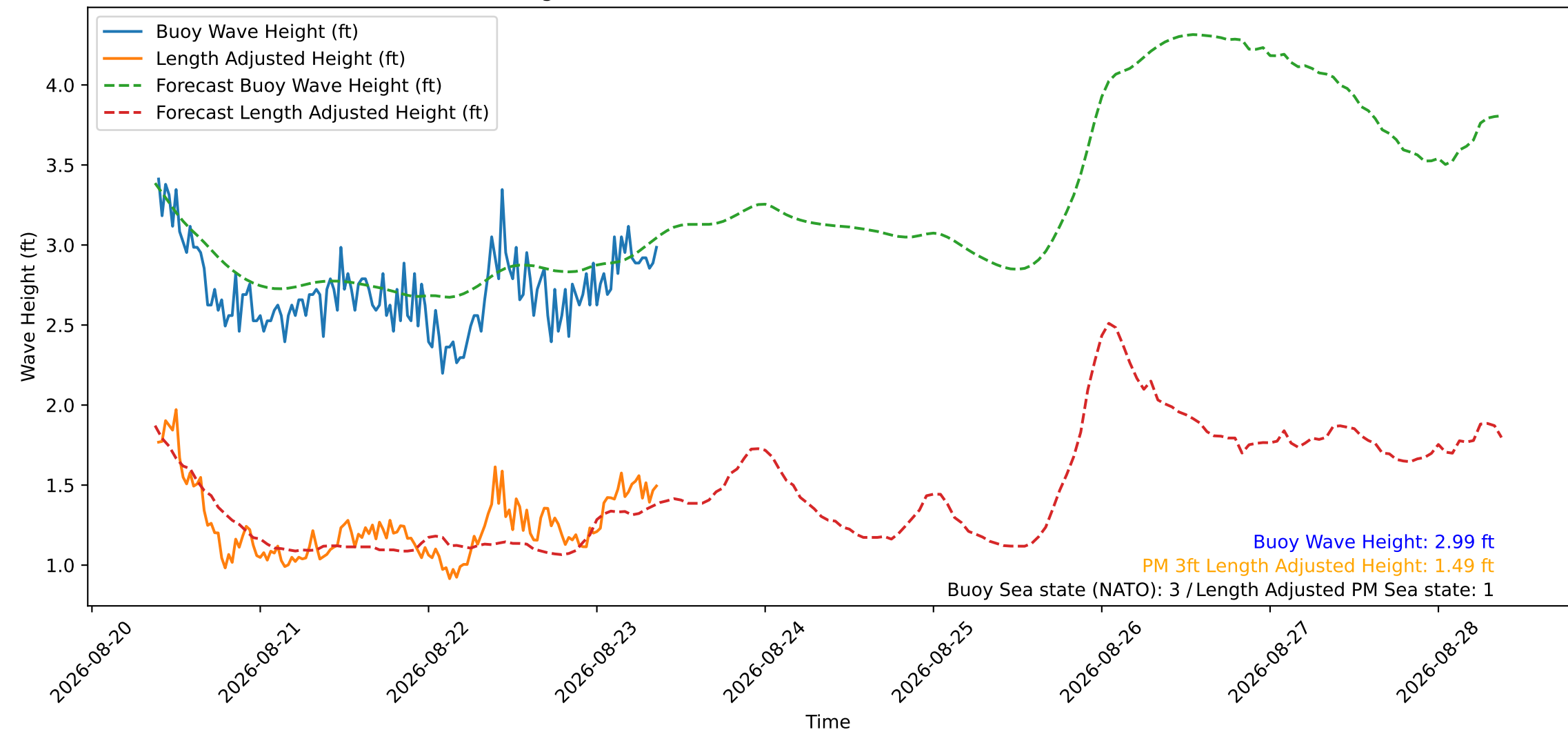
Wave Heights over Time for Oceanside Harbor at 2026-08-23 09:20:29
