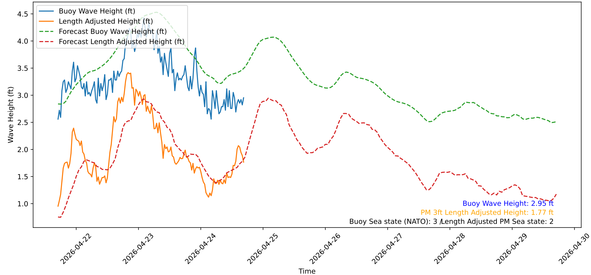
Wave Heights over Time for Oceanside Harbor at 2026-04-24 17:10:31
