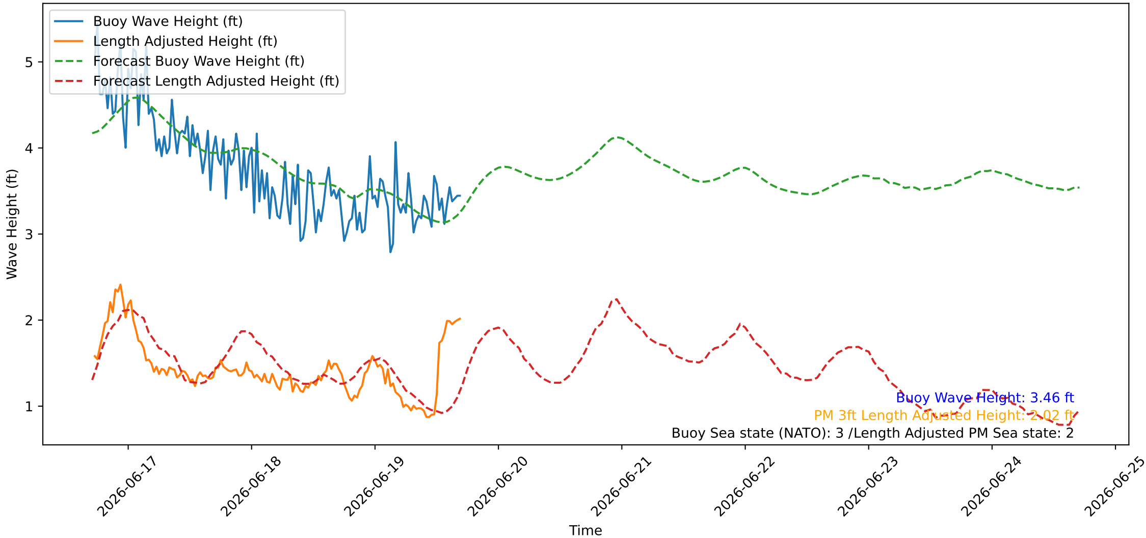
Wave Heights over Time for Oceanside Harbor at 2026-06-19 17:20:27
