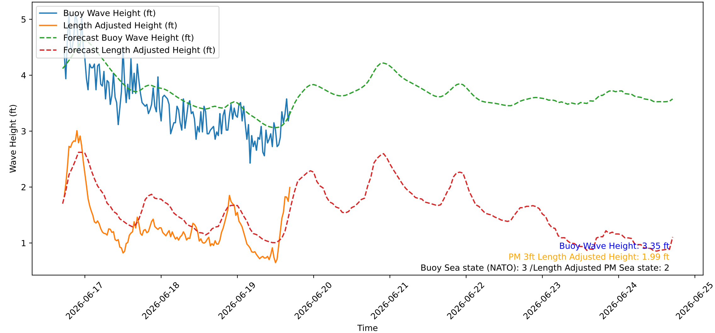
Wave Heights over Time for Green Beach at 2026-06-19 17:21:09
