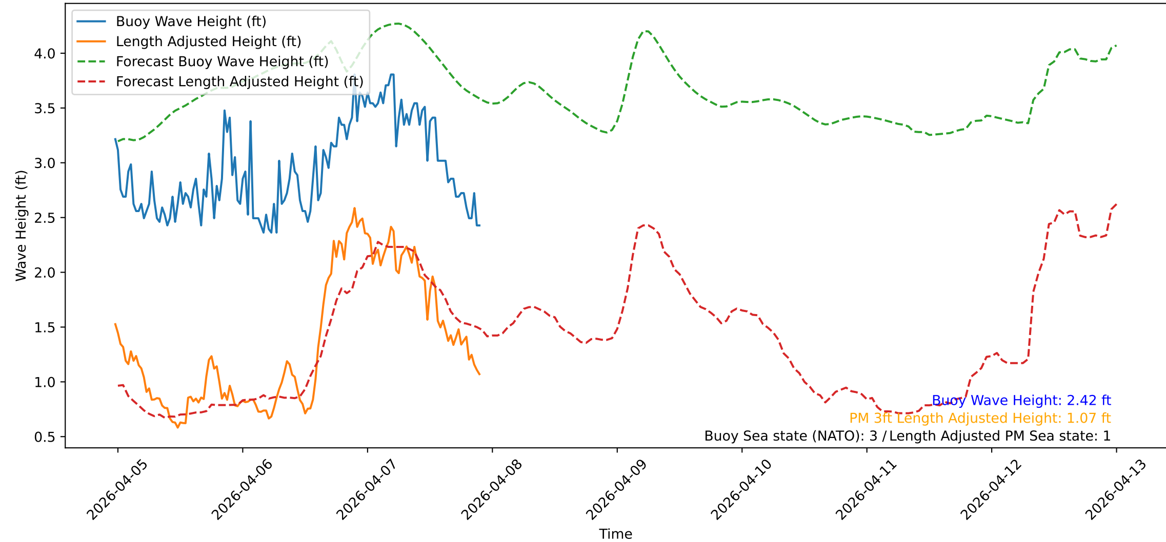
Wave Heights over Time for Green Beach at 2026-04-07 23:31:09
