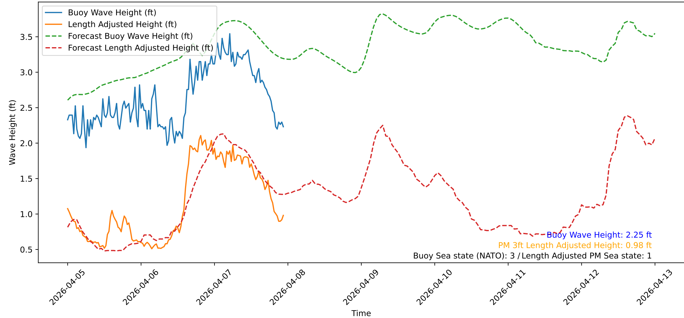
Wave Heights over Time for Red Beach at 2026-04-07 23:30:47
