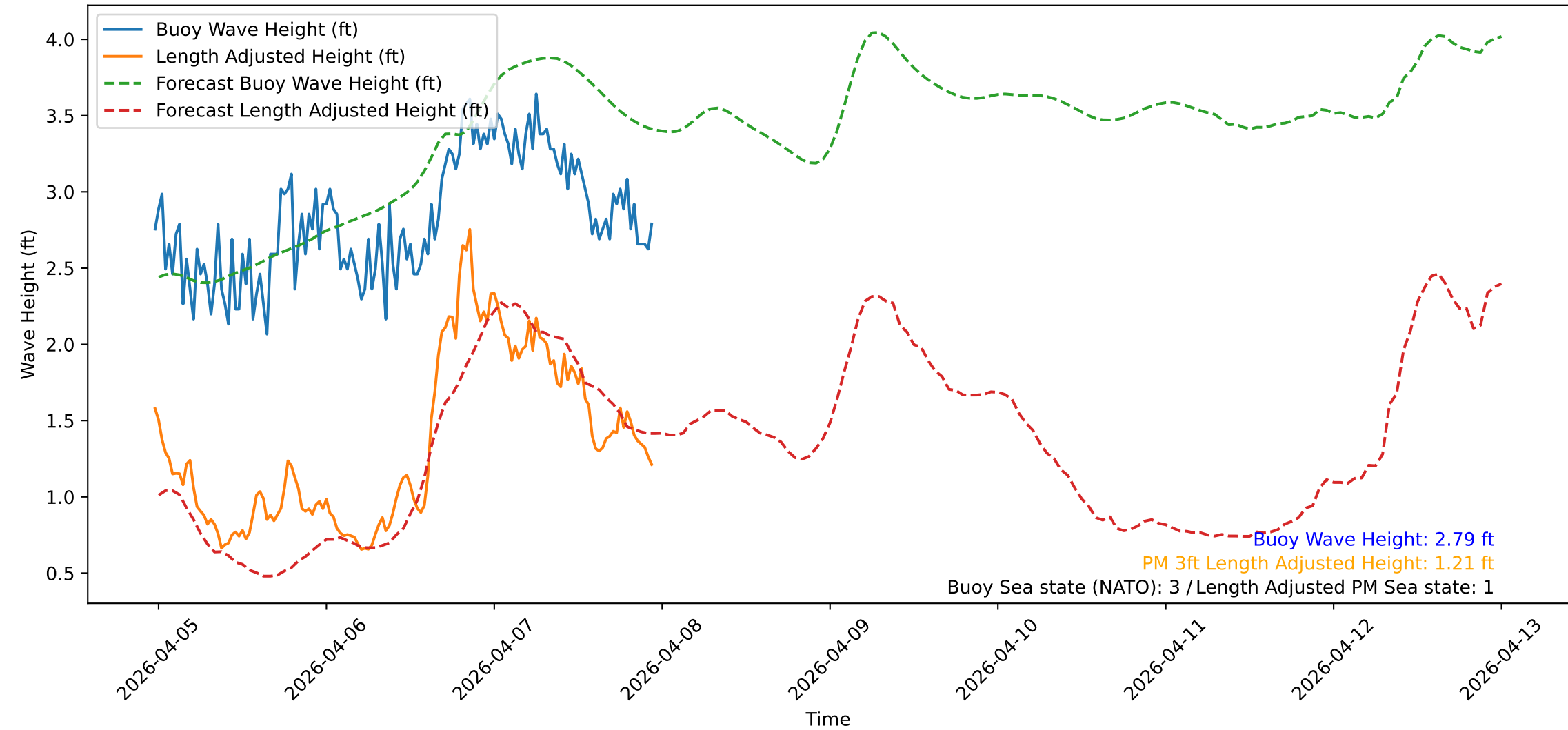
Wave Heights over Time for Oceanside Harbor at 2026-04-07 23:30:31
