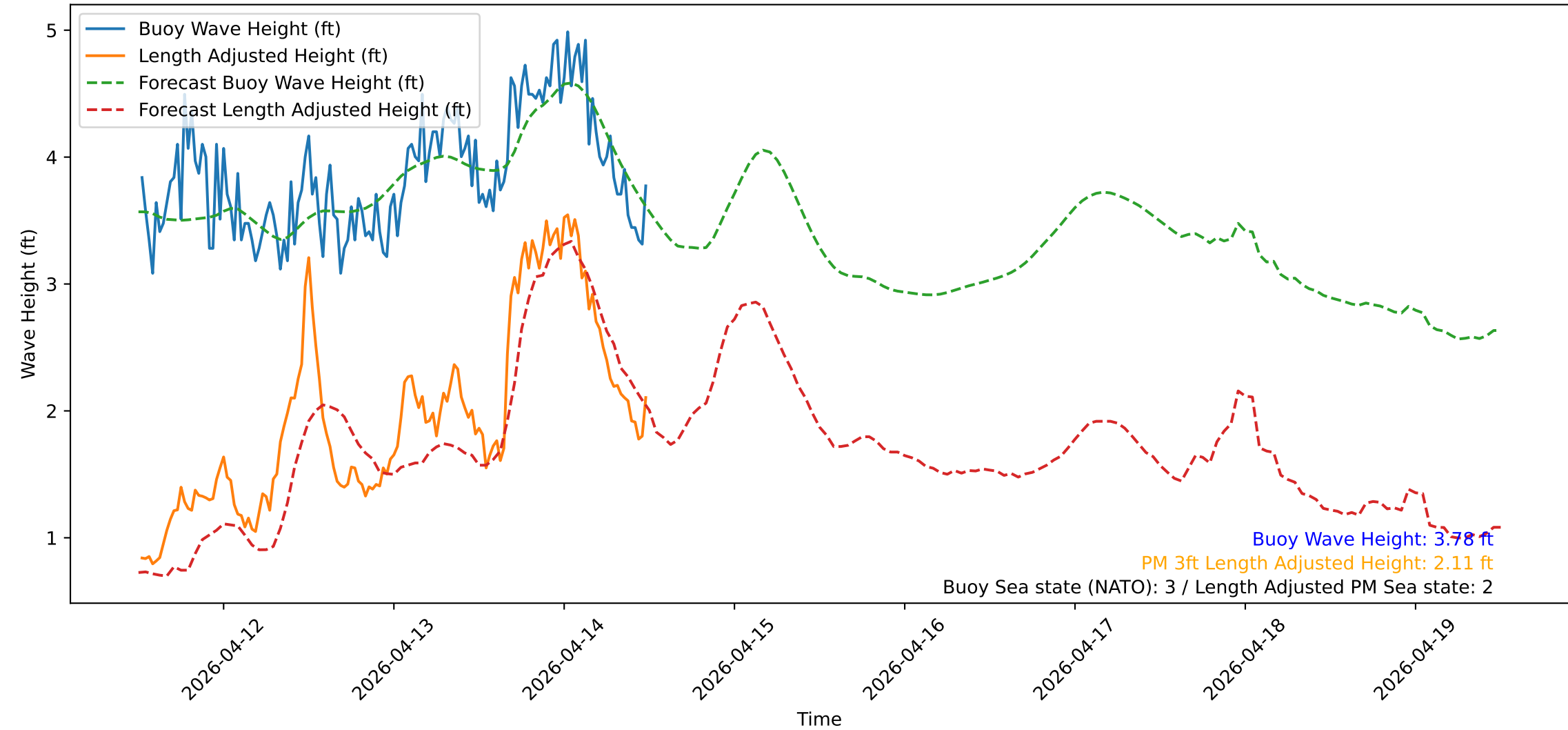
Wave Heights over Time for Green Beach at 2026-04-14 12:21:13
