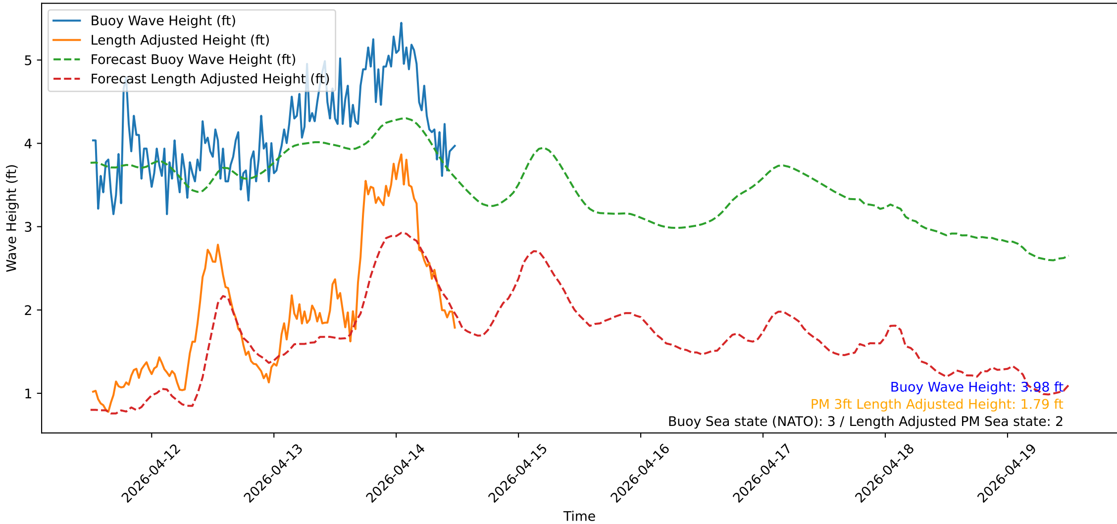
Wave Heights over Time for Oceanside Harbor at 2026-04-14 12:20:31
