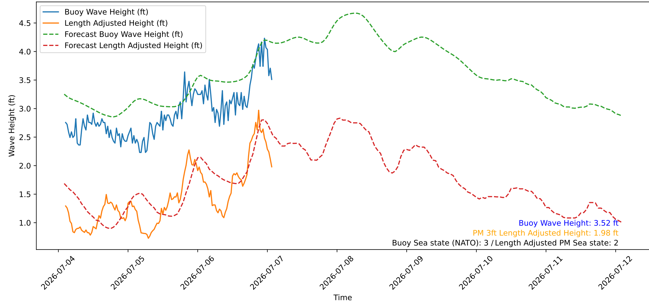
Wave Heights over Time for Red Beach at 2026-07-07 02:20:47
