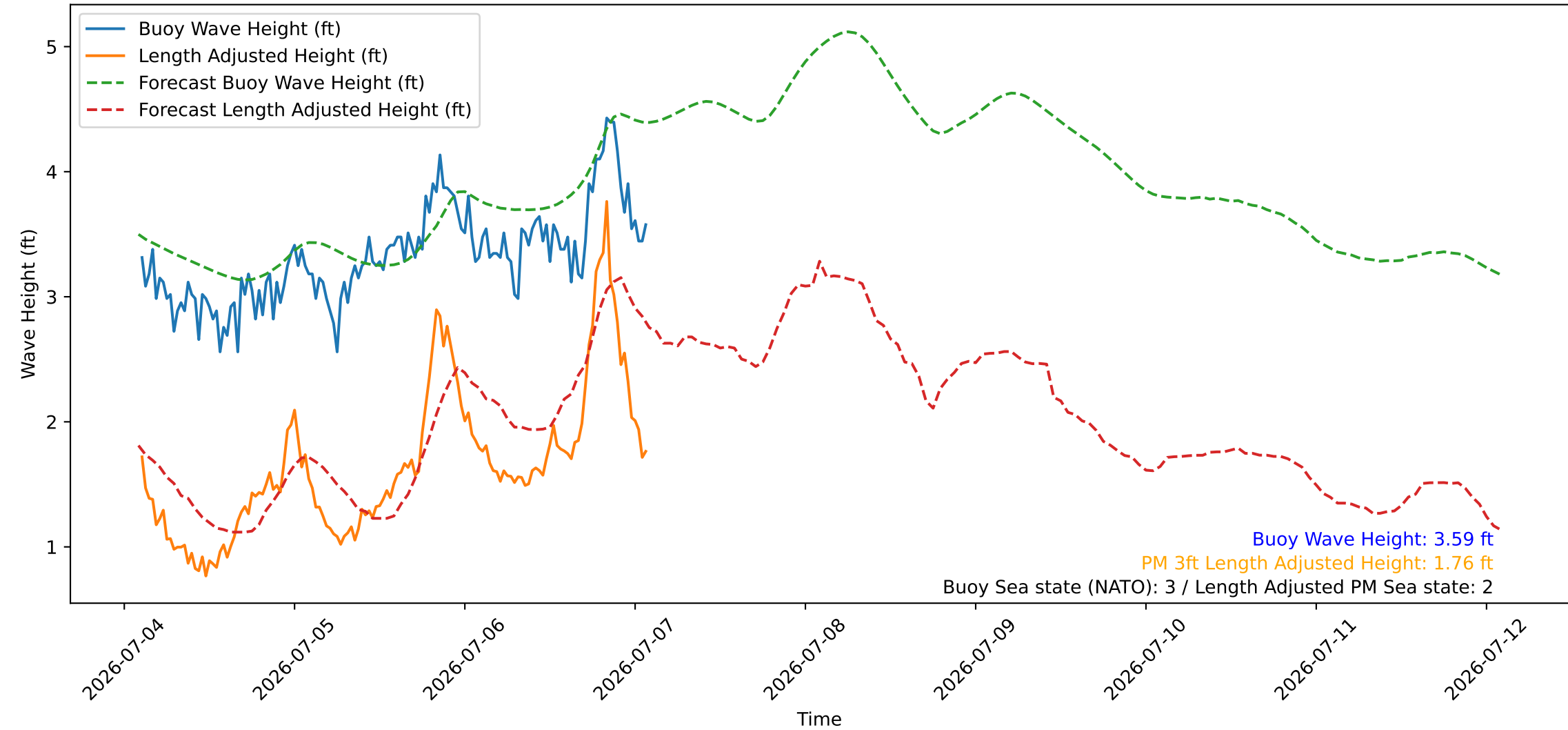
Wave Heights over Time for Green Beach at 2026-07-07 02:21:10
