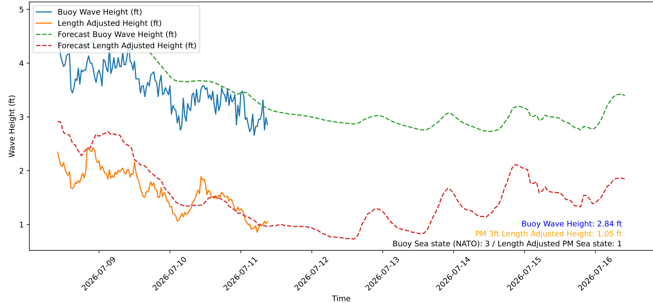
Wave Heights over Time for Green Beach at 2026-07-11 10:01:07
