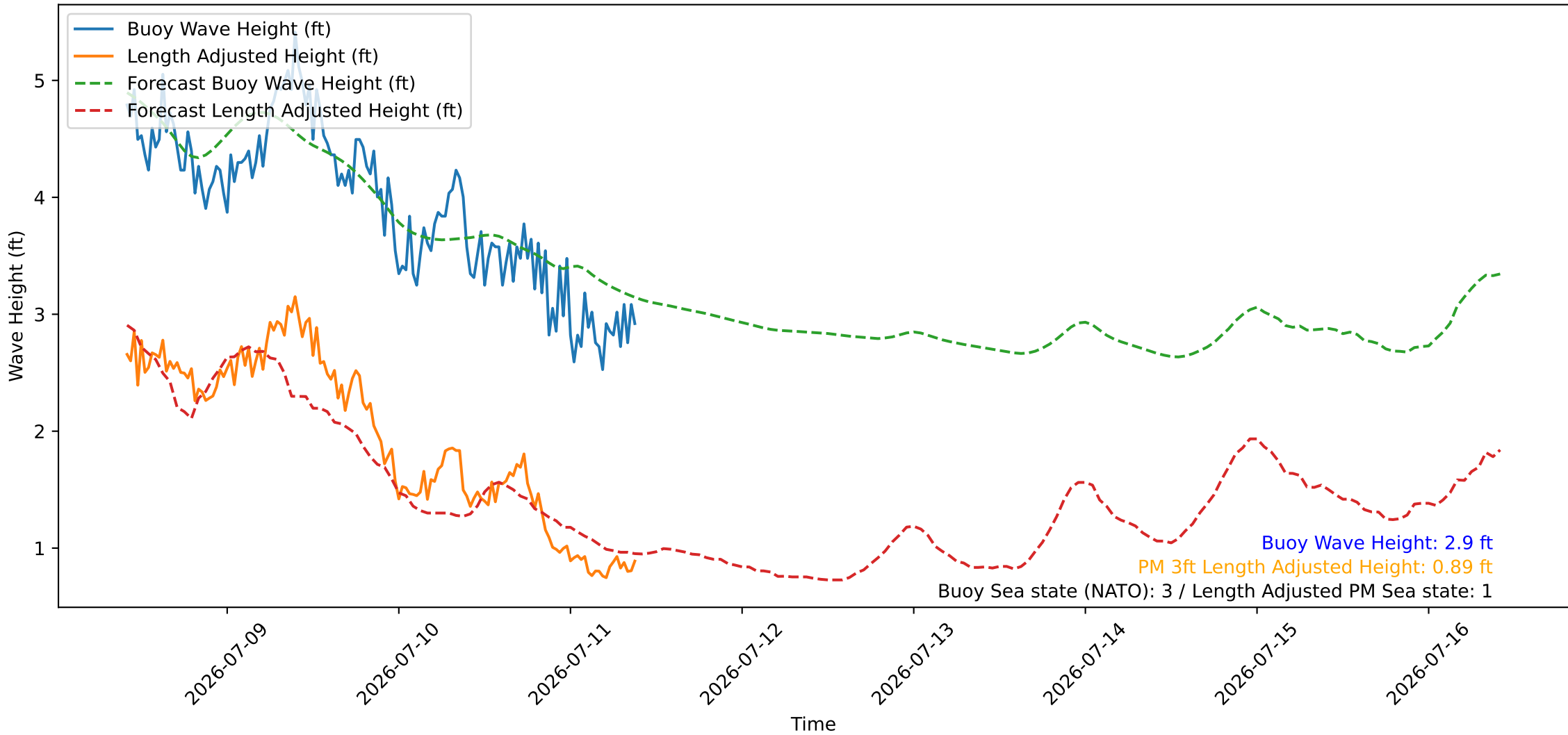
Wave Heights over Time for Oceanside Harbor at 2026-07-11 10:00:26
