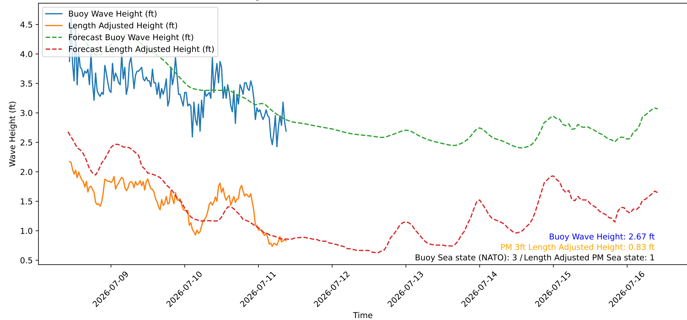
Wave Heights over Time for Red Beach at 2026-07-11 10:00:45
