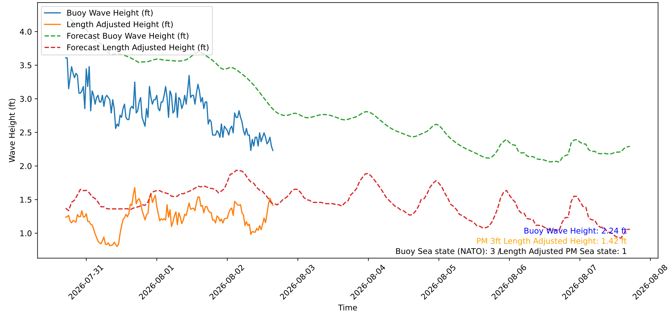
Wave Heights over Time for Red Beach at 2026-08-02 16:30:46
