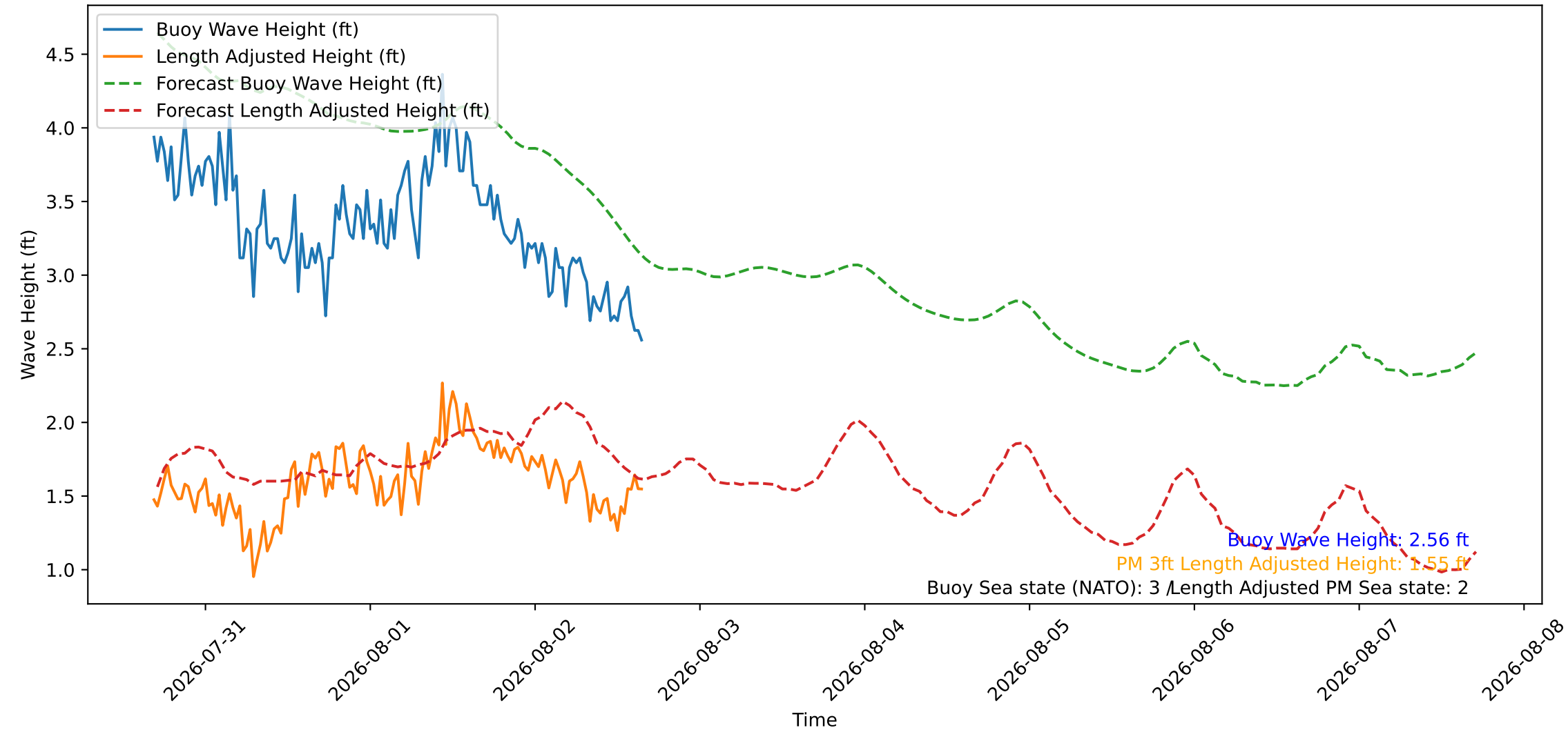
Wave Heights over Time for Oceanside Harbor at 2026-08-02 16:30:26
