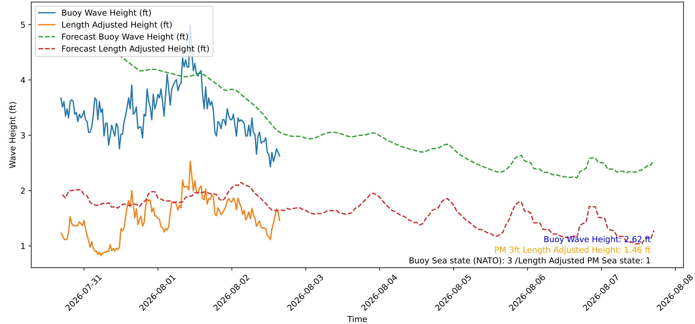
Wave Heights over Time for Green Beach at 2026-08-02 16:31:08
