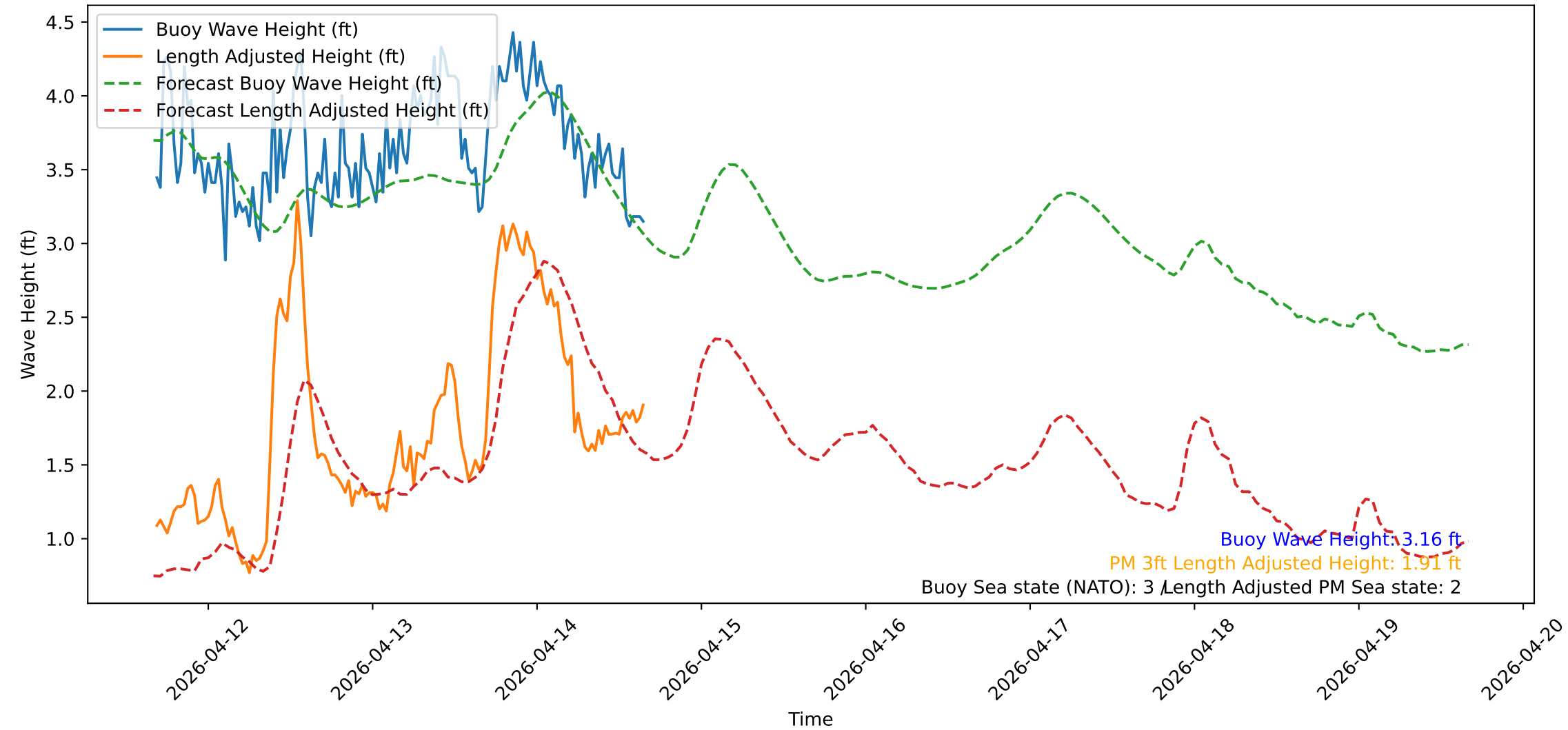
Wave Heights over Time for Red Beach at 2026-04-14 16:20:52
