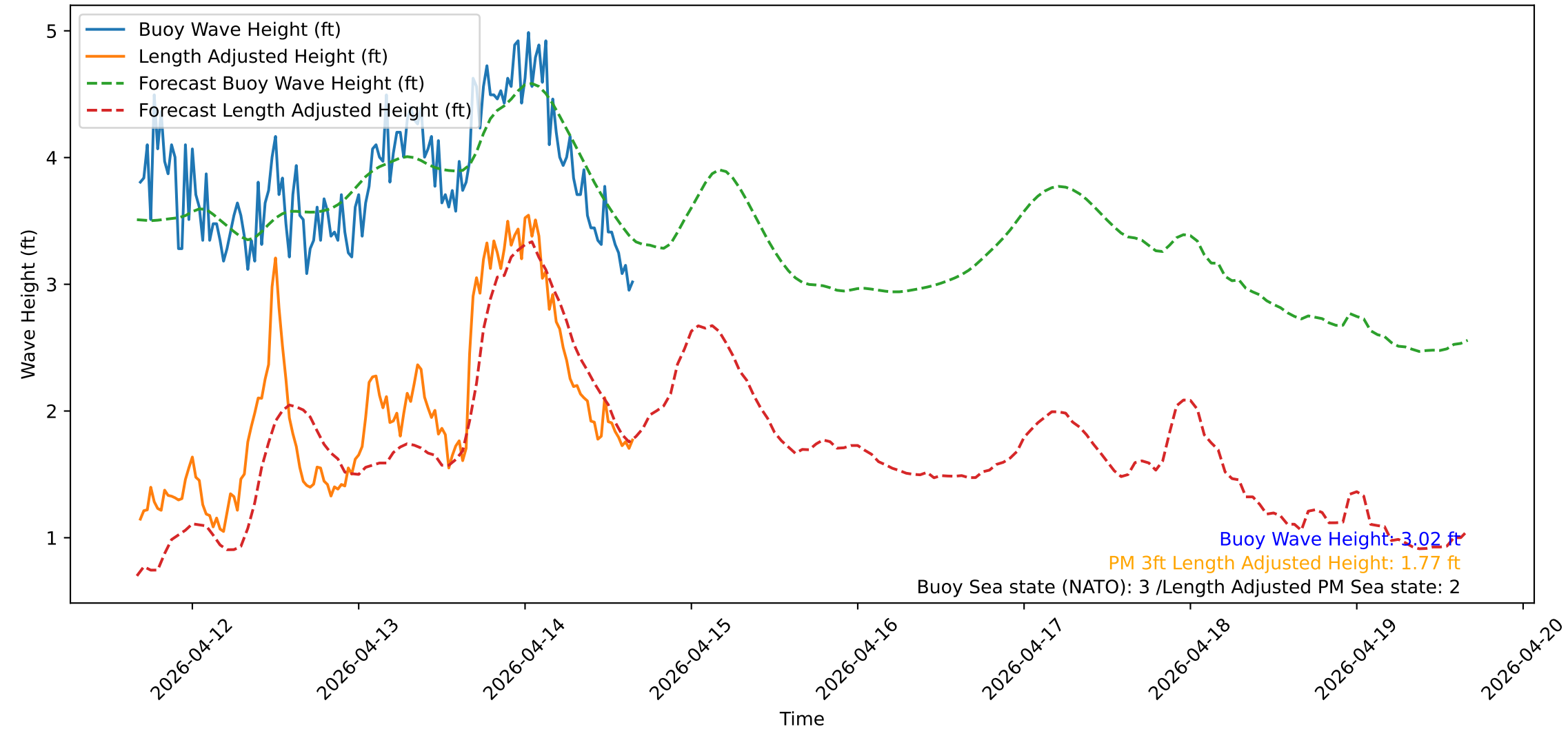
Wave Heights over Time for Green Beach at 2026-04-14 16:21:14
