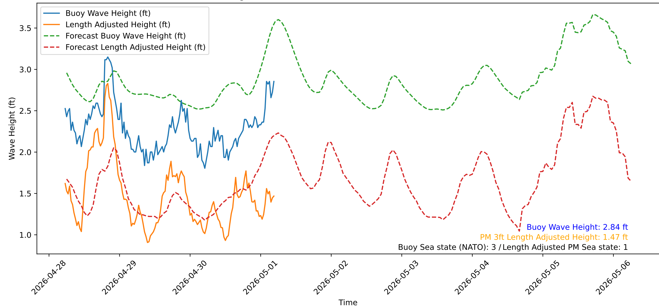
Wave Heights over Time for Green Beach at 2026-05-01 05:31:14
