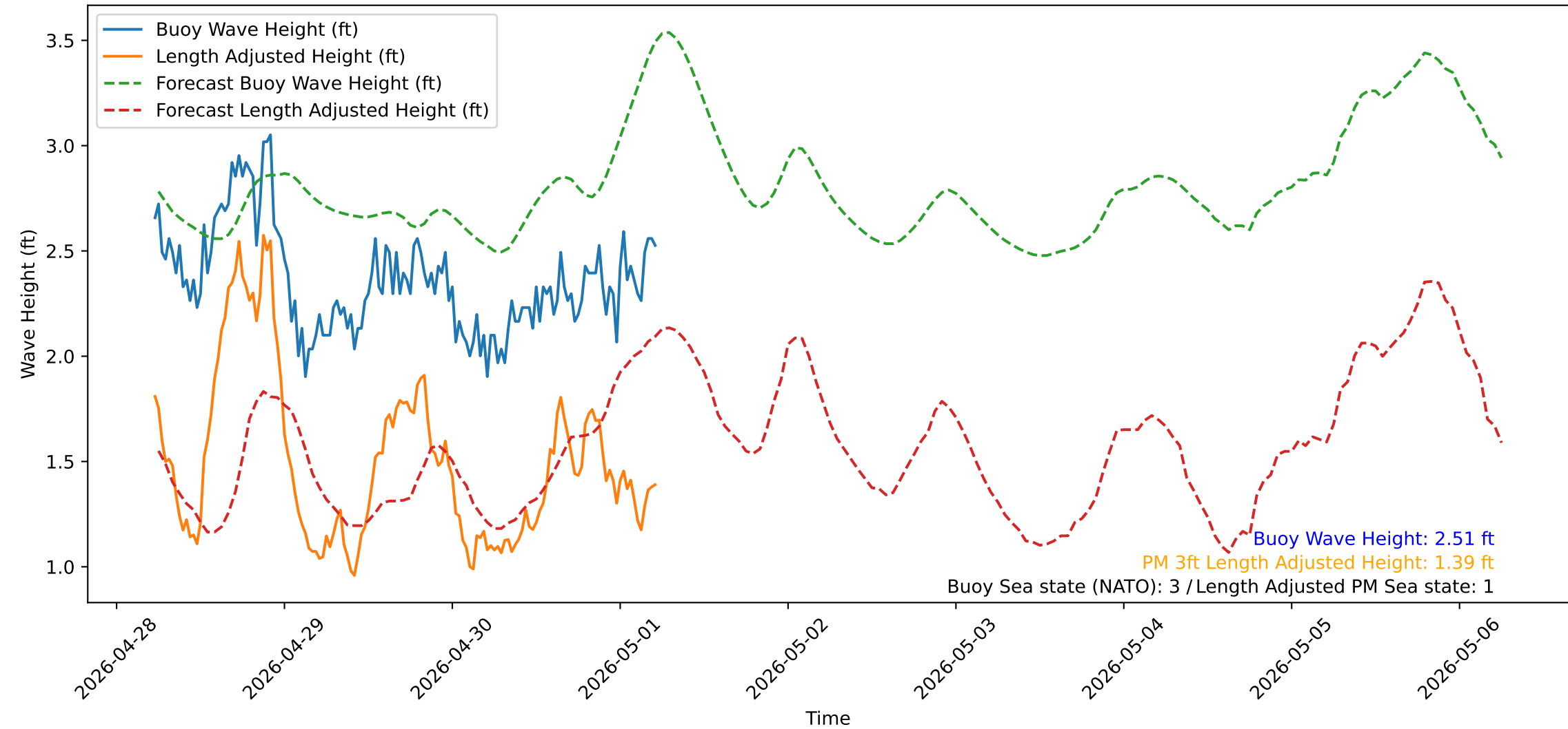
Wave Heights over Time for Oceanside Harbor at 2026-05-01 05:30:32
