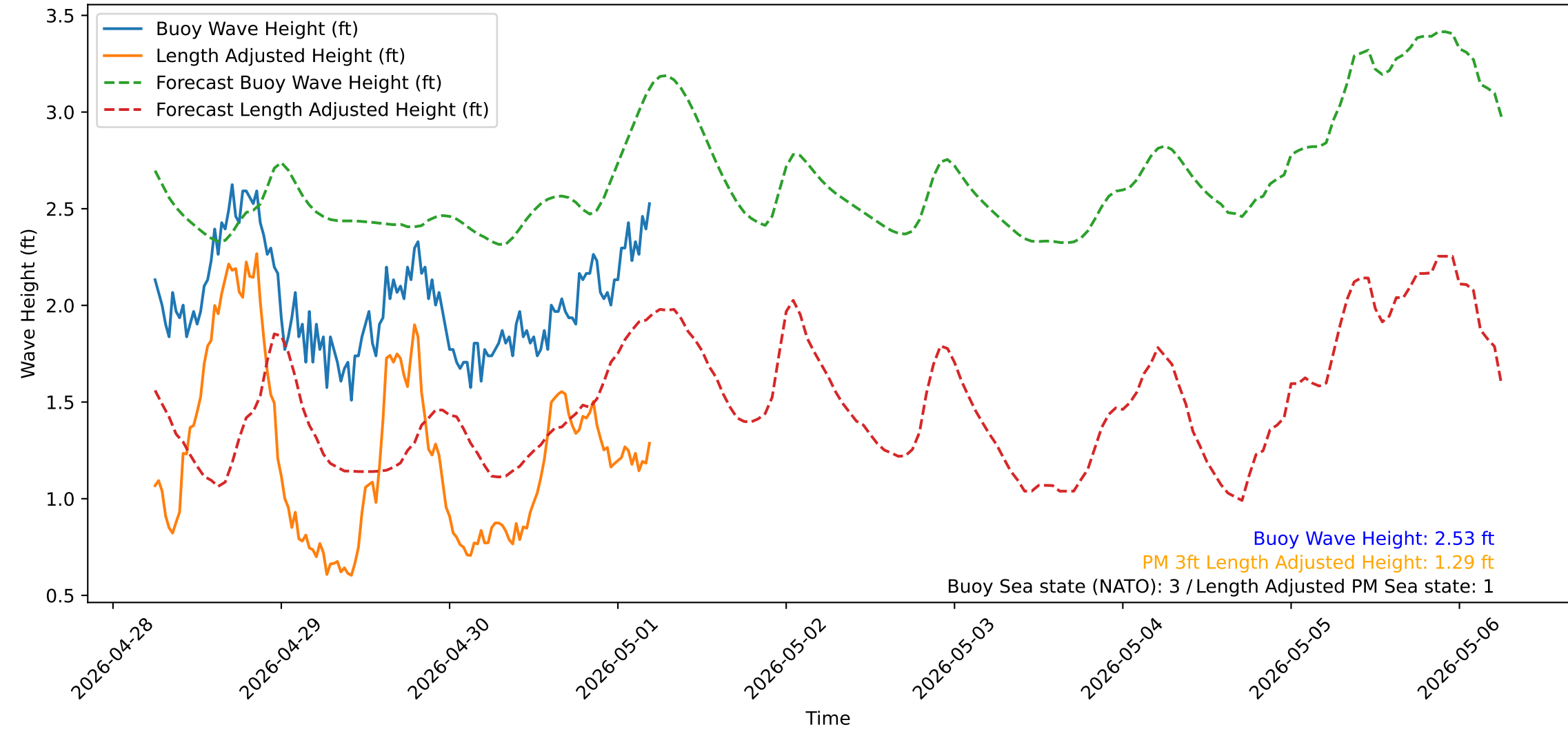
Wave Heights over Time for Red Beach at 2026-05-01 05:30:51
