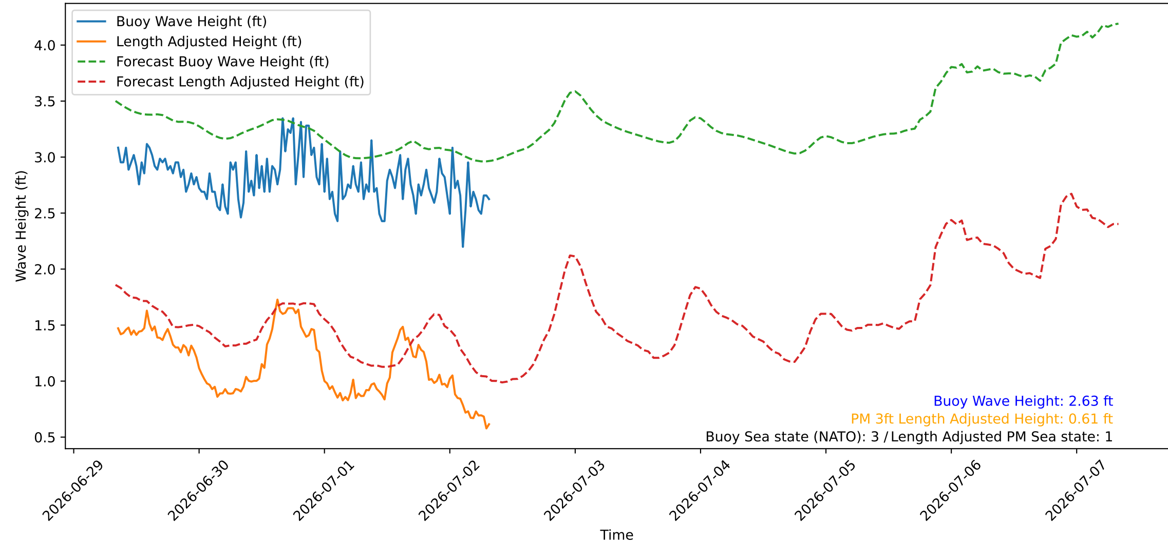
Wave Heights over Time for Red Beach at 2026-07-02 08:20:47
