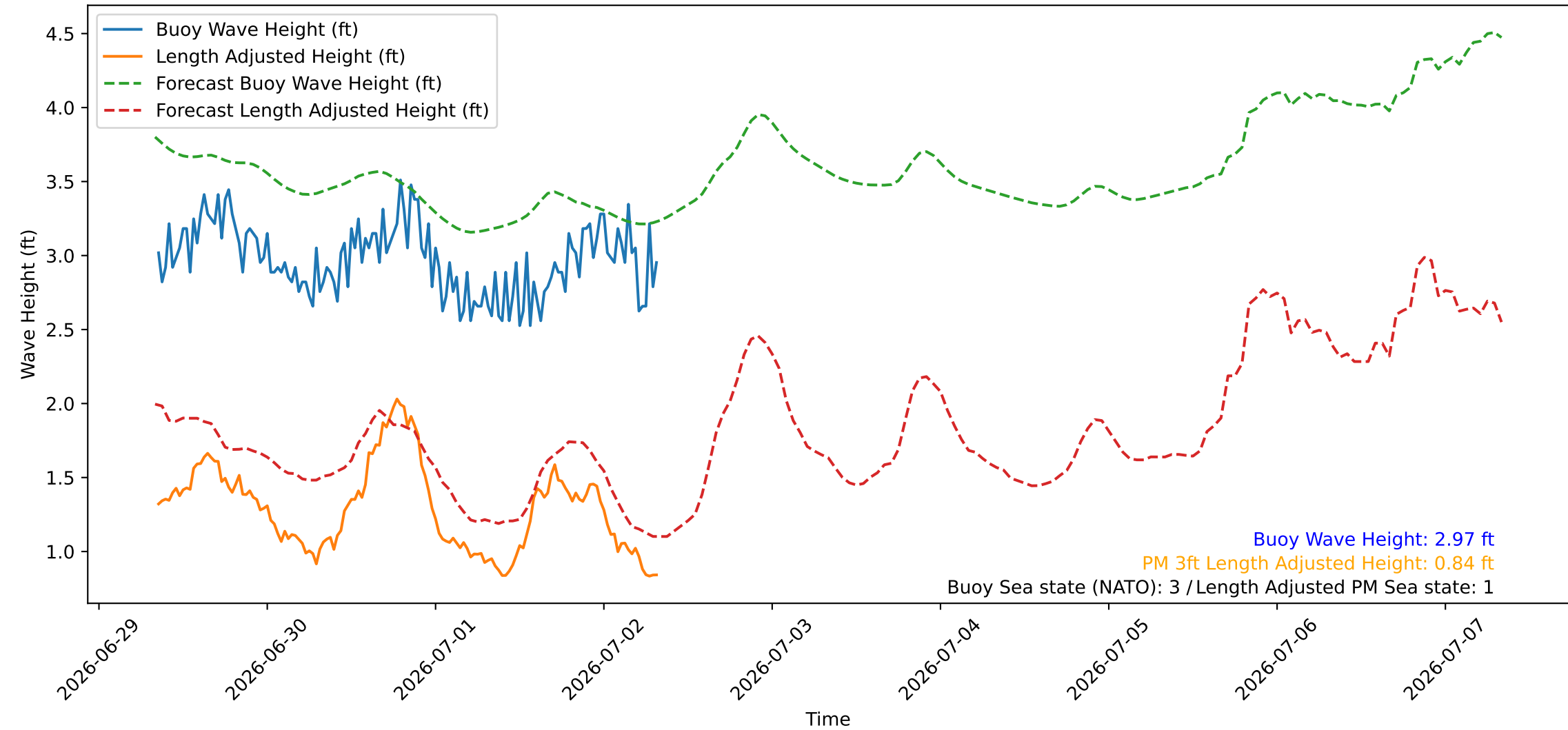
Wave Heights over Time for Green Beach at 2026-07-02 08:21:10
