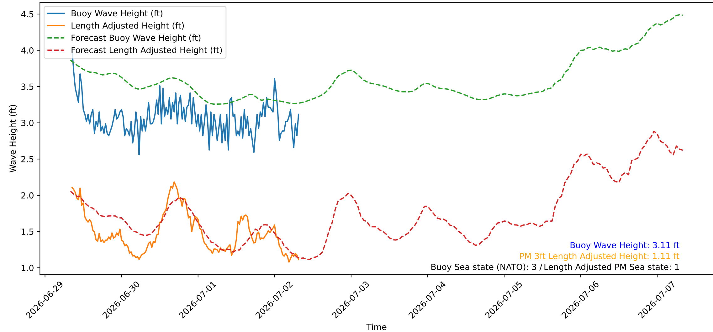
Wave Heights over Time for Oceanside Harbor at 2026-07-02 08:20:27
