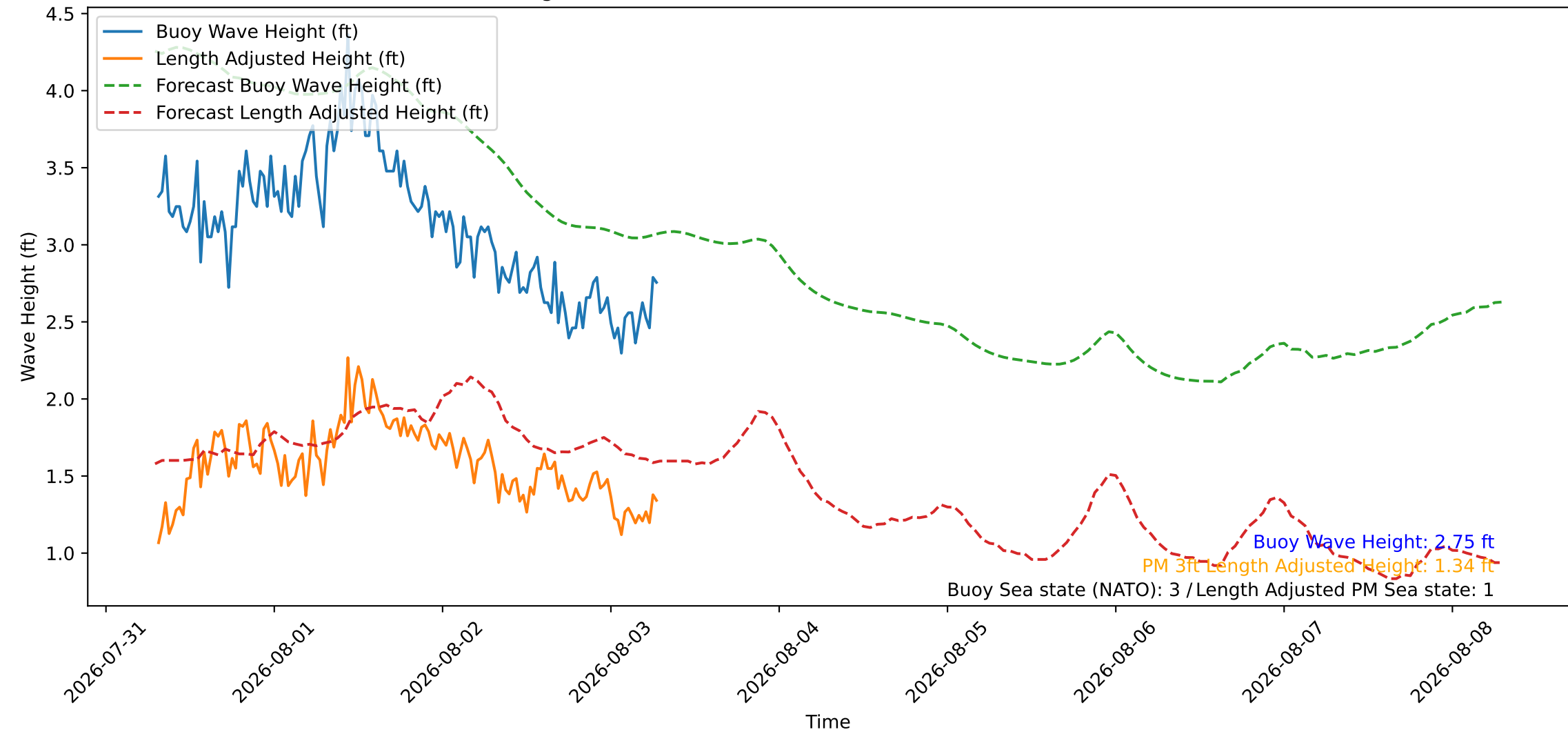
Wave Heights over Time for Oceanside Harbor at 2026-08-03 07:20:26
