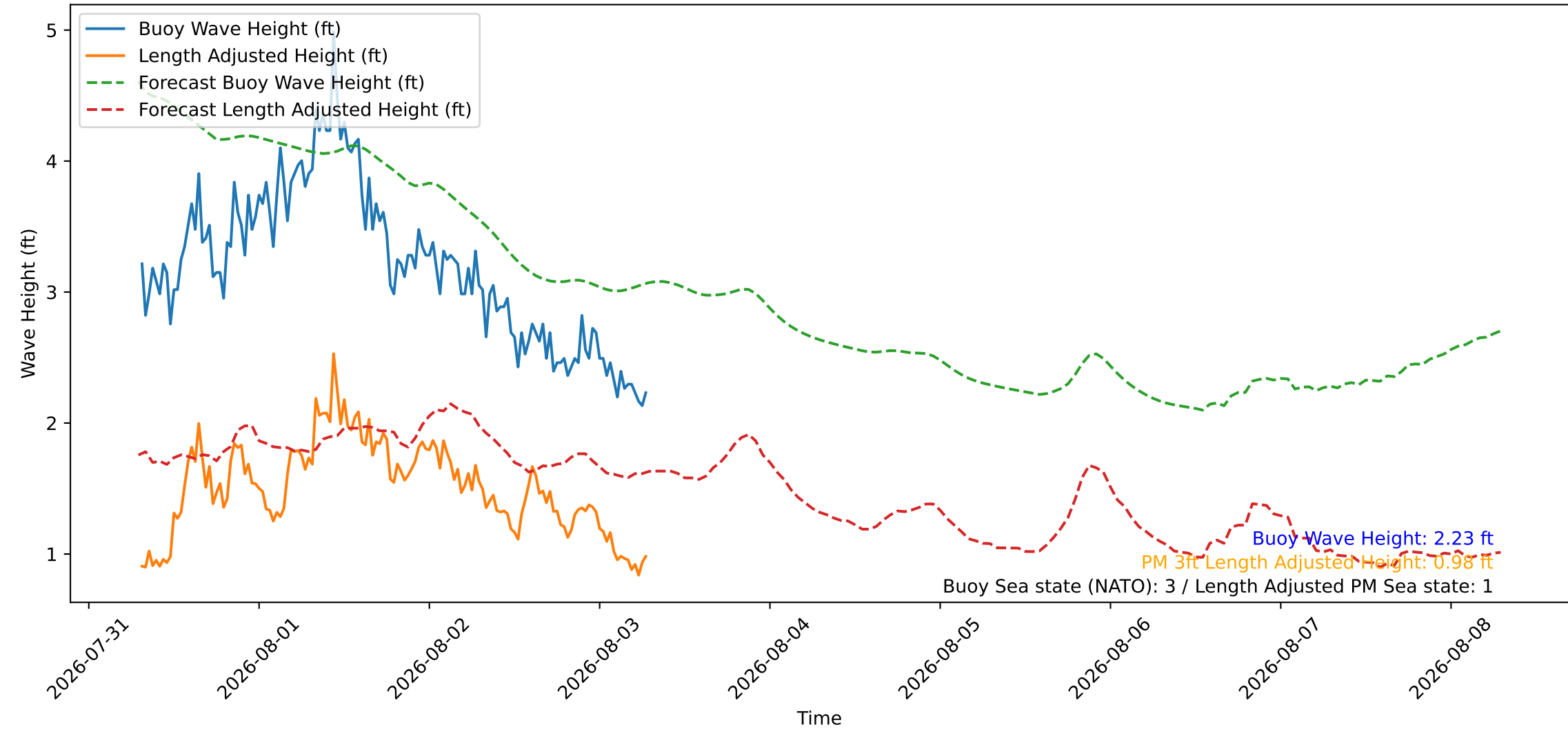
Wave Heights over Time for Green Beach at 2026-08-03 07:21:10
