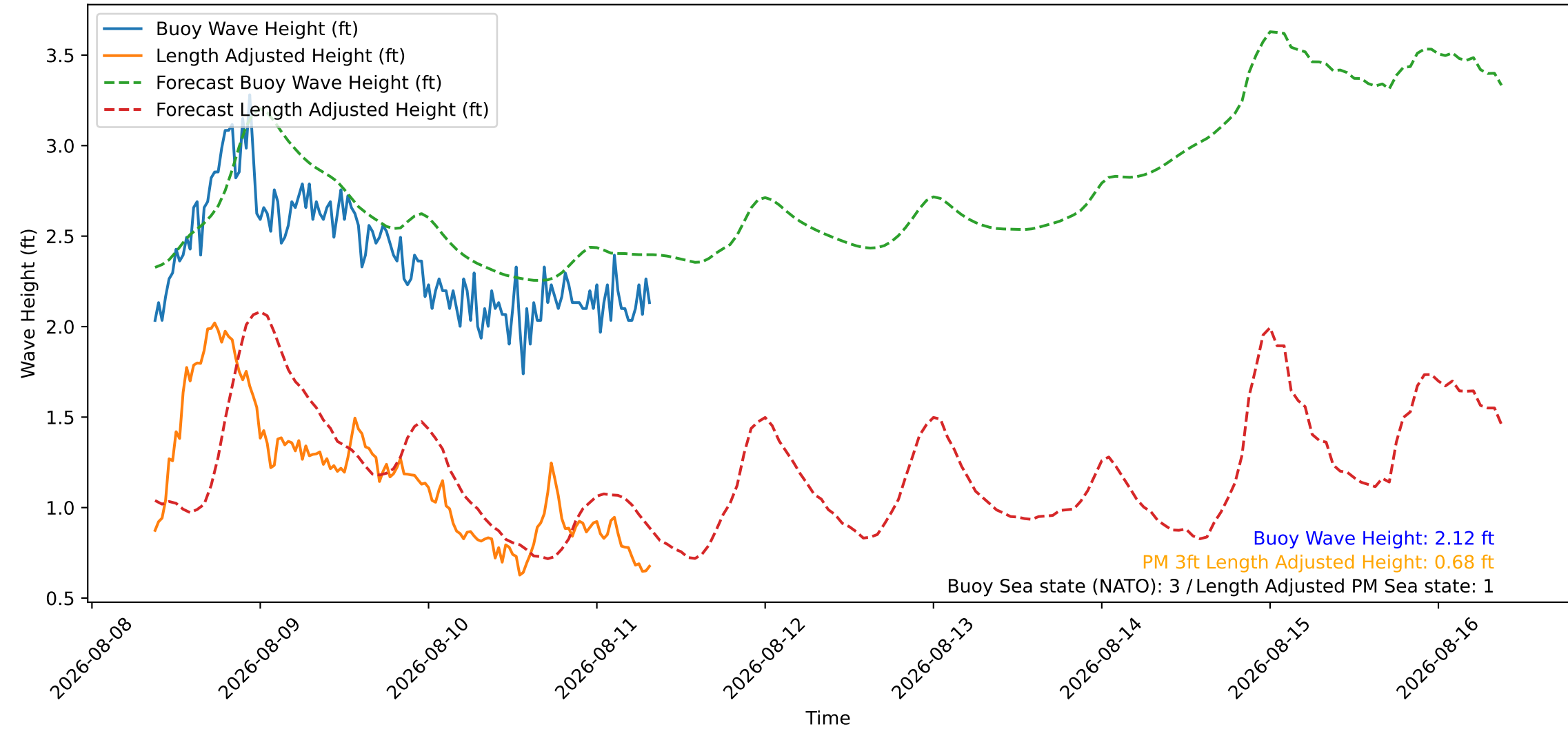
Wave Heights over Time for Red Beach at 2026-08-11 08:40:46
