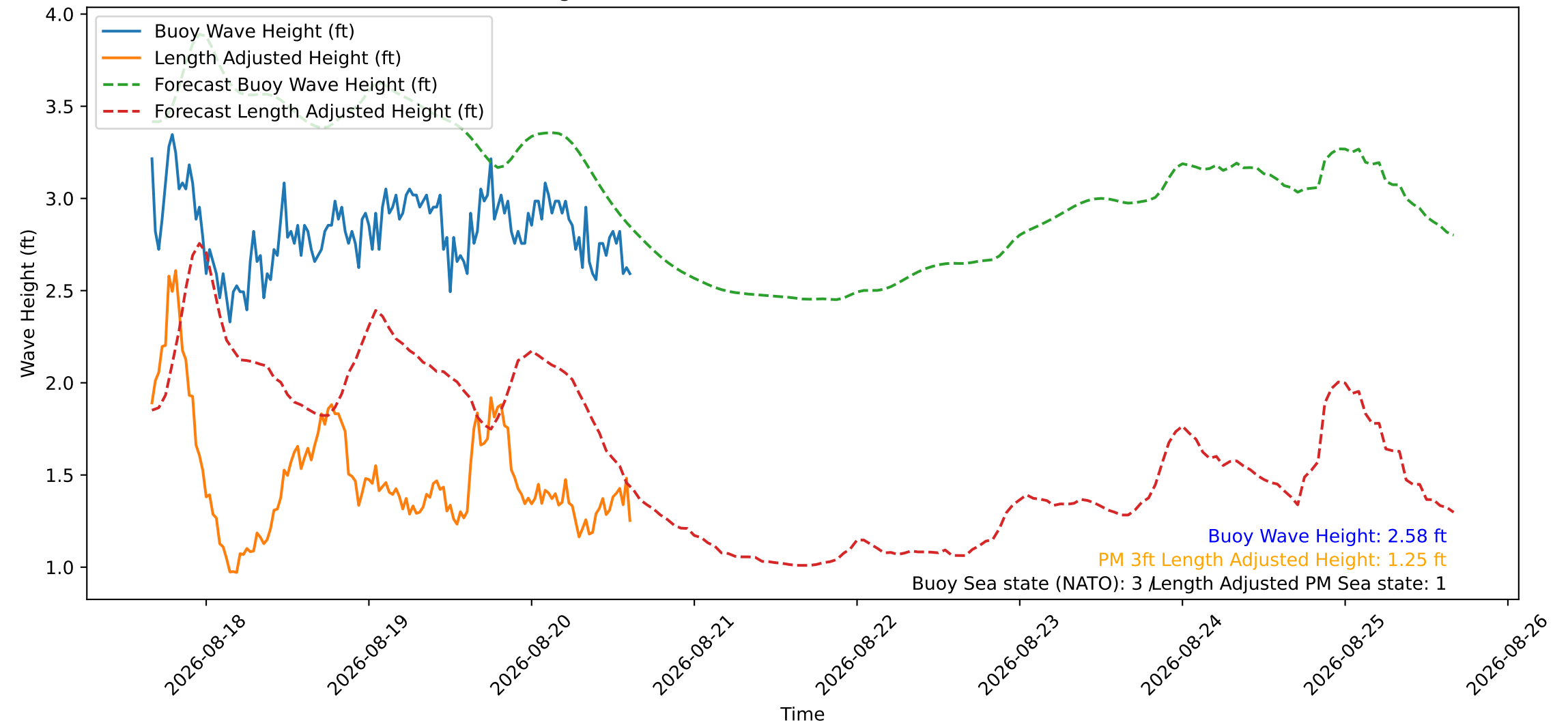
Wave Heights over Time for Red Beach at 2026-08-20 15:30:46
