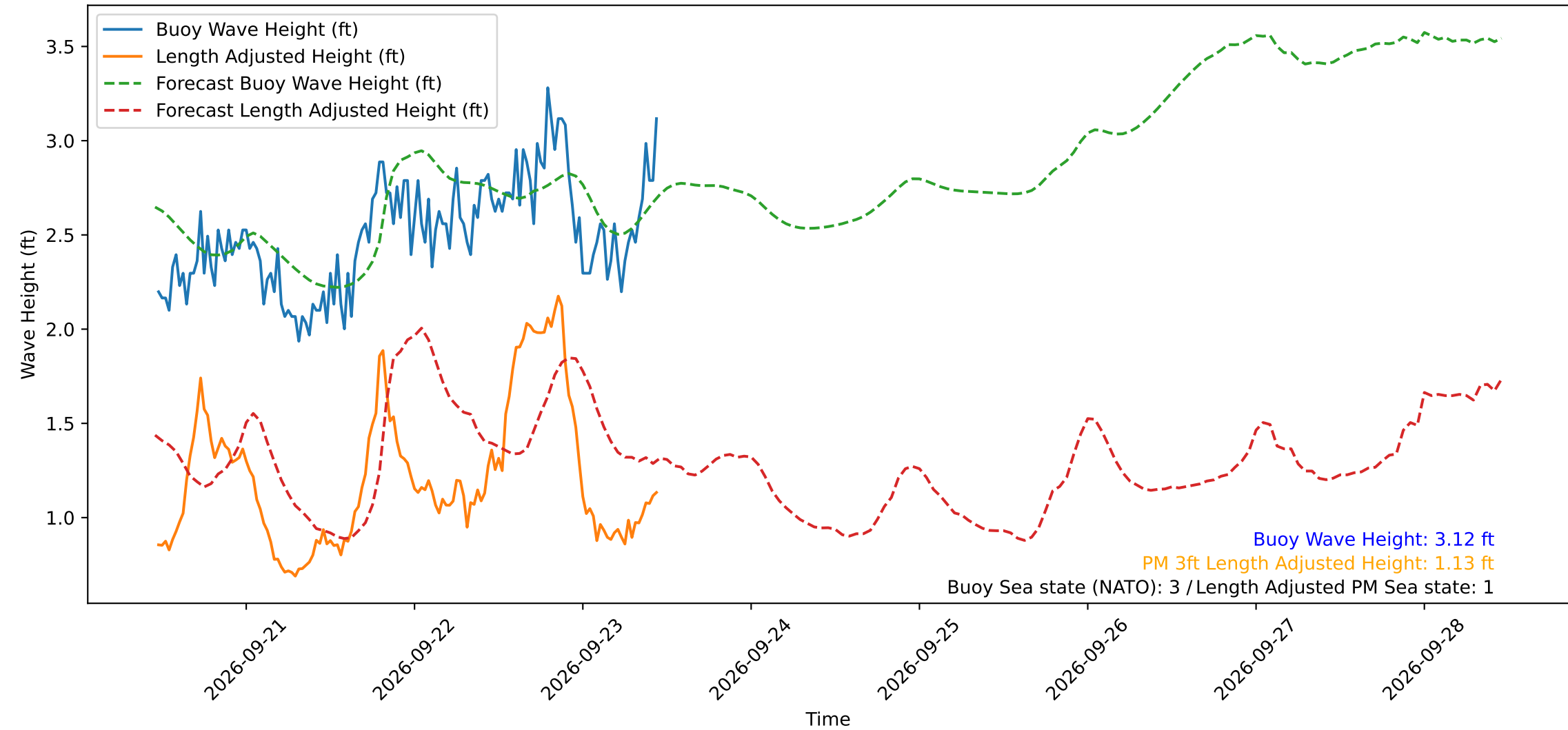
Wave Heights over Time for Red Beach at 2026-09-23 11:10:50
