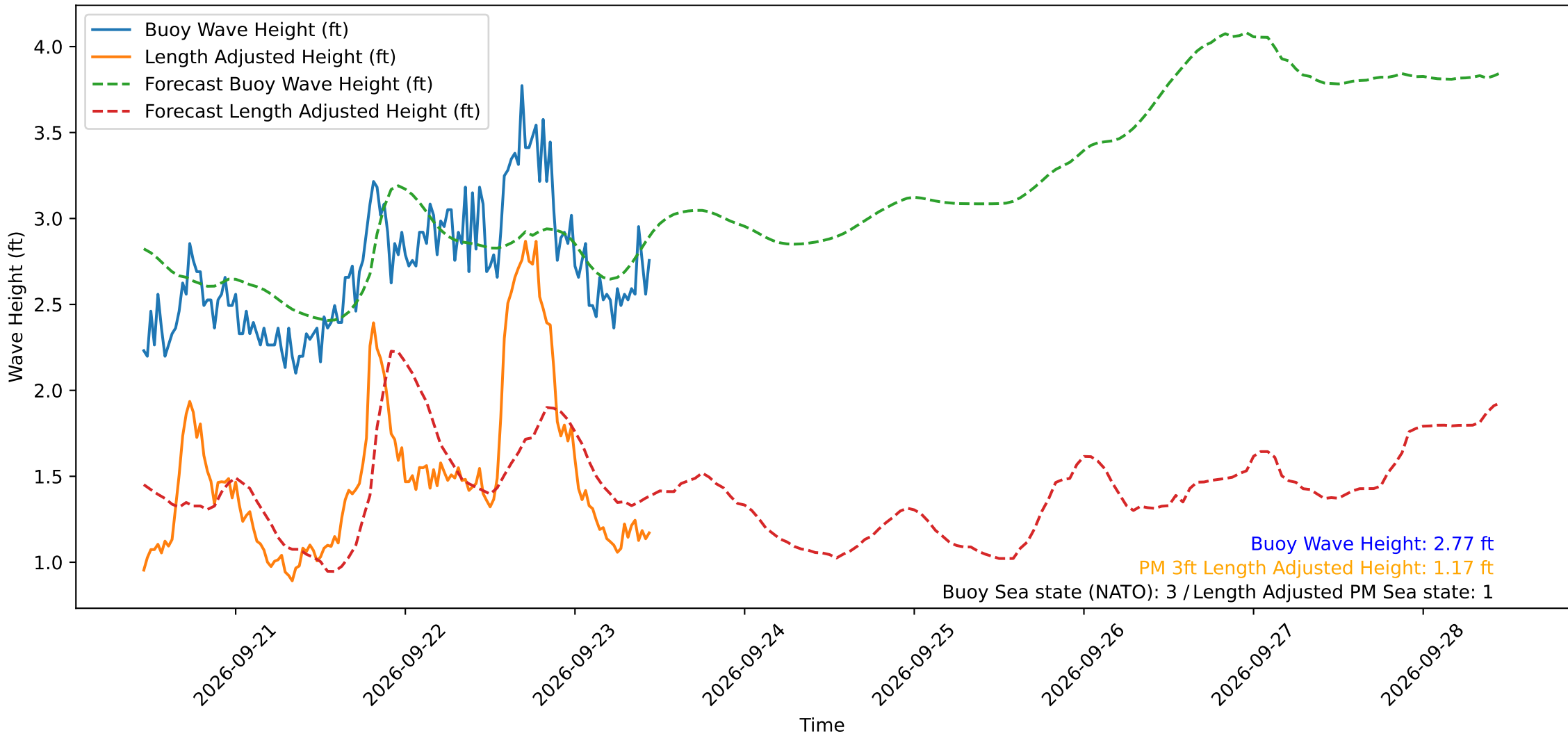
Wave Heights over Time for Oceanside Harbor at 2026-09-23 11:10:30
