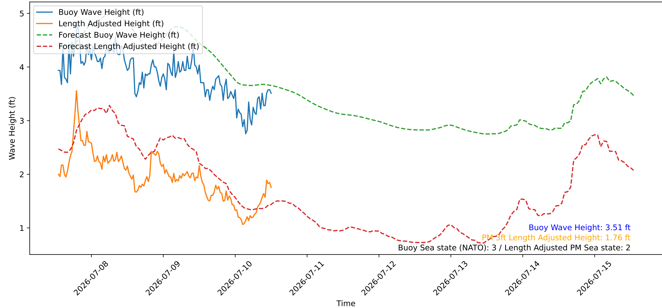
Wave Heights over Time for Green Beach at 2026-07-10 13:01:07
