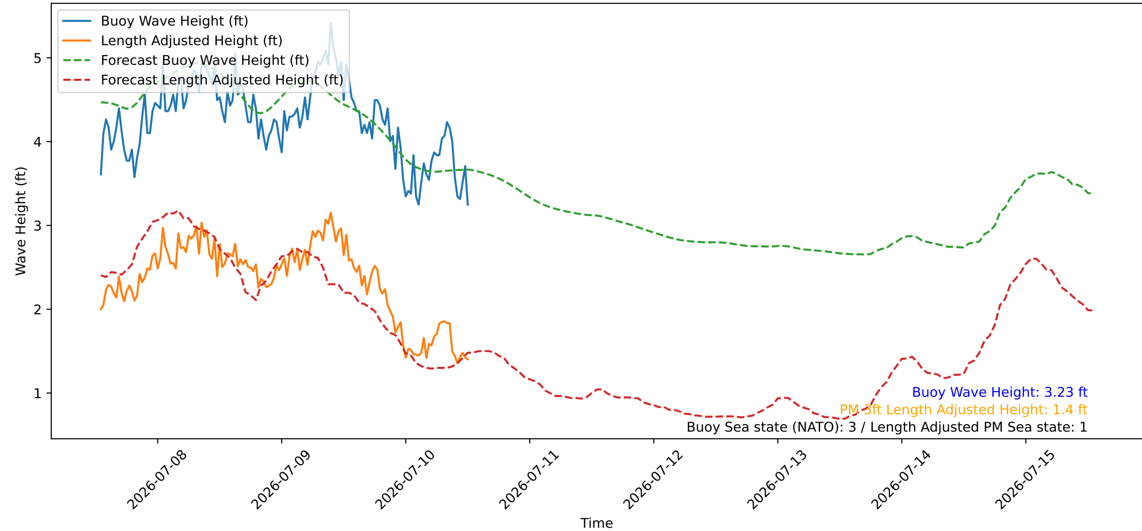
Wave Heights over Time for Oceanside Harbor at 2026-07-10 13:00:26
