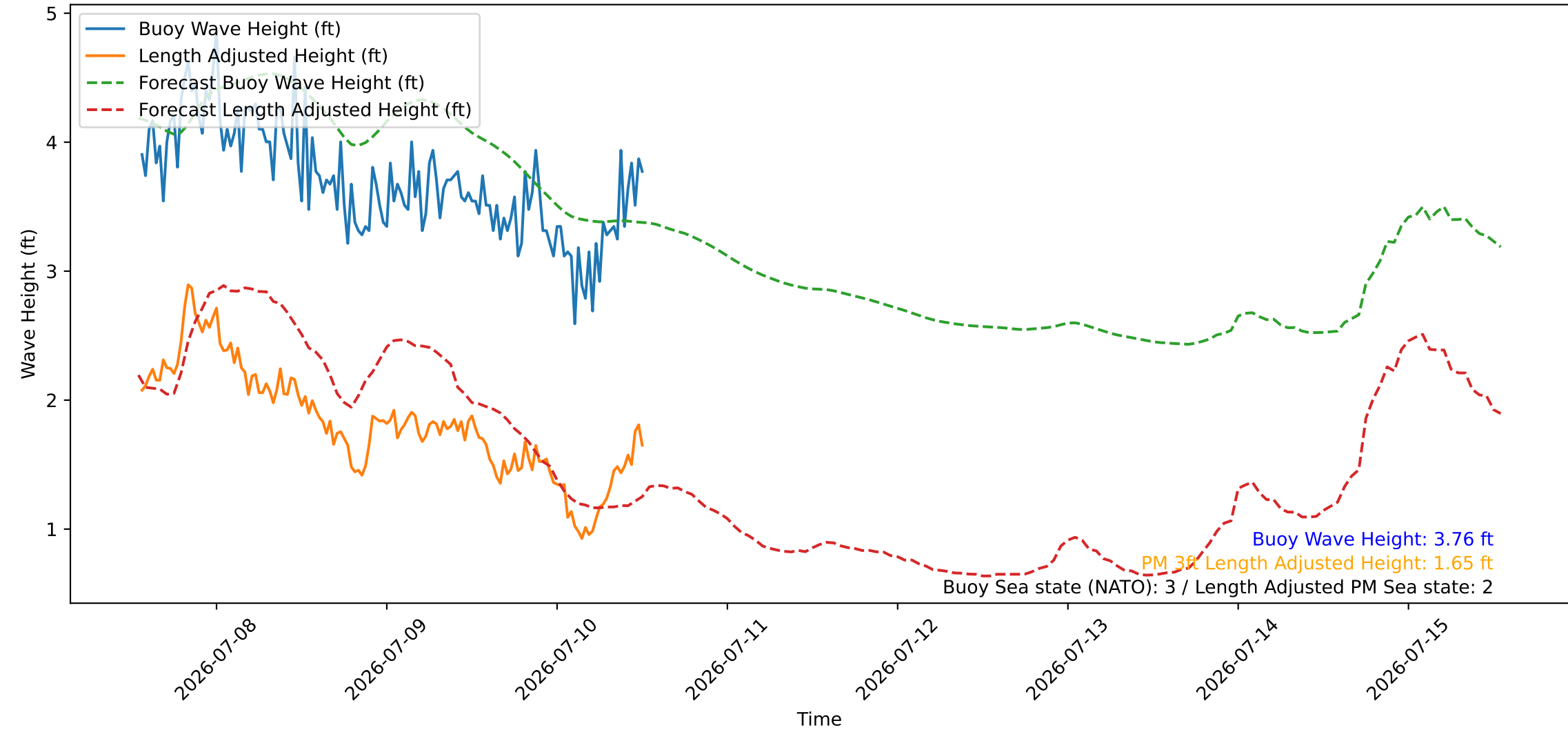
Wave Heights over Time for Red Beach at 2026-07-10 13:00:45
