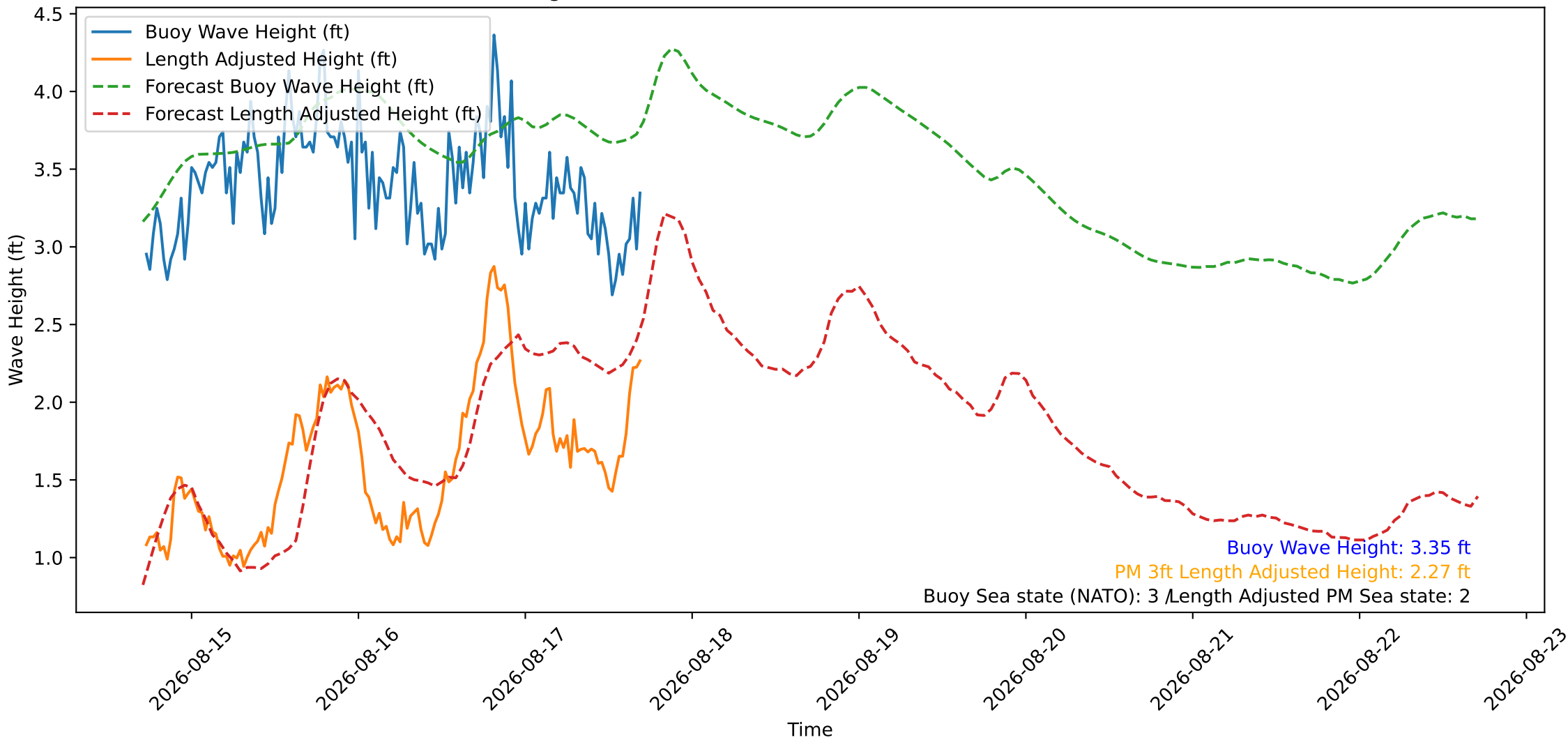
Wave Heights over Time for Green Beach at 2026-08-17 17:21:11
