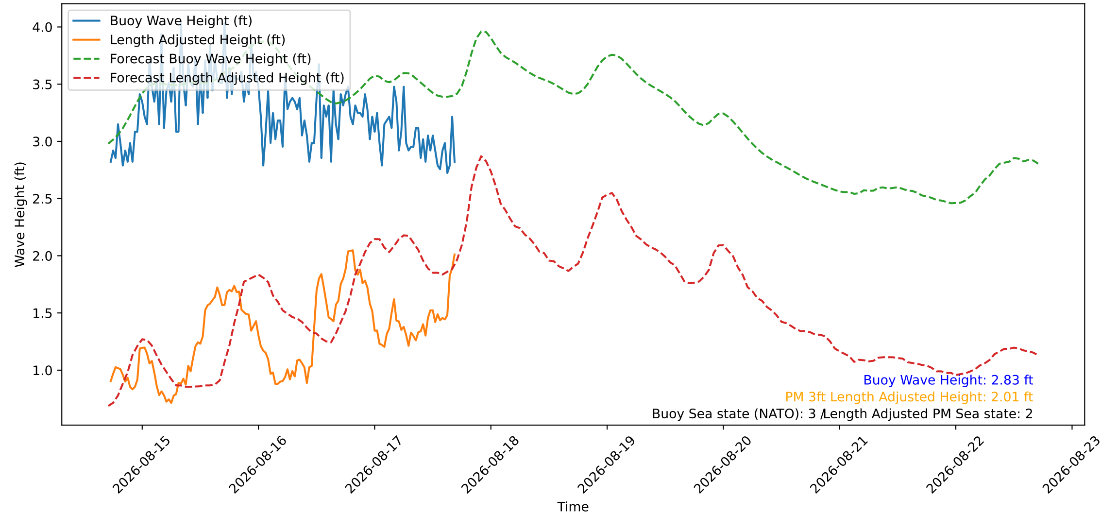
Wave Heights over Time for Red Beach at 2026-08-17 17:20:47
