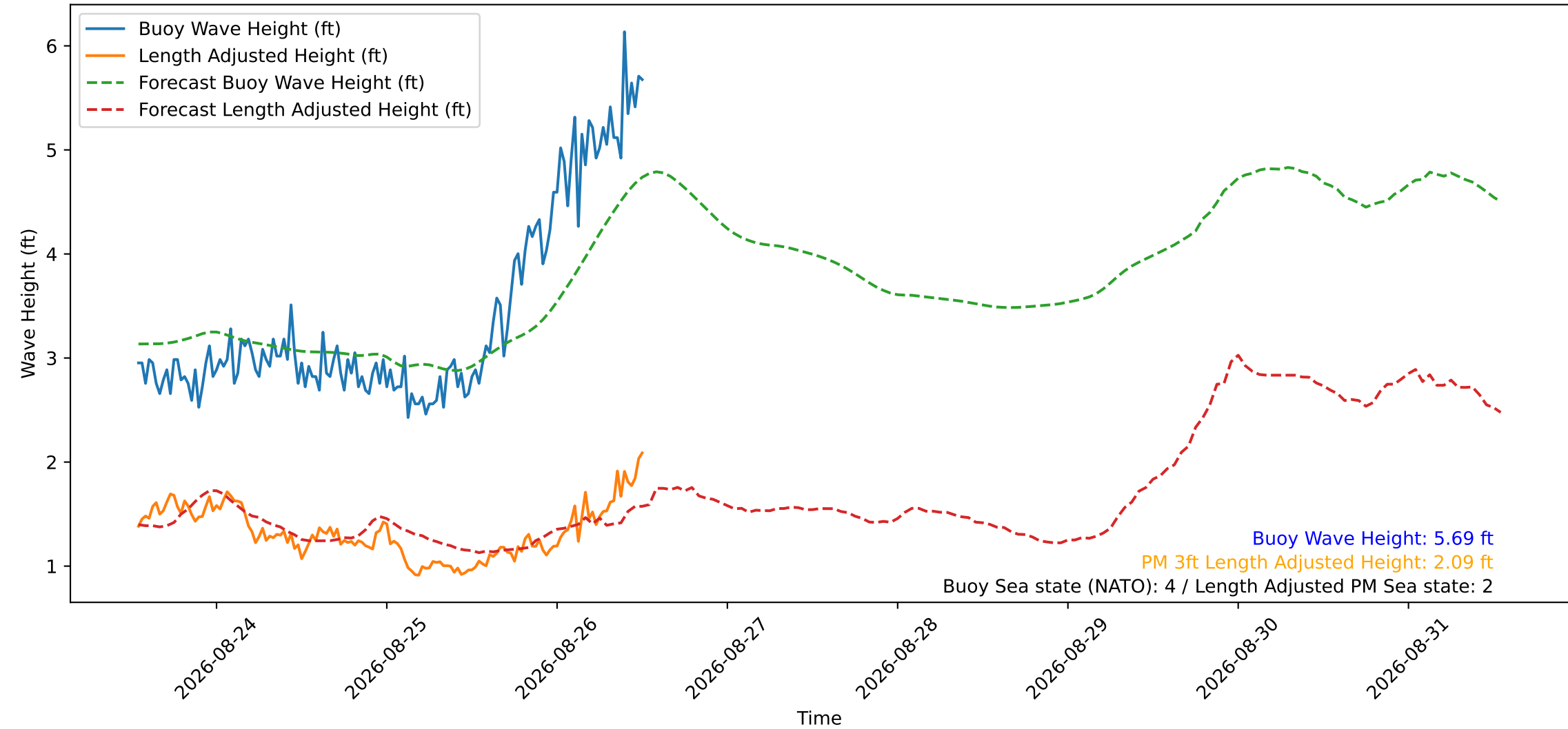
Wave Heights over Time for Oceanside Harbor at 2026-08-26 12:50:29
