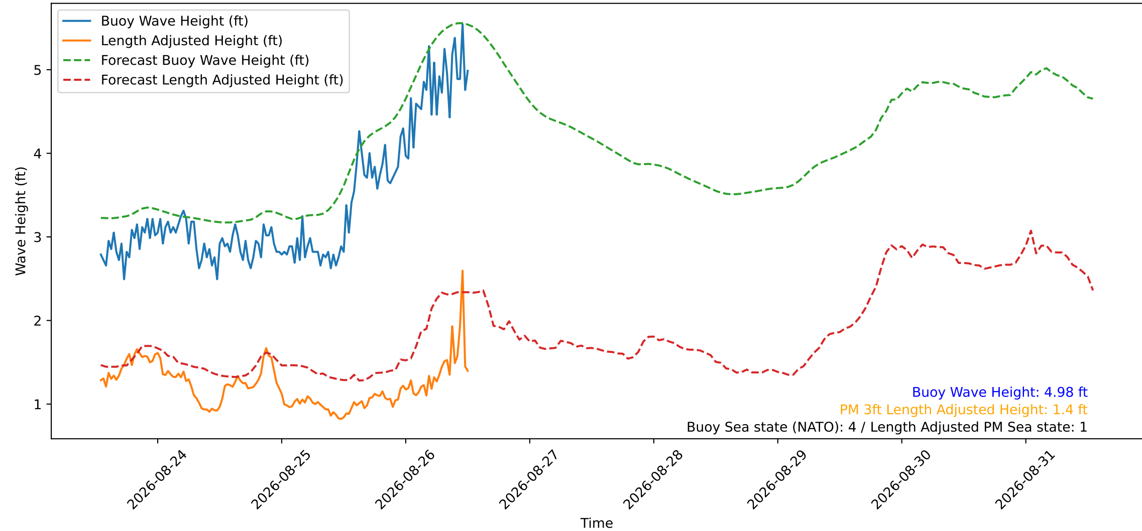
Wave Heights over Time for Green Beach at 2026-08-26 12:51:15
