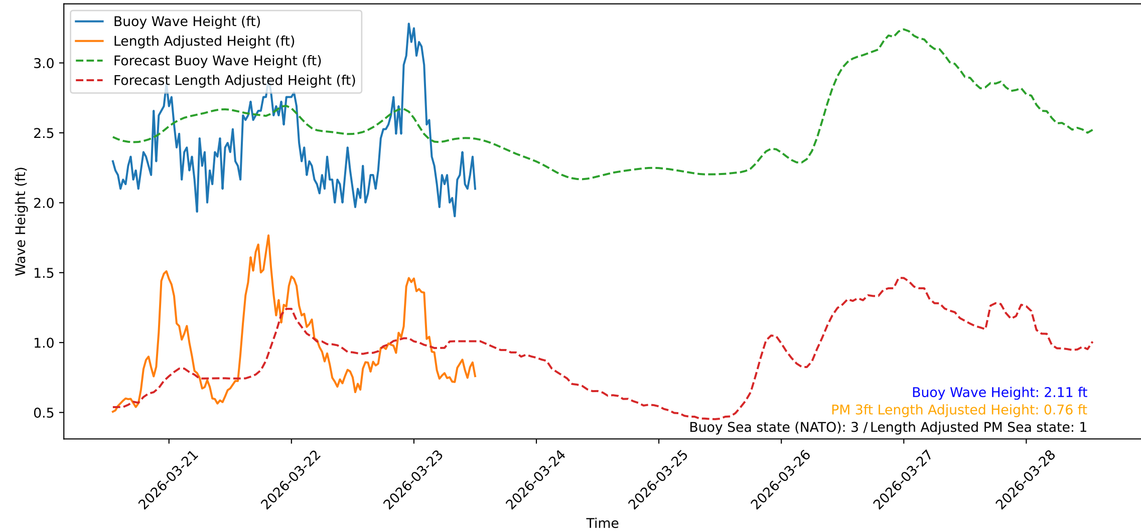
Wave Heights over Time for Green Beach at 2026-03-23 12:51:11
