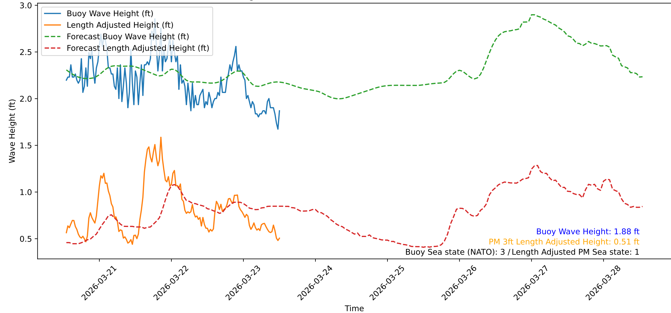
Wave Heights over Time for Red Beach at 2026-03-23 12:50:49
