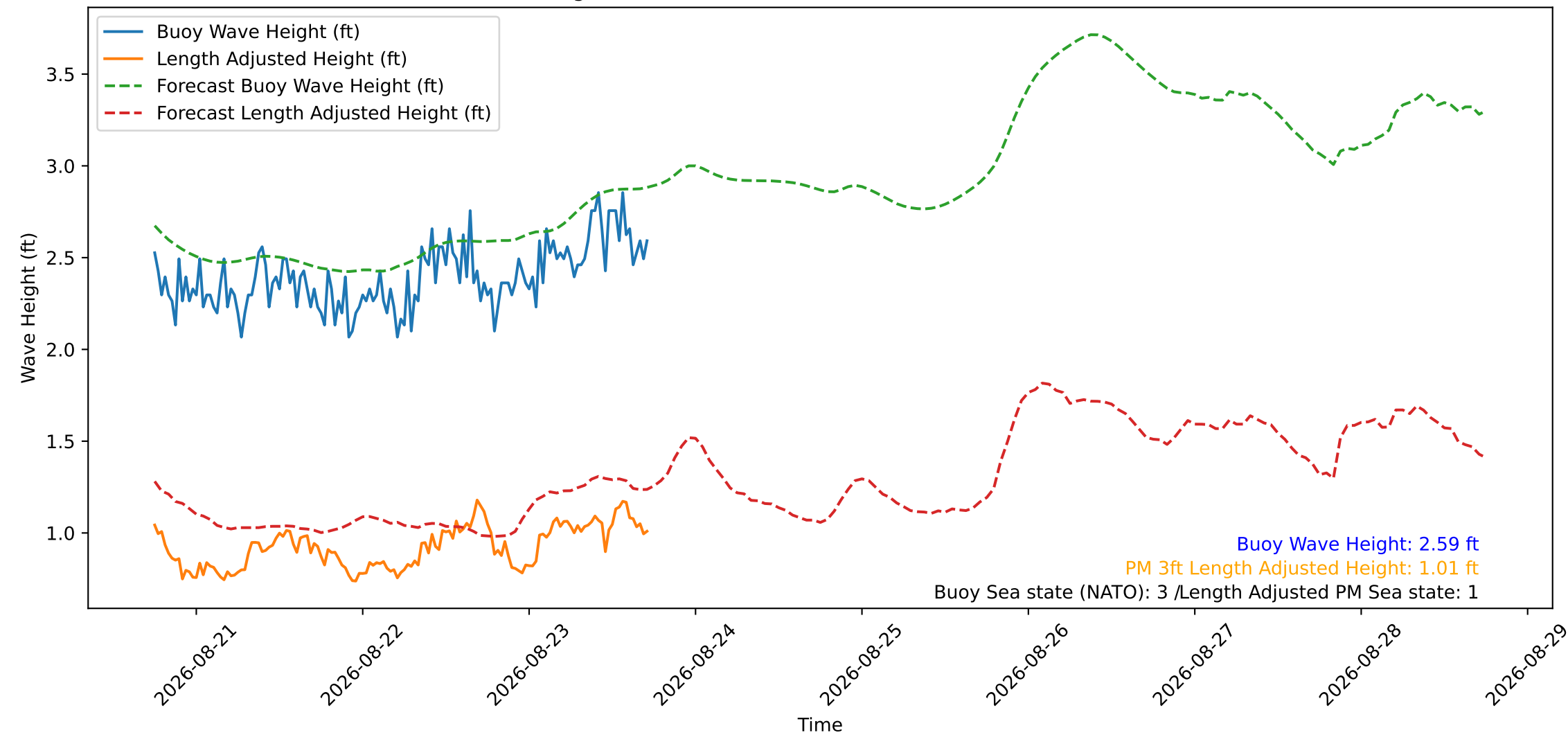
Wave Heights over Time for Red Beach at 2026-08-23 17:50:50
