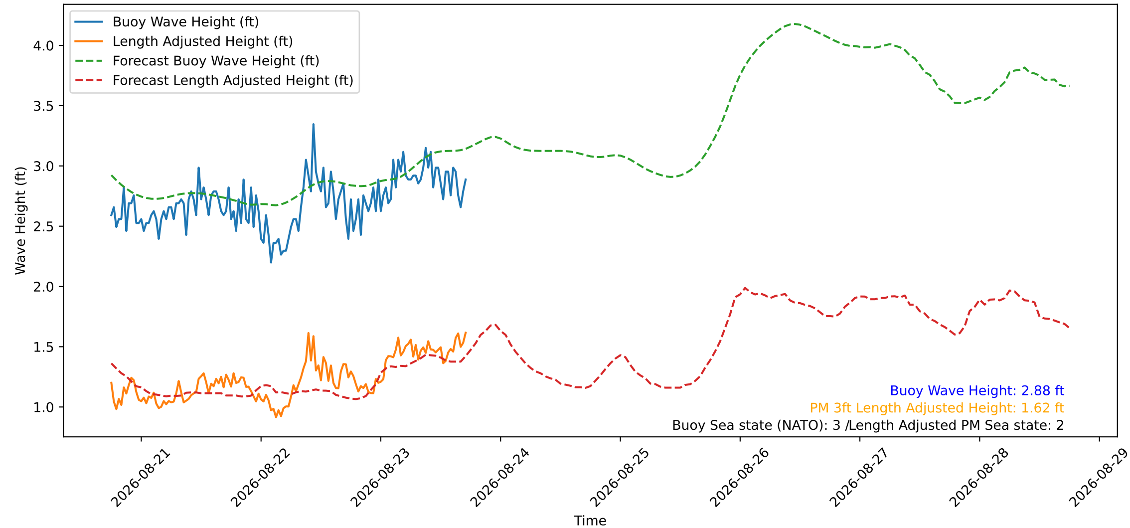
Wave Heights over Time for Oceanside Harbor at 2026-08-23 17:50:29
