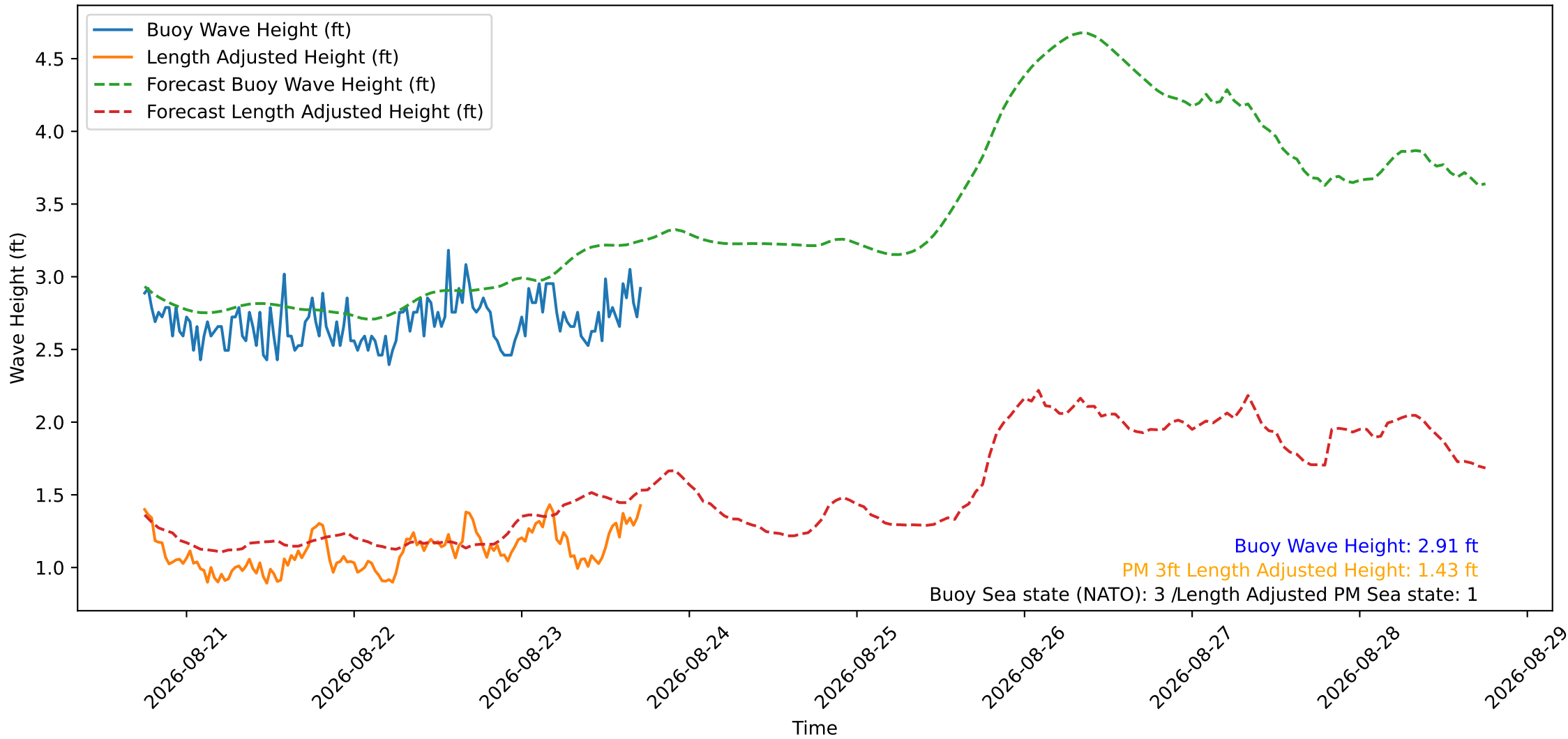
Wave Heights over Time for Green Beach at 2026-08-23 17:51:14
