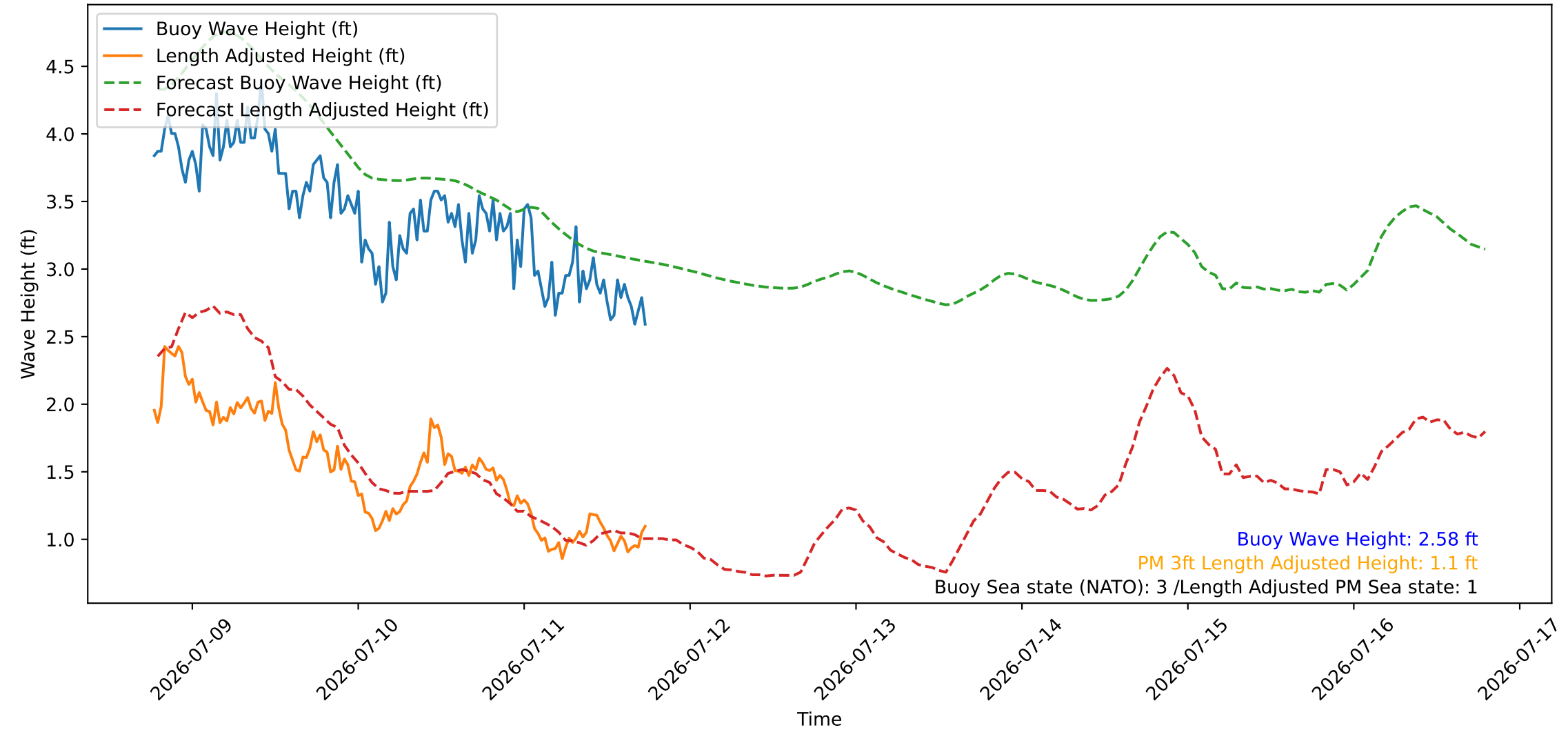
Wave Heights over Time for Green Beach at 2026-07-11 18:31:08
