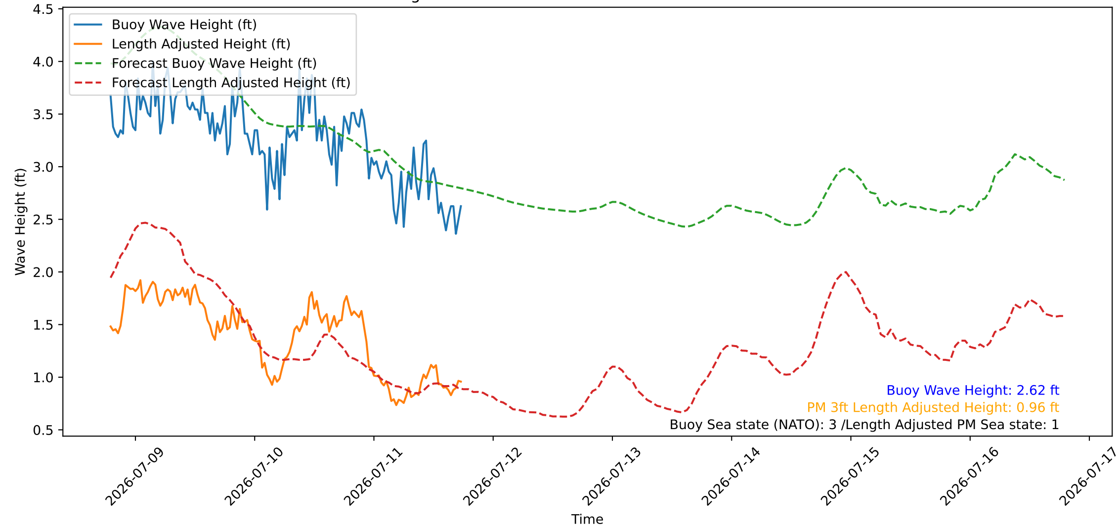
Wave Heights over Time for Red Beach at 2026-07-11 18:30:46
