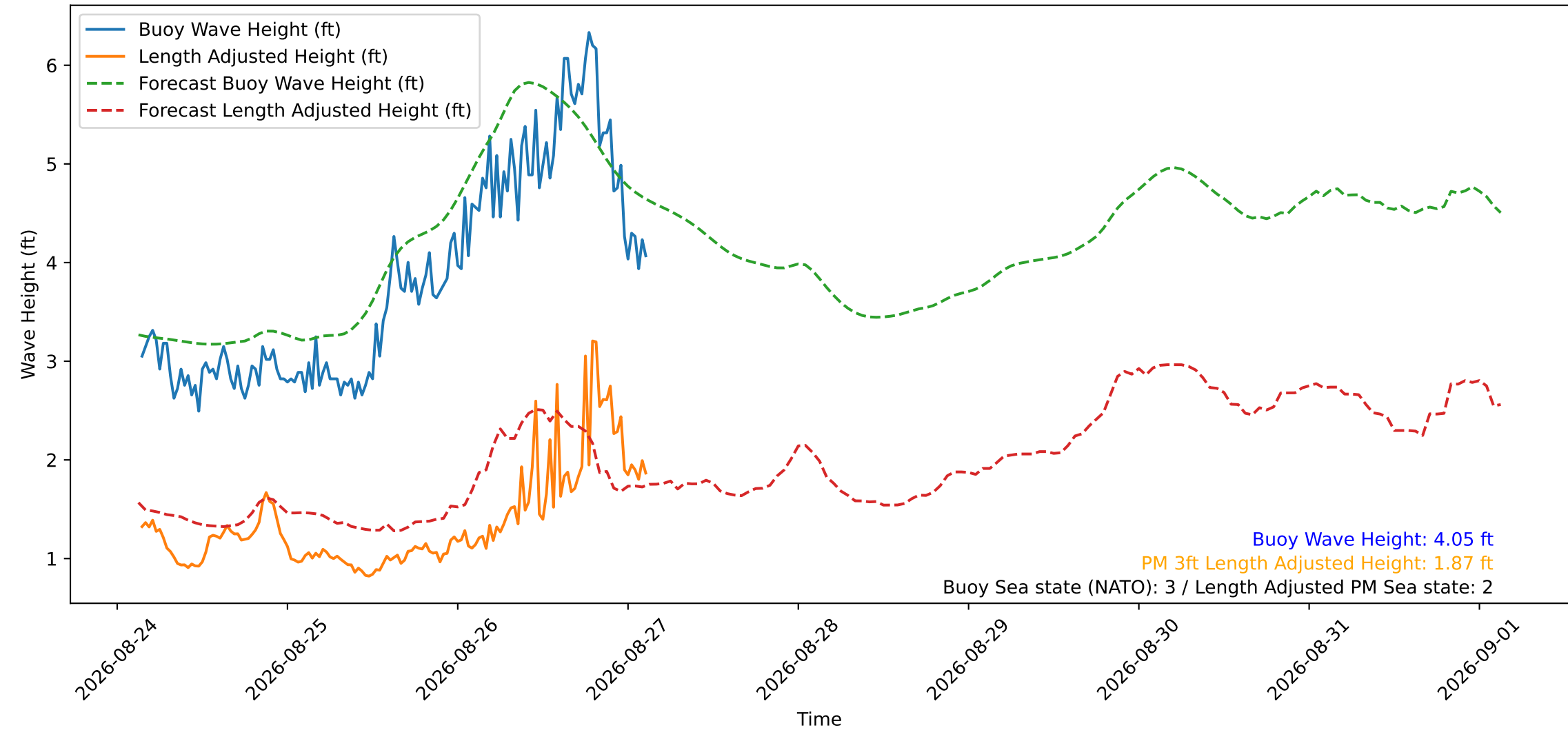
Wave Heights over Time for Green Beach at 2026-08-27 03:11:13
