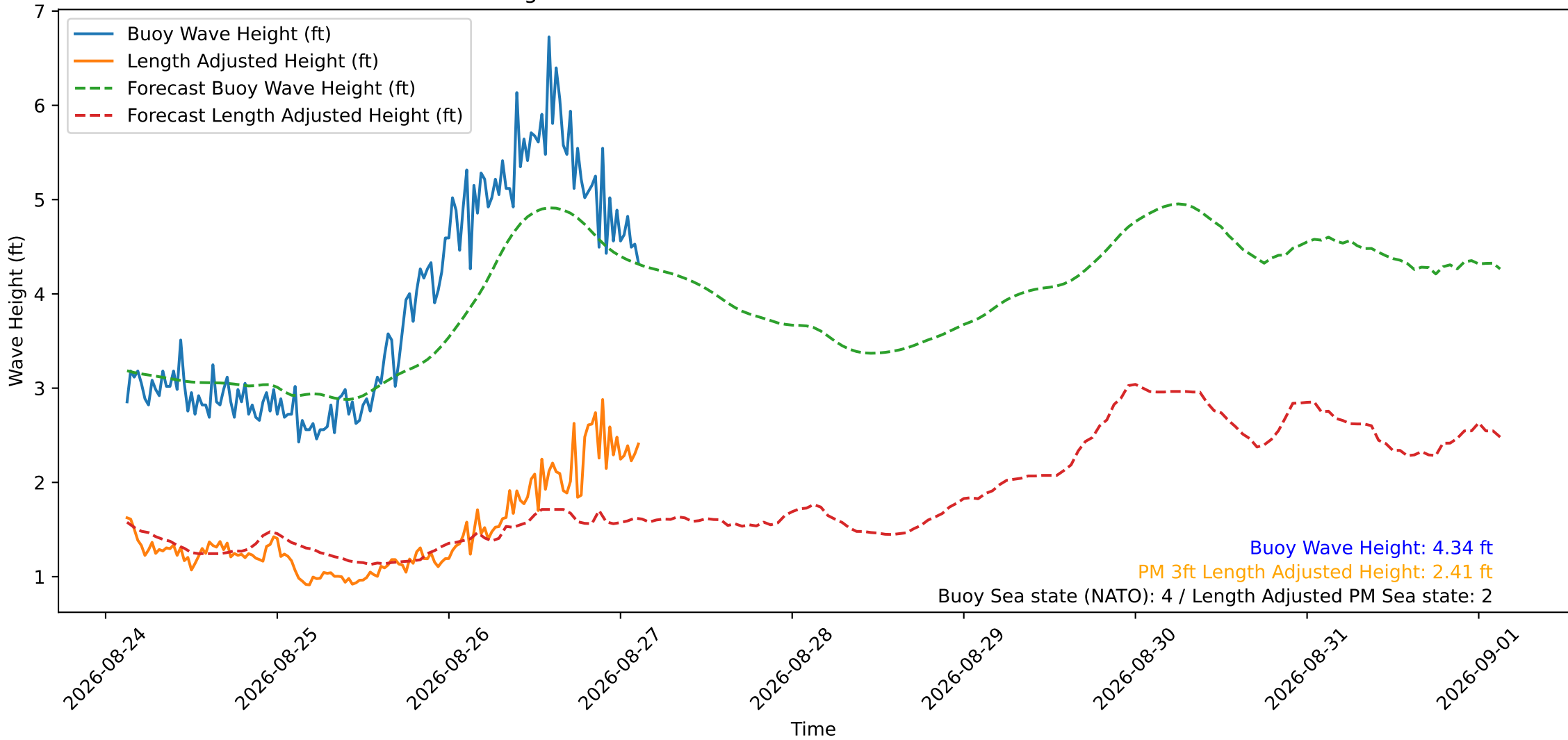
Wave Heights over Time for Oceanside Harbor at 2026-08-27 03:10:30
