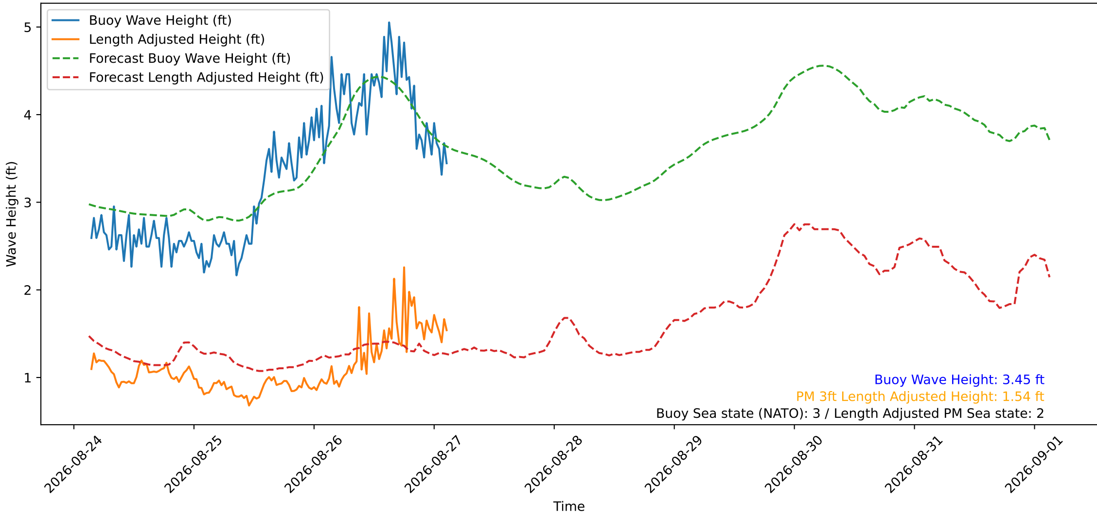
Wave Heights over Time for Red Beach at 2026-08-27 03:10:50
