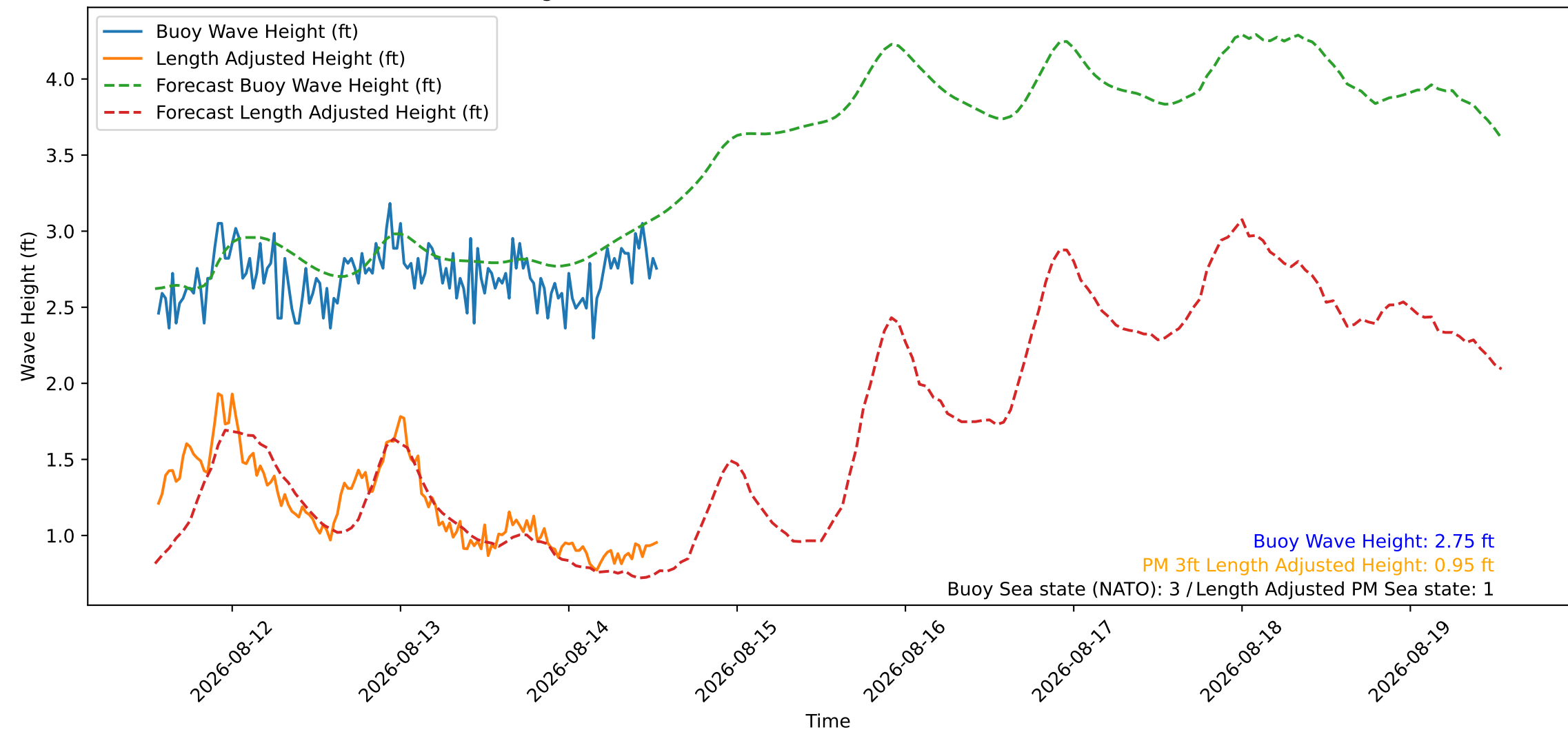
Wave Heights over Time for Oceanside Harbor at 2026-08-14 13:20:26
