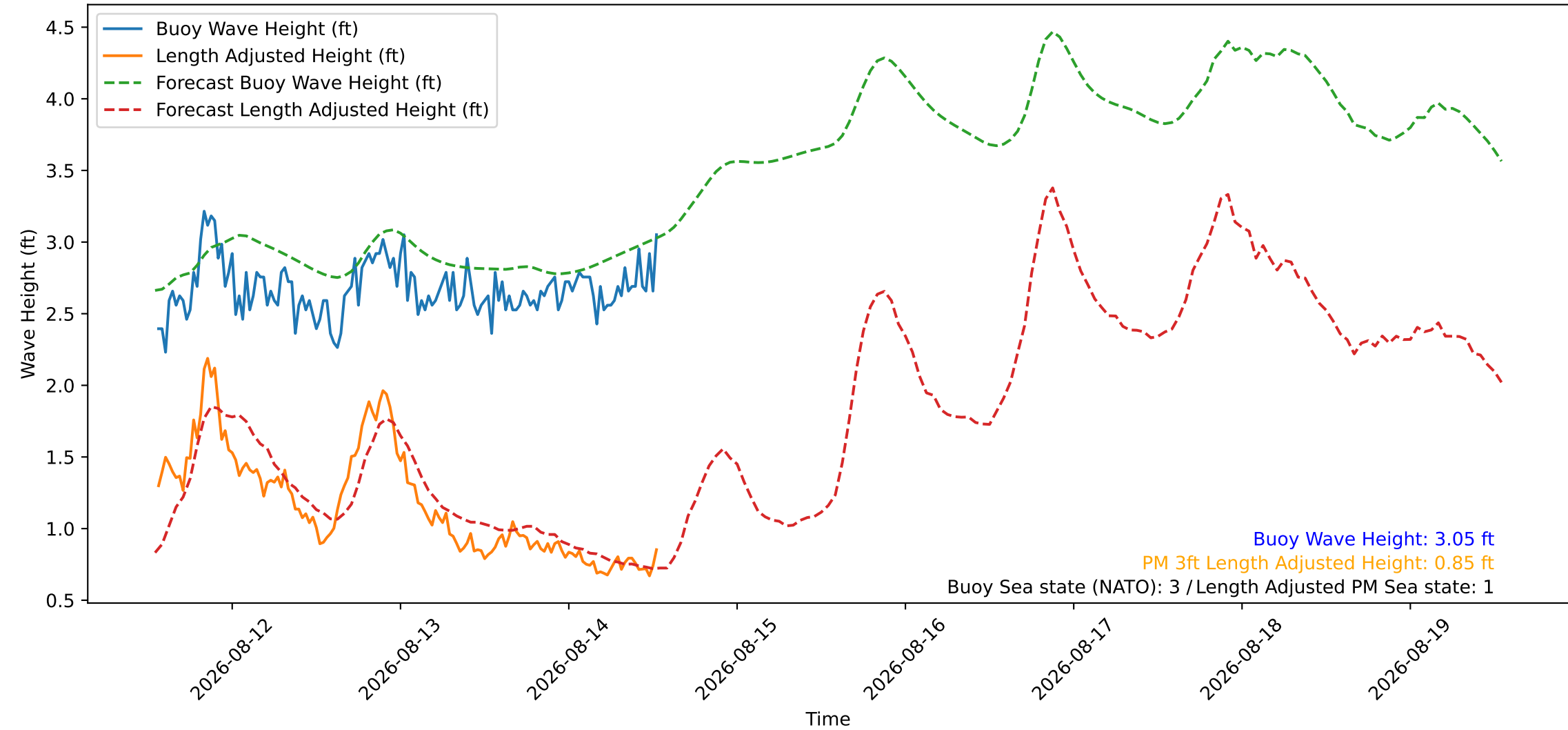
Wave Heights over Time for Green Beach at 2026-08-14 13:21:09
