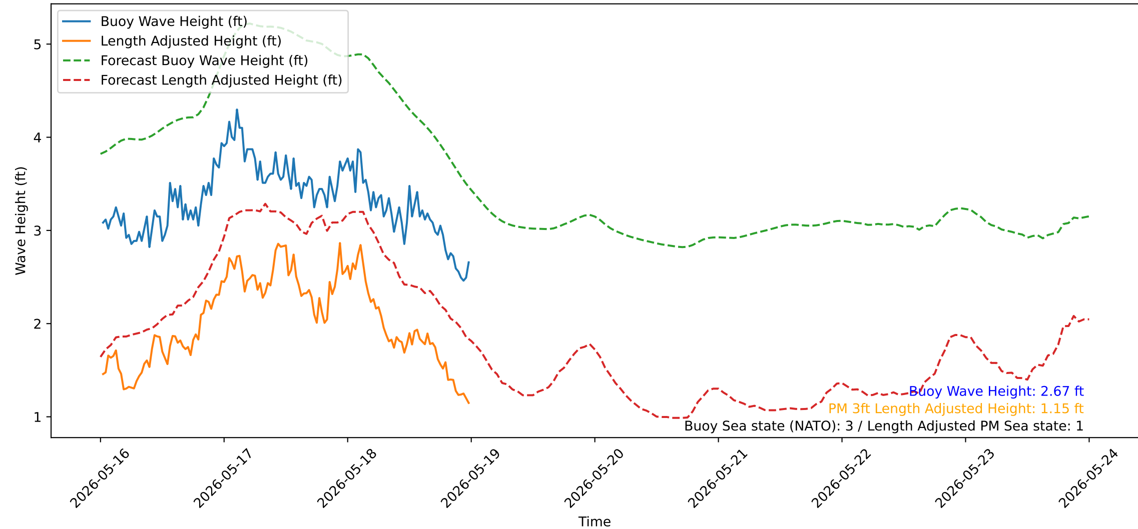
Wave Heights over Time for Oceanside Harbor at 2026-05-19 00:20:31
