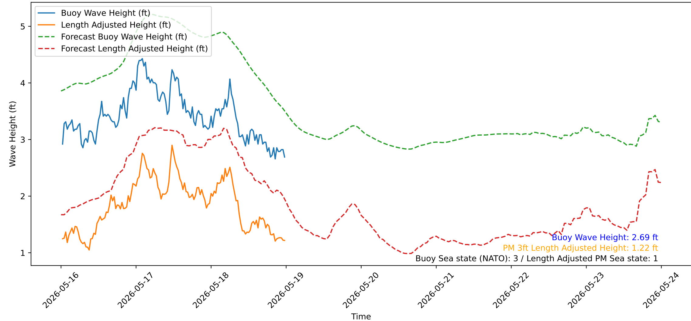
Wave Heights over Time for Green Beach at 2026-05-19 00:21:16
