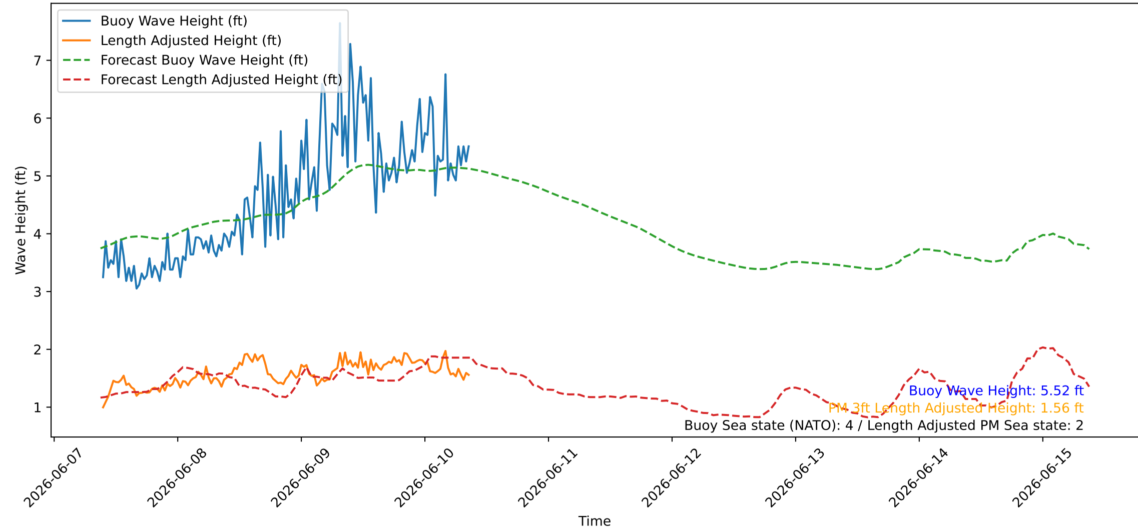
Wave Heights over Time for Red Beach at 2026-06-10 09:20:47
