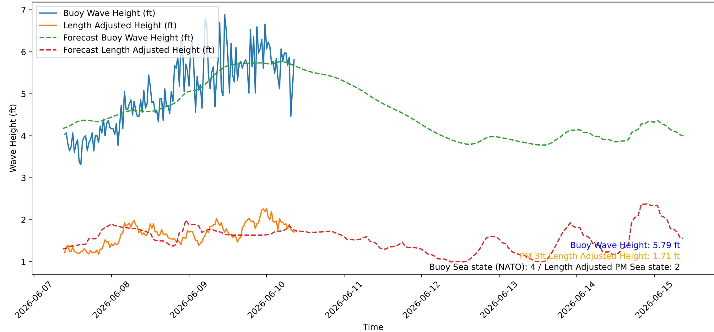
Wave Heights over Time for Green Beach at 2026-06-10 09:21:10
